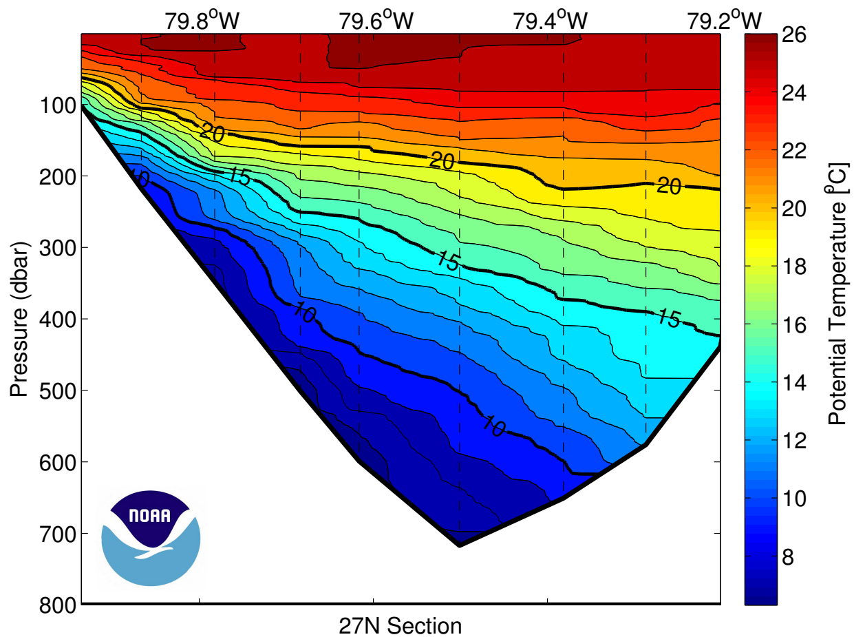
Figure 35: Potential Temperature ( ^{\circ}\text{C} ) section for the Florida Current North section. Contour intervals are 1^{\circ}\text{C} . Dashed vertical lines are the CTD station locations.
