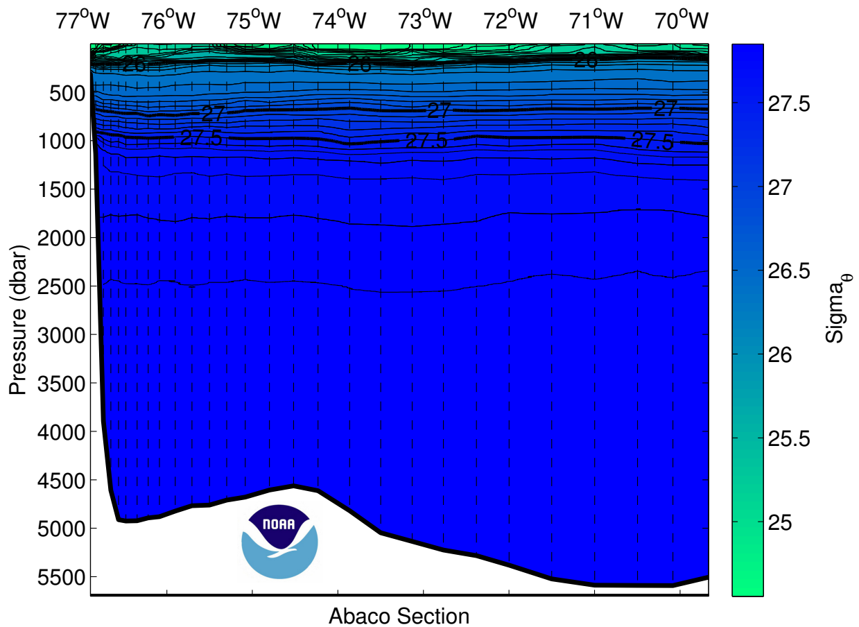
Figure 34: Potential density ( \text{kg/m}^3 ) section for the Abaco Section. Contour intervals are 0.1 \text{kg/m}^3 for density values greater than 27.5 \text{kg/m}^3 and 0.05 \text{kg/m}^3 below 27.5 \text{kg/m}^3 . Dashed vertical lines are the CTD station locations.
