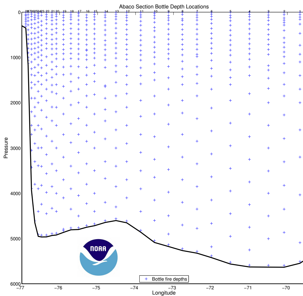
Figure 3: Bottle locations for 26.5°N Deep Western Boundary Current section east of Abaco Island.
