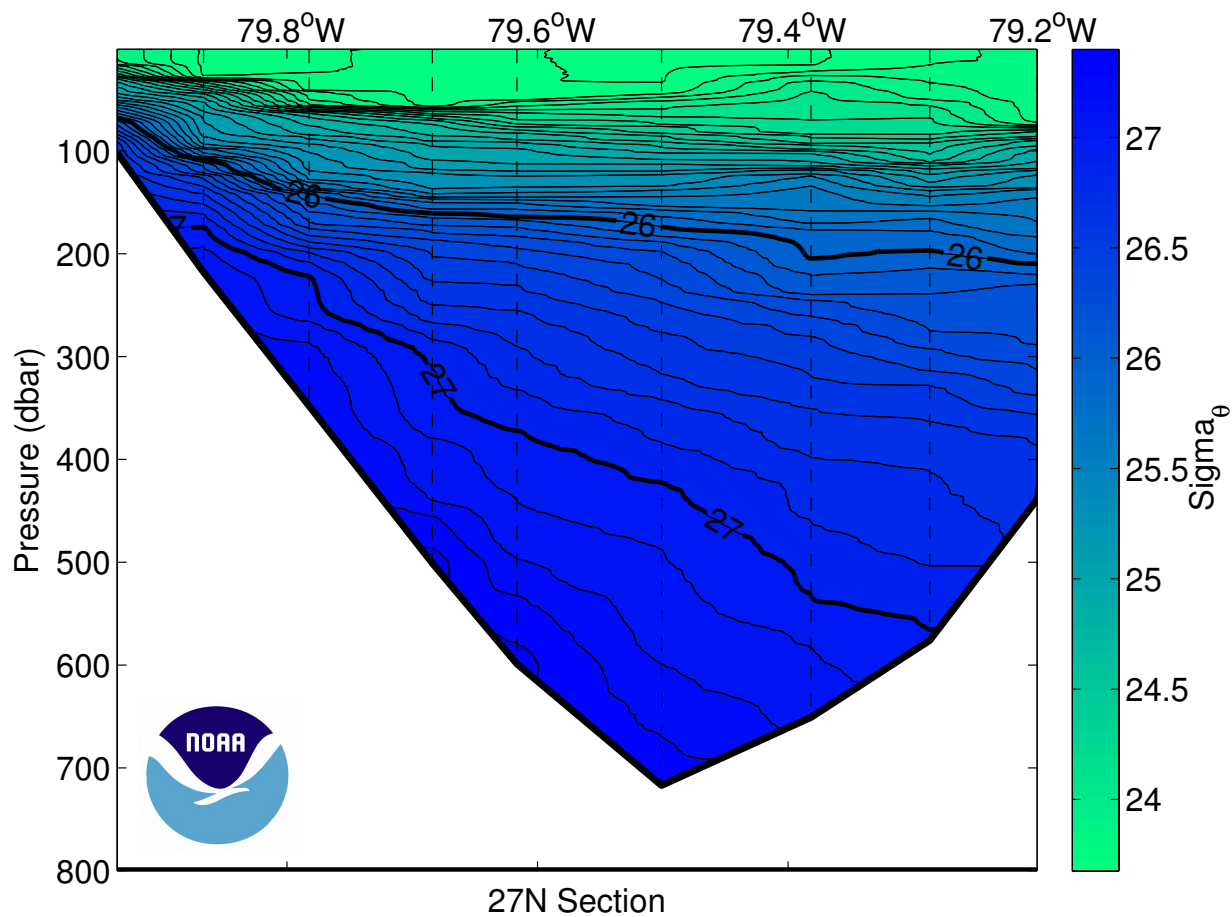
Figure 38: Potential density ( \text{kg/m}^3 ) section for the Florida Current North section. Contour intervals are 0.1 \text{ kg/m}^3 . Dashed vertical lines are the CTD station locations.
