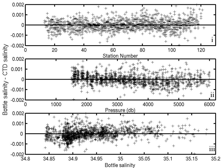
Figure 9.1b: Bottle – CTD salinity versus i. station number, ii. pressure and iii. bottle salinity for pressure > 1500db. Selection limits are |S_{\text{bot}} - S_{\text{CTD}}| < 0.002 (refer to Table 9.5 for statistics of bottles rejected).
