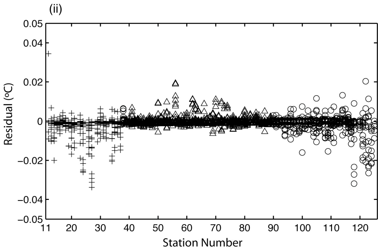
Figure 10.1: SBE35 – CTD temperature residual after application of limit 1(\pm 0.05^{\circ}\text{C}, \pm 2\sigma, \pm 2\sigma) . (i) Primary CTD temperature sensors (Groups A – C). (ii) Secondary CTD temperature sensors (Groups D – F). Station groups are (+) A or D, ( \Delta ) B or E and (o) C or F.
