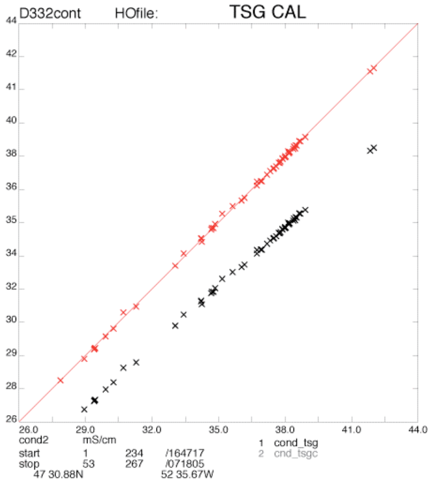
Figure 9.6 Scatter plot of CTD primary conductivity against TSG conductivity as measured (black) and following calibration (red). The red line indicates a 1:1 relationship.
