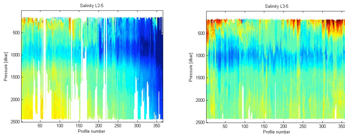
Figure 2.1: One year of vertical salinity profiles for the moorings Loco 2-5 (left) and Loco 3-5 (right). The colour scale ranges from 34.75 psu (dark blue) to 35.1 psu (dark red).
