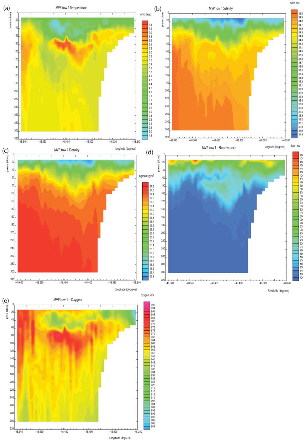
Figure 5.2: Contour plots of temperature (a), salinity (b), density (c), fluorescence (d) and oxygen (e) for the MVP tow across the Greenland shelf towards the Labrador Basin. Salinity has had the initial calibration described in the text applied. Fluorescence and oxygen remain, however, in raw instrument units.
