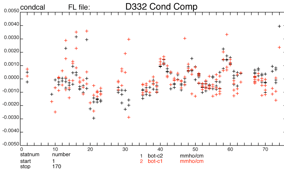
Figure 3.1: CTD primary (black, cond2) and secondary (red, cond) post-calibration conductivity differences (bottle minus CTD).
