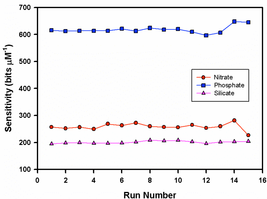
Figure 8.4: Instrument sensitivity of nitrate, phosphate, and silicate over the course of the cruise.
