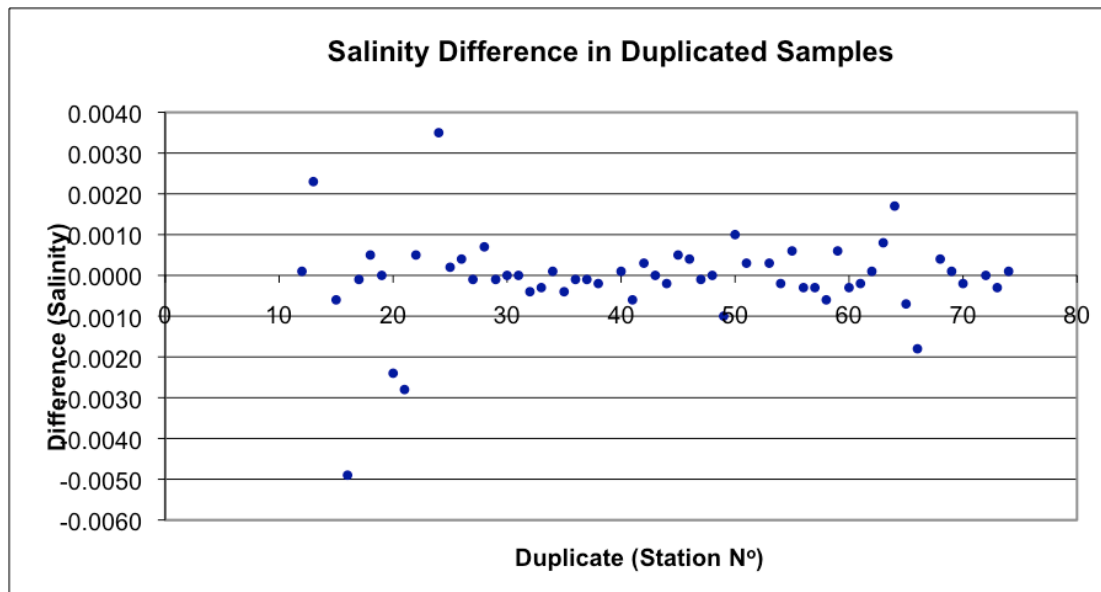
Figure 8.7.1: Plot of the differences between salinity measurements of duplicate samples.
