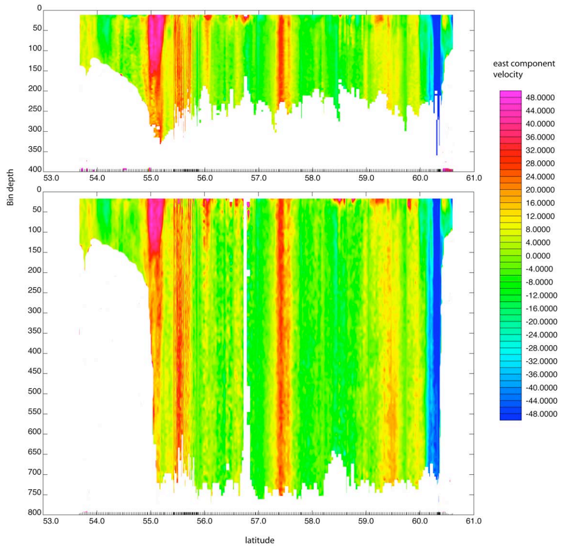
Figure 7.1: East component velocity for the 150 kHz VM-ADCP (top) and the 75 kHz VM-ADCP bottom, across the Labrador sea (section AR7W).
