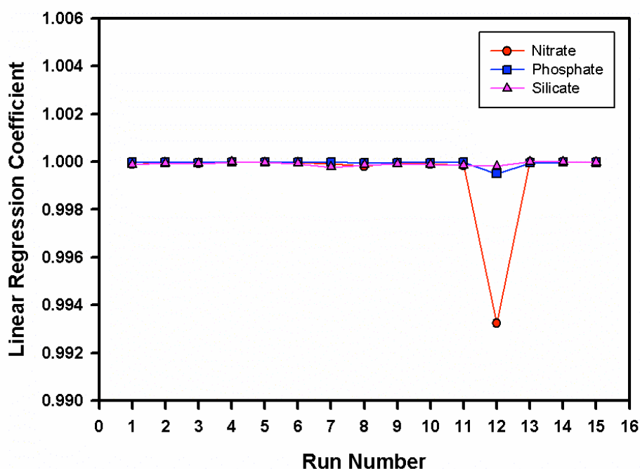
Figure 8.1: Linear regression coefficients for the standard calibrations for the inorganic nutrients nitrate, phosphate, and silicate.
