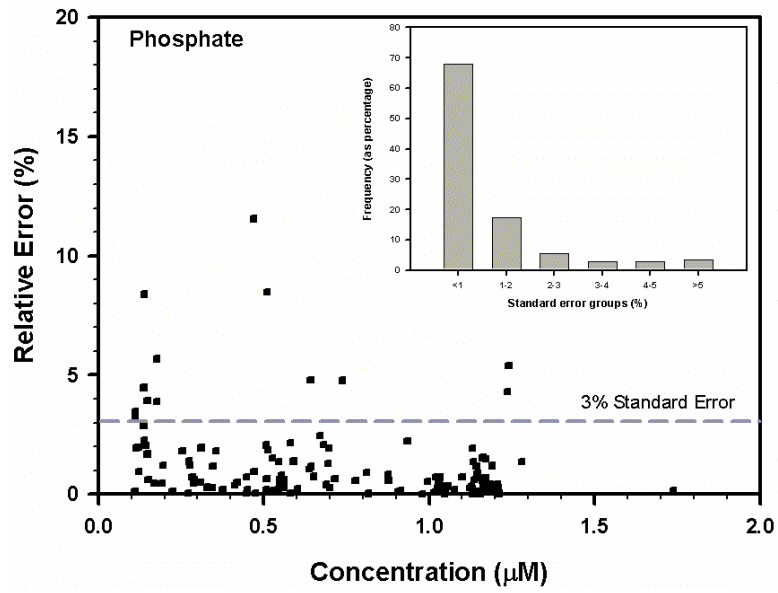
Figure 8.8: Shows sample precision for phosphate as a function of sample concentration. The inlay shows, as a percentage, the distribution of data over the discrete precision intervals <1, 1-2, 2-3, 3-4, 4-5, and >5%.
