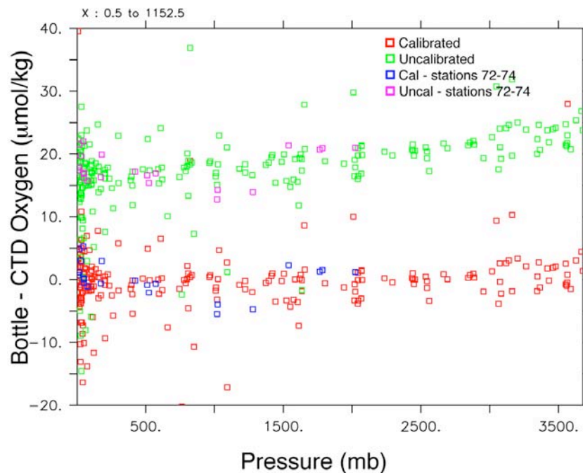
Figure 3.3: Bottle - sensor oxygen differences ( \mu\text{mol/kg} ) as a function of pressure. Green points are uncalibrated data for stations 1-70, pink for stations 72-74. Red shows the differences after application of the calibration for stations 1-70, blue shows differences for stations 72-74.
