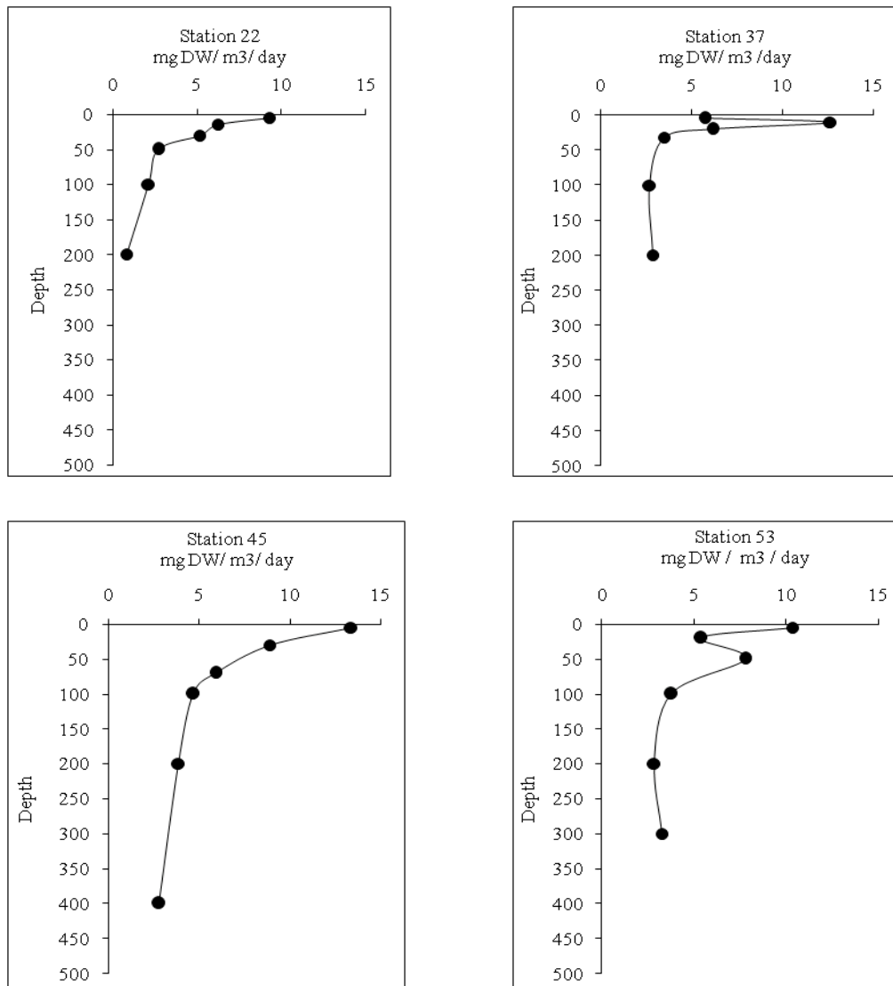
Figure 8.8.1: Examples of the production profiles as measured at selected stations.
