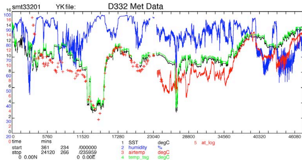
Figure 9.5 Full cruise time series of SST, humidity, air temperature (airtemp) and TSG temperature (temp_tsg).
