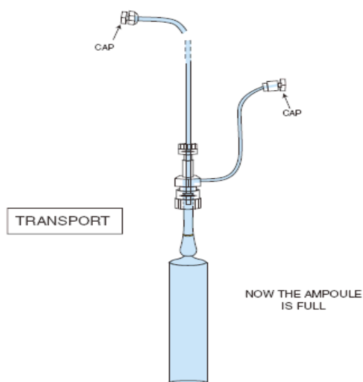
Figure 8.3.1: Schematic of the glass ampoule and tee during sampling.
