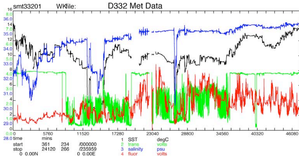
Figure 9.4 Full cruise time series of SST, transmissivity, salinity and fluorescence.
