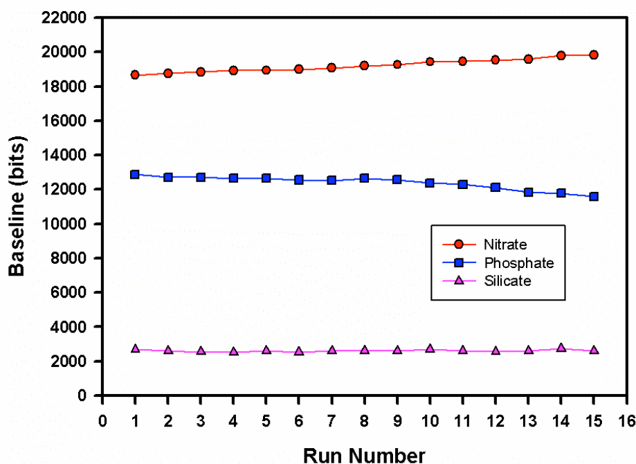
Figure 8.3: Baseline values for the three inorganic nutrients nitrate, phosphate and silicate.
