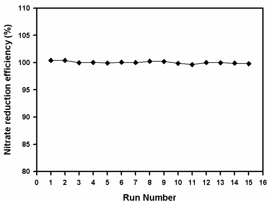
Figure 8.2: Shows the quantitative reduction efficiency of nitrate to nitrite by the cadmium column as a function of time.
