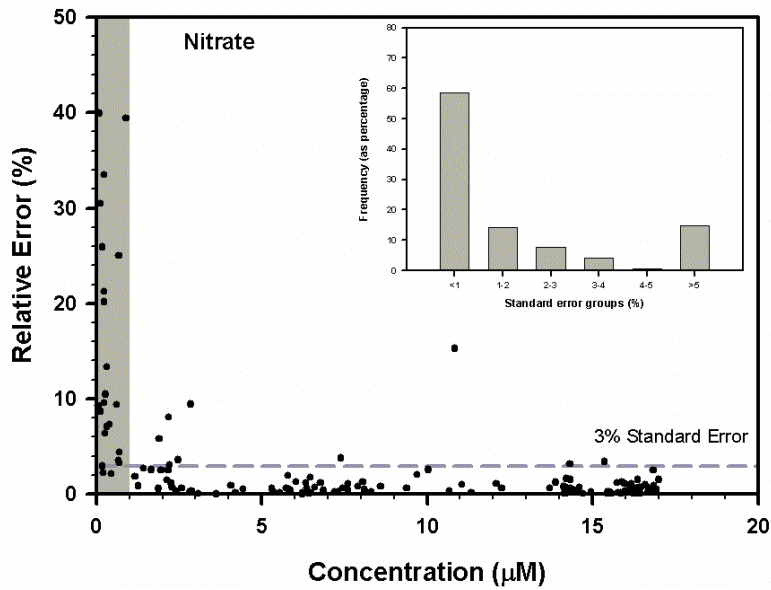
Figure 8.6: Shows sample precision for nitrate as a function of sample concentration. Grey shaded area marks the region where the sample concentration is less than 1\mu\text{M} . The inlay shows, as a percentage, the distribution of data over the discrete precision intervals <1, 1-2, 2-3, 3-4, 4-5, and >5%.
