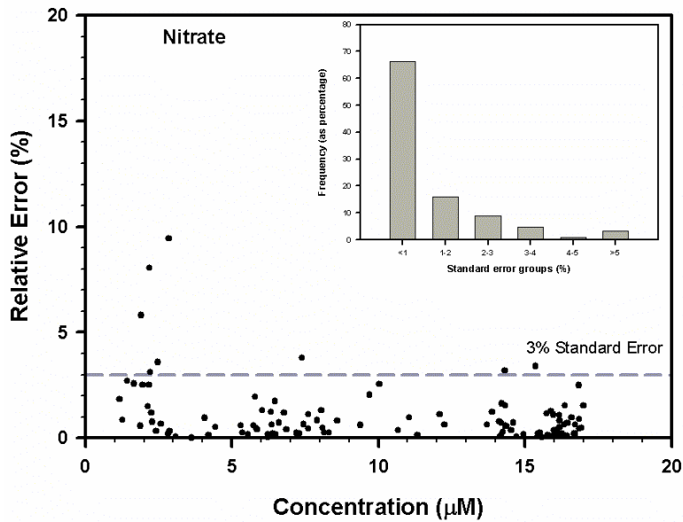
Figure 8.7: Shows sample precision for nitrate as a function of sample concentration with <1\mu\text{M} data removed. The inlay shows, as a percentage, the distribution of data over the discrete precision intervals <1, 1-2, 2-3, 3-4, 4-5, and >5% excluding the <1\mu\text{M} data.
