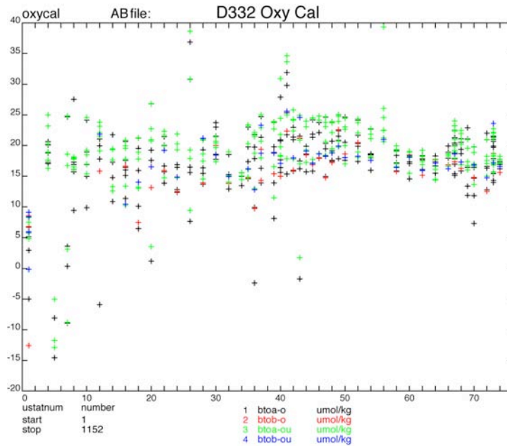
Figure 3.2: Bottle - sensor oxygen differences ( \mu\text{mol/kg} ) as a function of D332 station number. Black & red: downcast sensor values interpolated to upcast using pbotle; Green and blue: upcast sensor values. Black and green are for the main bottle oxygens, red and blue are the duplicates. Note the change of sensor after failure on station 71.
