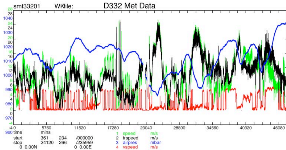
Figure 9.2 Full cruise time series of relative wind speed (speed), true wind speed (trspeer), atmospheric pressure (airpres) and ship speed (vspeed).
