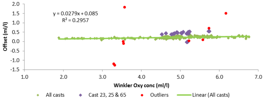
Fig. 4: Oxygen concentration offsets against Winkler titration measurements from discrete samples.
