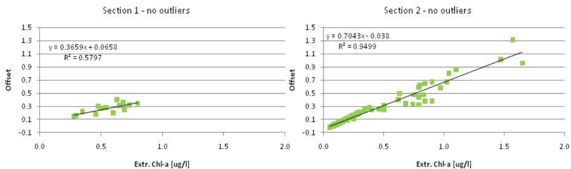
Fig. 10: Fluorescence offsets against extr chl-a measurements on discrete underway samples split between 30/09/2011 08:00 to 03/10/2011 13:04 (section 1) and 03/10/2011 13:04 to 09/11/2011 14 (section2).
