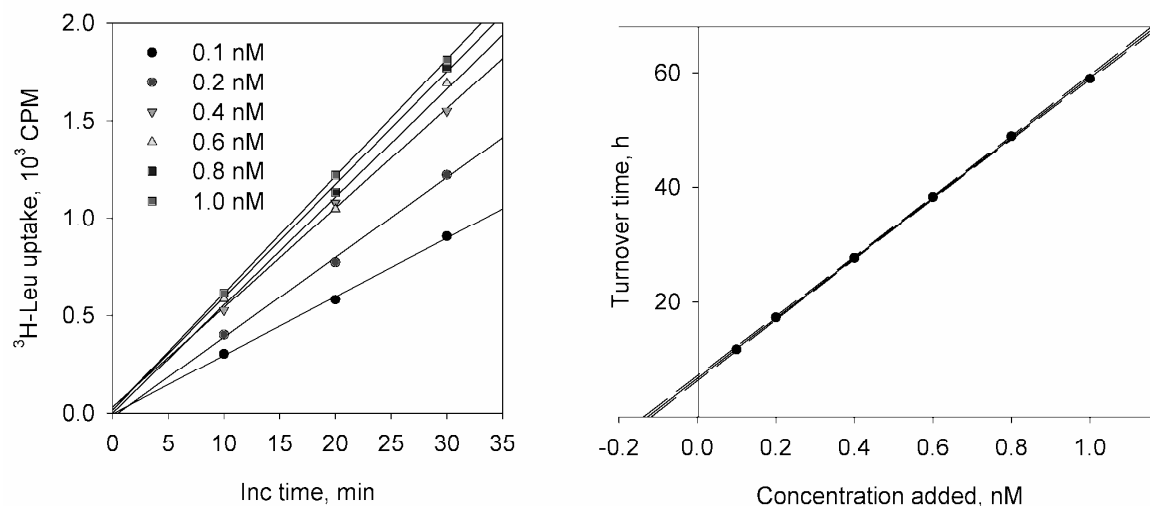
Figure 1: Example of data from a 3 H-Leucine bioassay.
