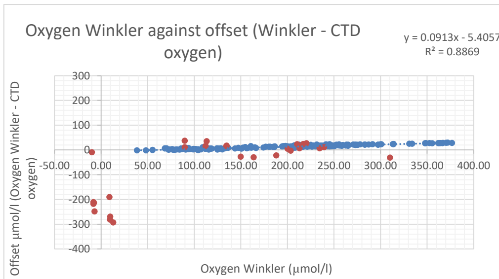
Fig. 6: Oxygen concentration offsets against Winkler titration measurements from discrete samples. Outliers removed from calibration dataset are shown.
