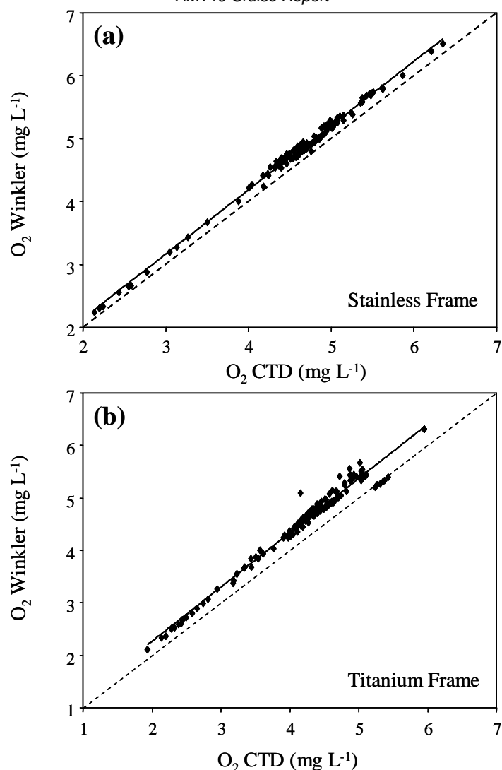
Figure 1: Calibration of O 2 sensors on the Conductivity Temperature Depth profilers during AMT 19 (JC_039). O 2 determined by Winkler titration against sensor data. (a) Stainless Steel Frame, (b) Titanium Frame. The 1:1 line is shown in each case.
