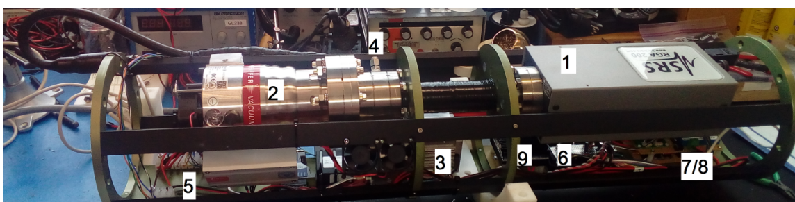
Figure 18.2: Design of on board MIMS 1.Mass spec, 2.Turbo pup, 3.Rafting pump, 4.Membrane inlet connector, 5.Terminal strip for all connection communications, 6.Arduino – communicates to control board-communicates through the housing to the user, 7.Electronic controls / analog sensor output / power control board, 8.Voltage changer to 24 V and gives it to the mass spec, 9.Power management, change voltage 24-12 V or what's coming to 24 V.
