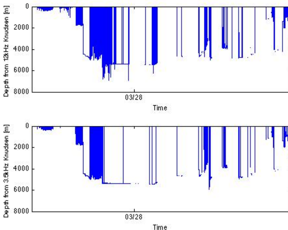
Figure 7: Time series of the two Knudsen echosounders on board the vessel. The high frequency 12kHz data is in the upper panel, the 3.5 kHz low frequency data is in the lower panel. The data was of poor quality during rough weather, so generally the echosounders were only turned on during mooring and CTD work.
