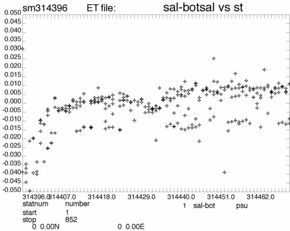
Figure 5a. Bottle – CTD salinity residuals plotted as a function of station number.
