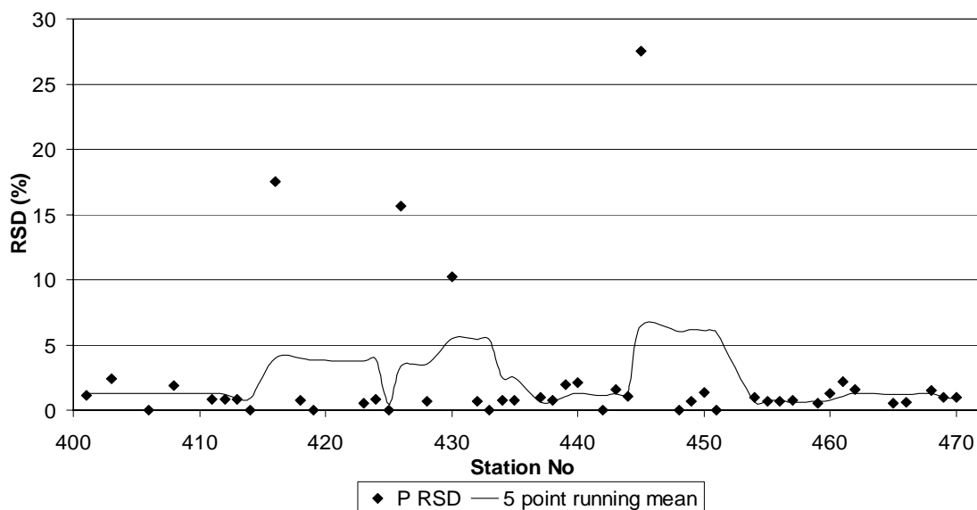
Figure 11c. Time series of phosphate RSD variation.
