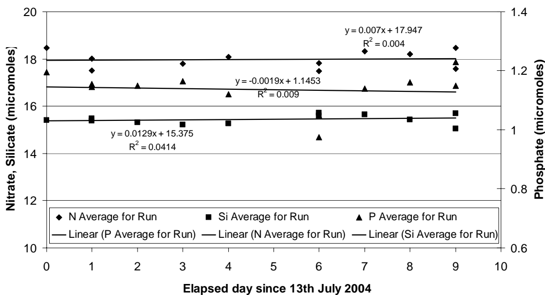
Figures 12. Time series of bulk nutrient concentrations.
