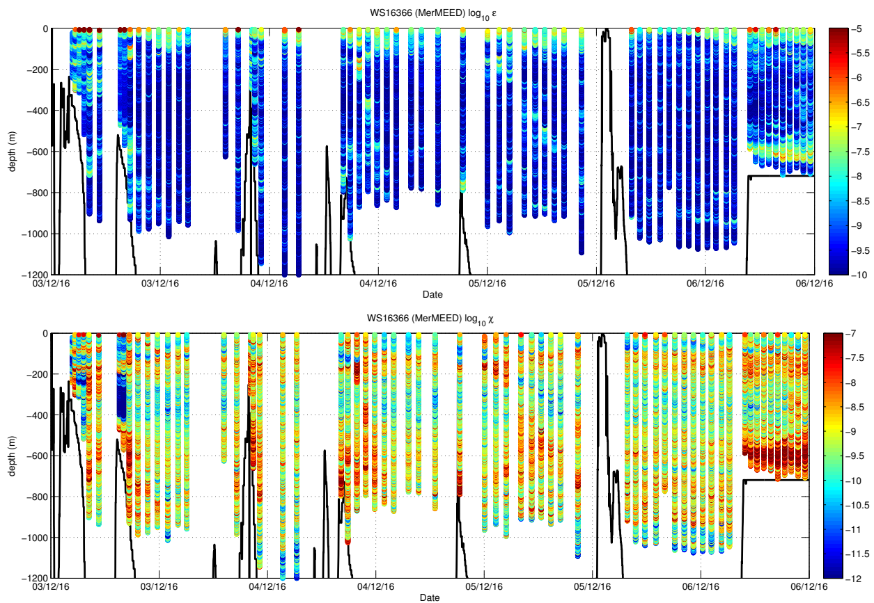
Figure 3: Profiles of turbulent dissipation ( \epsilon , top panel) and temperature variance ( \chi , bottom panel) collected during cruise WS16336.
