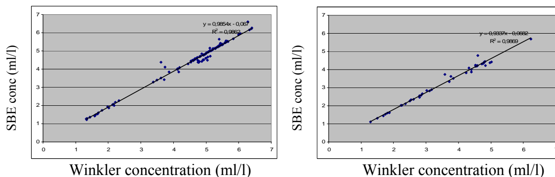
Figure 1. Dissolved oxygen calibration curves for the Seabird CTD sensor versus onboard determined Winkler titrations
