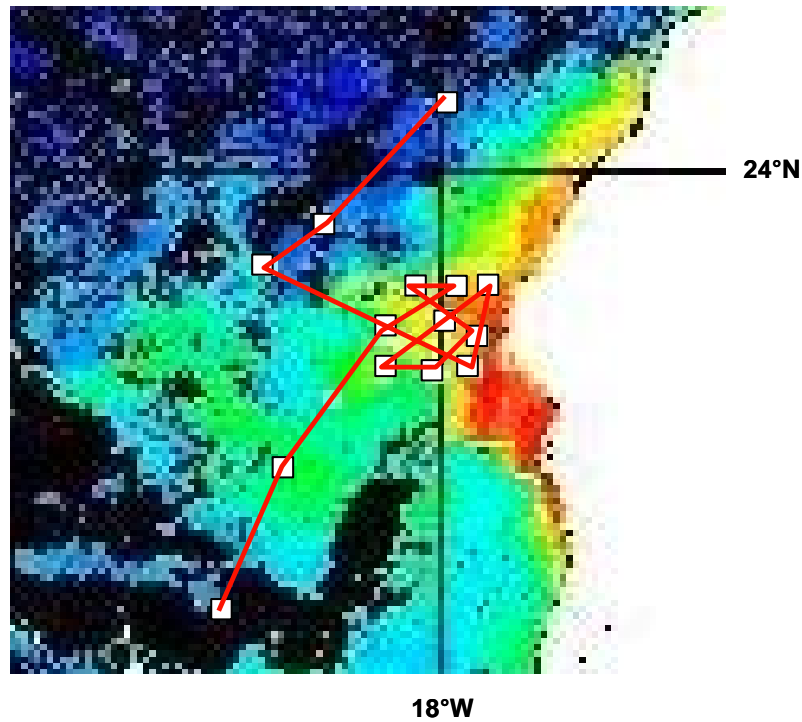
Figure 3. Cruise track during survey of the North West African Upwelling overlaid onto SeaWiFS chlorophyll image for 04.10.2004
