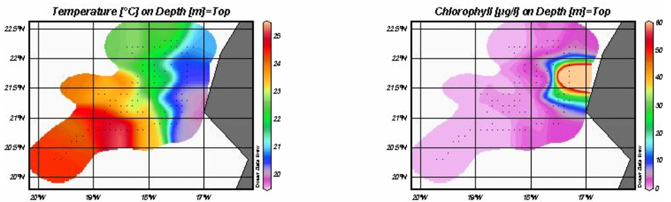
Figure 4. Surface contours (30 minute resolution) of temperature and chlorophyll for North West African Upwelling
