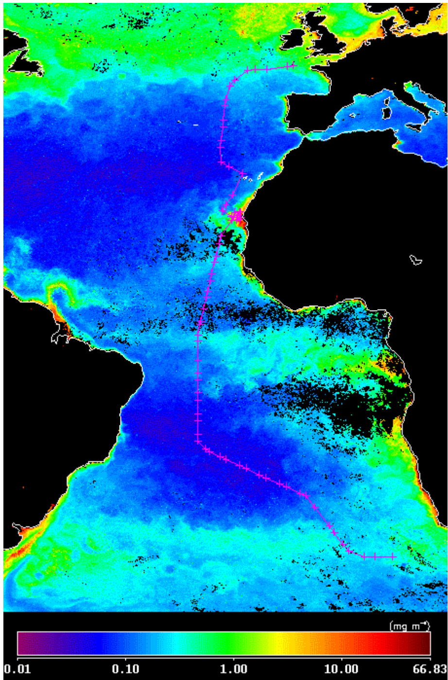
Figure 1. Cruise track overlaid on SeaWiFS chlorophyll composite for September 2004
