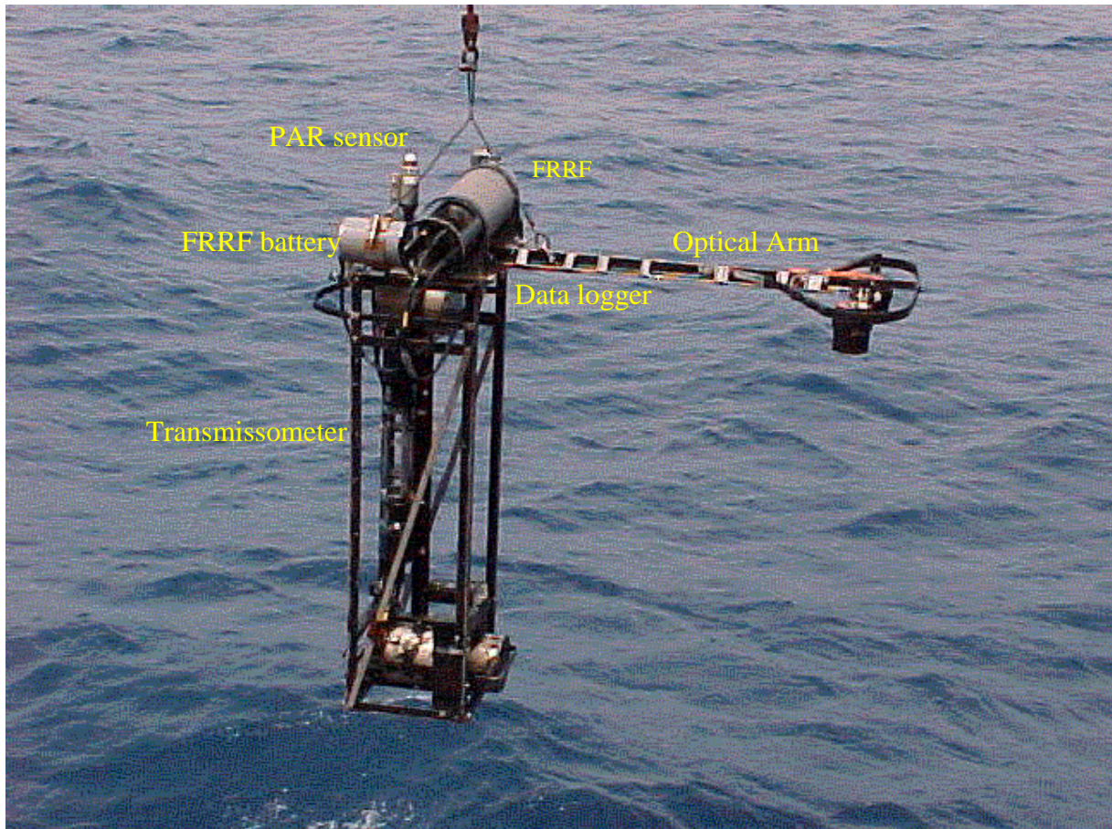
Figure 1. Arrangement of the optical rig employed for AMT 11
