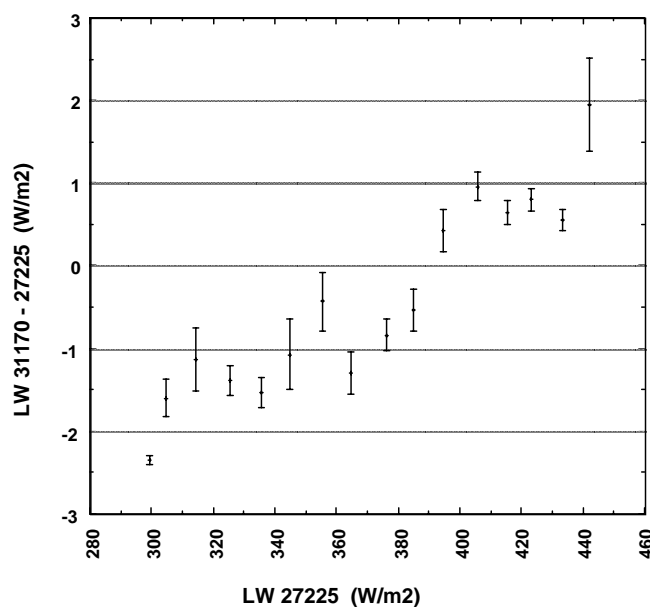
Figure 8. The difference in longwave radiation from the two pyrgeometers. The error bars indicate the standard deviation of the mean.
