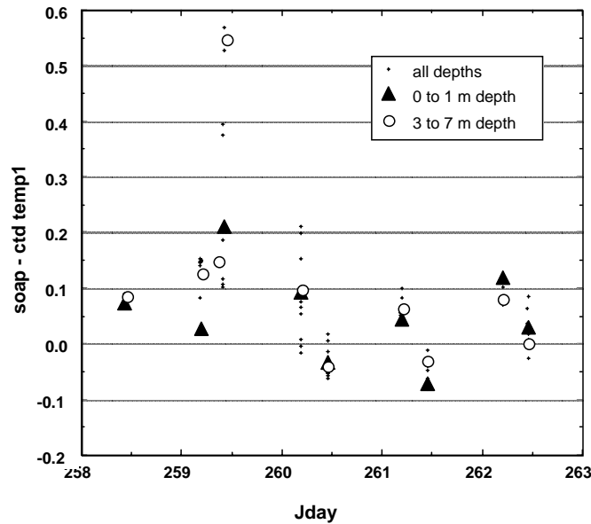
Figure 3. Soap - CTD temp1 SST differences for the first nine CTD casts.
