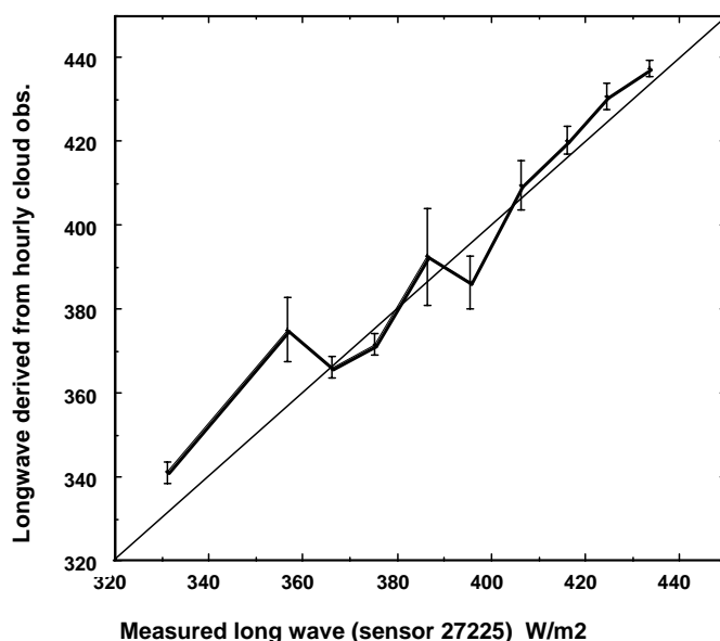
Figure 7. Comparison of longwave radiation derived from the hourly cloud observations against that measured by the Eppley instrument.
