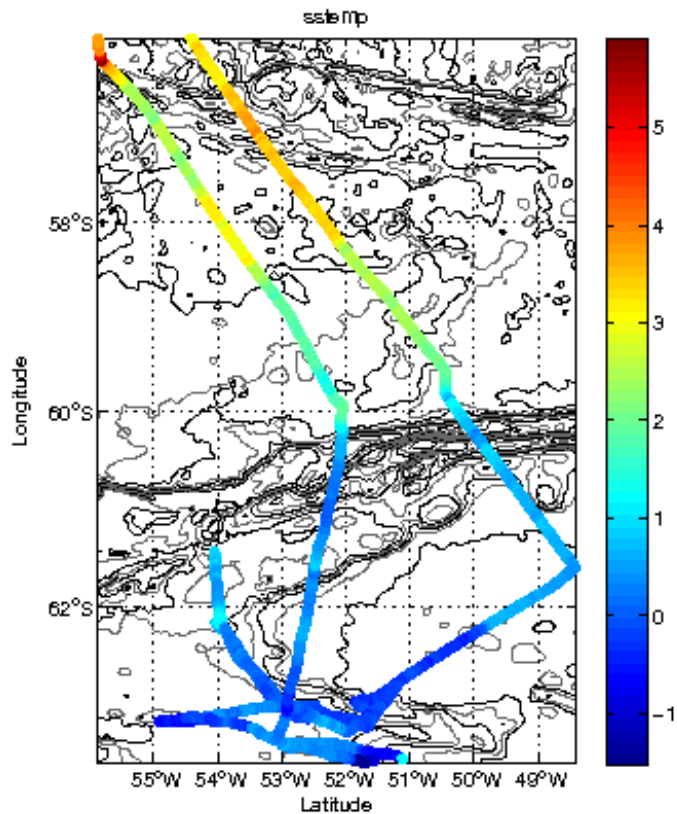
Figure 1 Cruise track with Sea Surface Temperature (SST) as from shipboard thermosalinograph.
