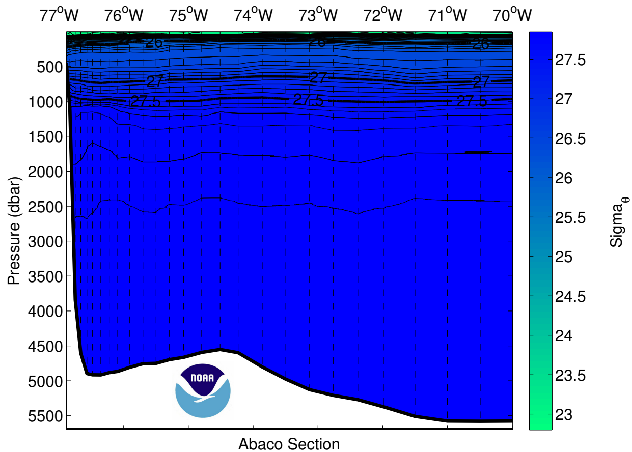
Figure 31: Potential density ( \text{kg/m}^3 ) section for the Abaco Section. Contour intervals are 0.1 \text{kg/m}^3 for density values greater than 27.5 \text{kg/m}^3 and 0.05 \text{kg/m}^3 below 27.5 \text{kg/m}^3 . Dashed vertical lines are the CTD station locations.
