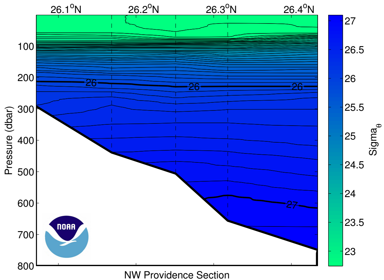
Figure 39: Potential density ( \text{kg/m}^3 ) section for the Northwest Providence Channel section. Contour intervals are 0.1 \text{ kg/m}^3 . Dashed vertical lines are the CTD station locations.
