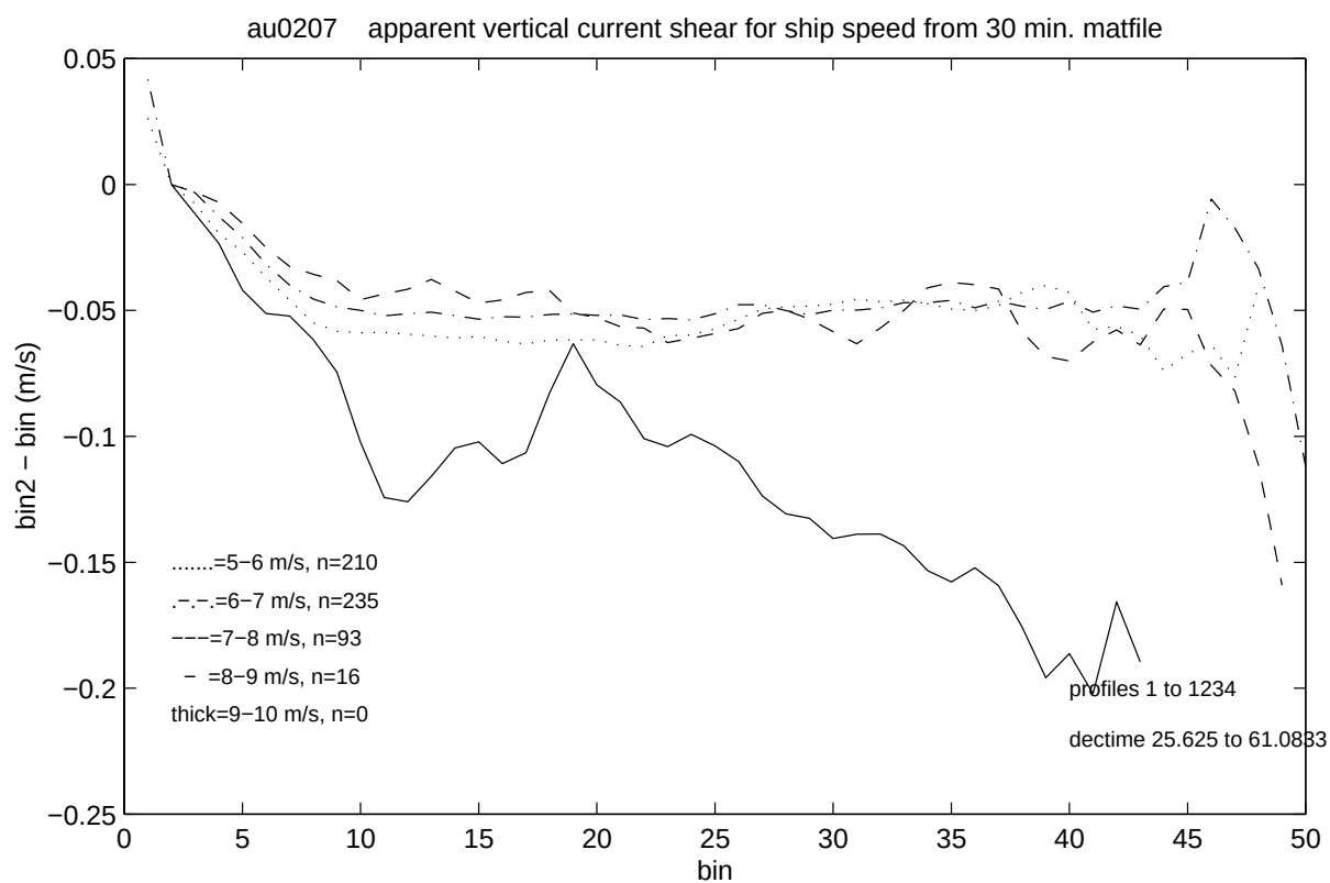
Figure 1.5b: Apparent vertical current shear calculated from uncorrected (i.e. ship speed included) ADCP velocities for cruise au0207.
