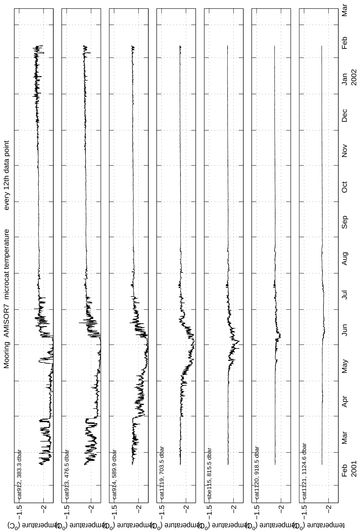
Figure 2.5m: Microcat and SBE39 temperature data for mooring AMISOR7.
