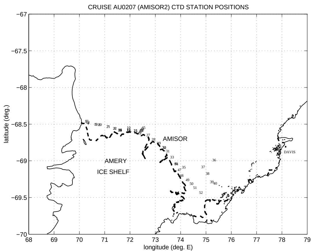
Figure 1.3: AU0207 cruise track and CTD station positions.
