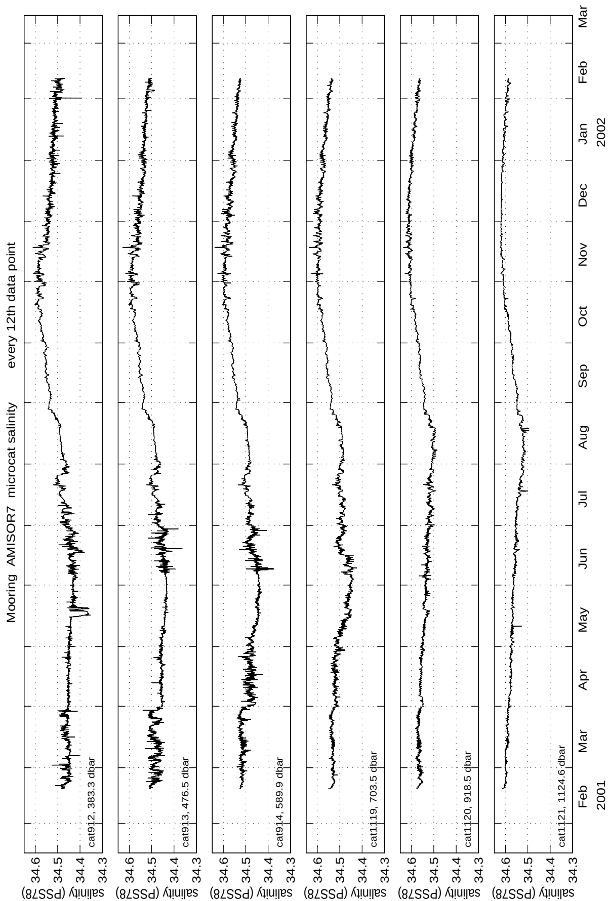
Figure 2.5n: Microcat salinity data for mooring AMISOR7.
