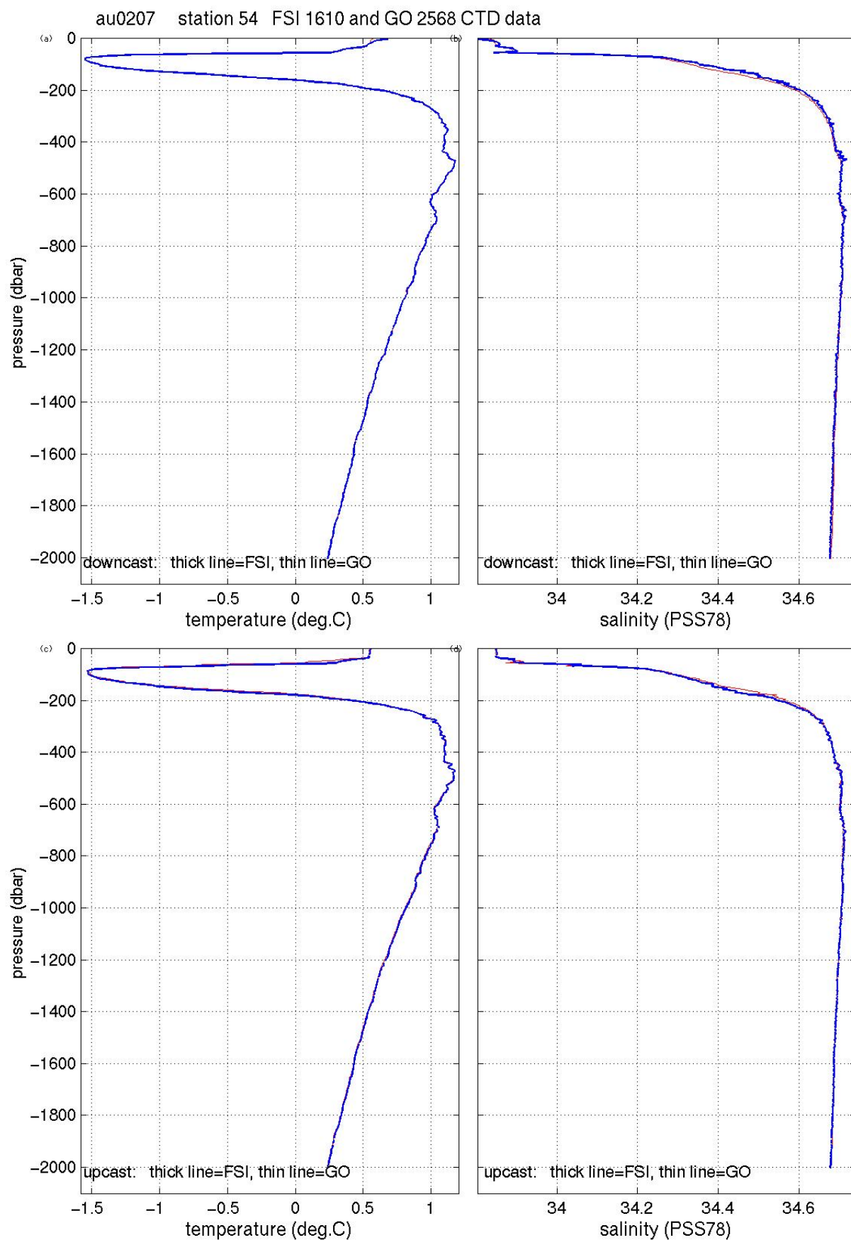
Figure A1.3.3: Comparison of FSI and GO CTD data, cruise au0207, station 54.
