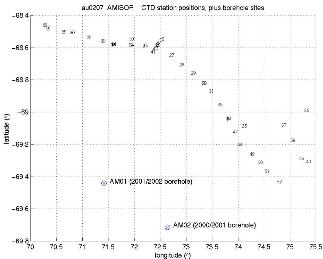
Figure A1.3.2: CTD station positions for cruise au0207, and Amery Ice Shelf boreholes AM01 and AM02 from 2001/2002 and 2000/2001 seasons respectively.
