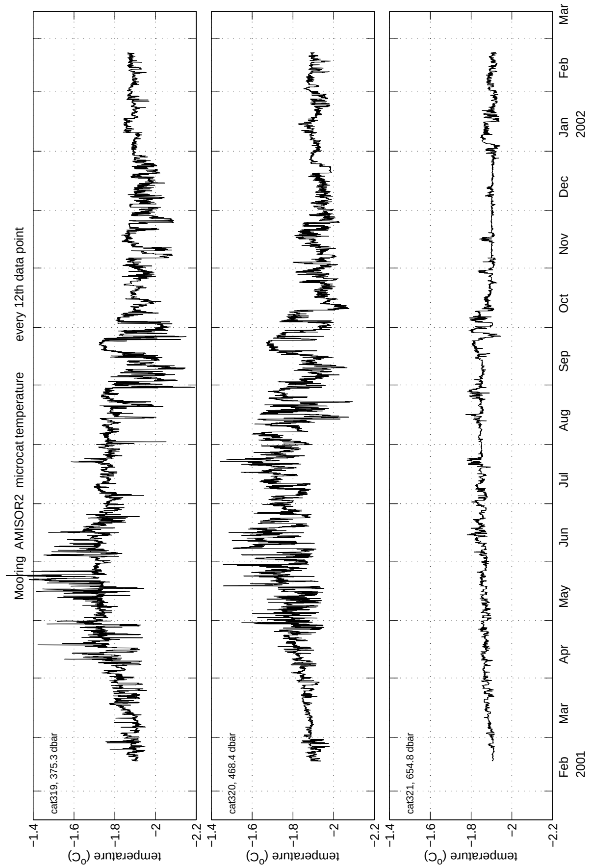
Figure 2.5c: Microcat temperature data for mooring AMISOR2.
