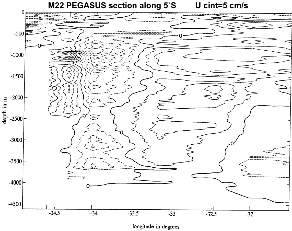
Fig. 20: Pegasus section of the meridional currents at 5°S. Contour interval is 5 cm/s. Northward contours are solid, southward dashed. The stations are indicated with the longer tick marks at the bottom of the plot.
