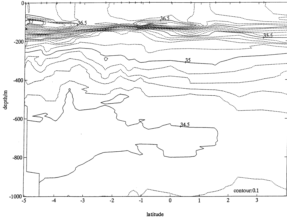
Fig. 13: Salinity distribution along 35°W between 5°01'S and 4°N from November 2 to 7, 1992 for the upper 1000m of the ocean with a contour interval of 0.1.
