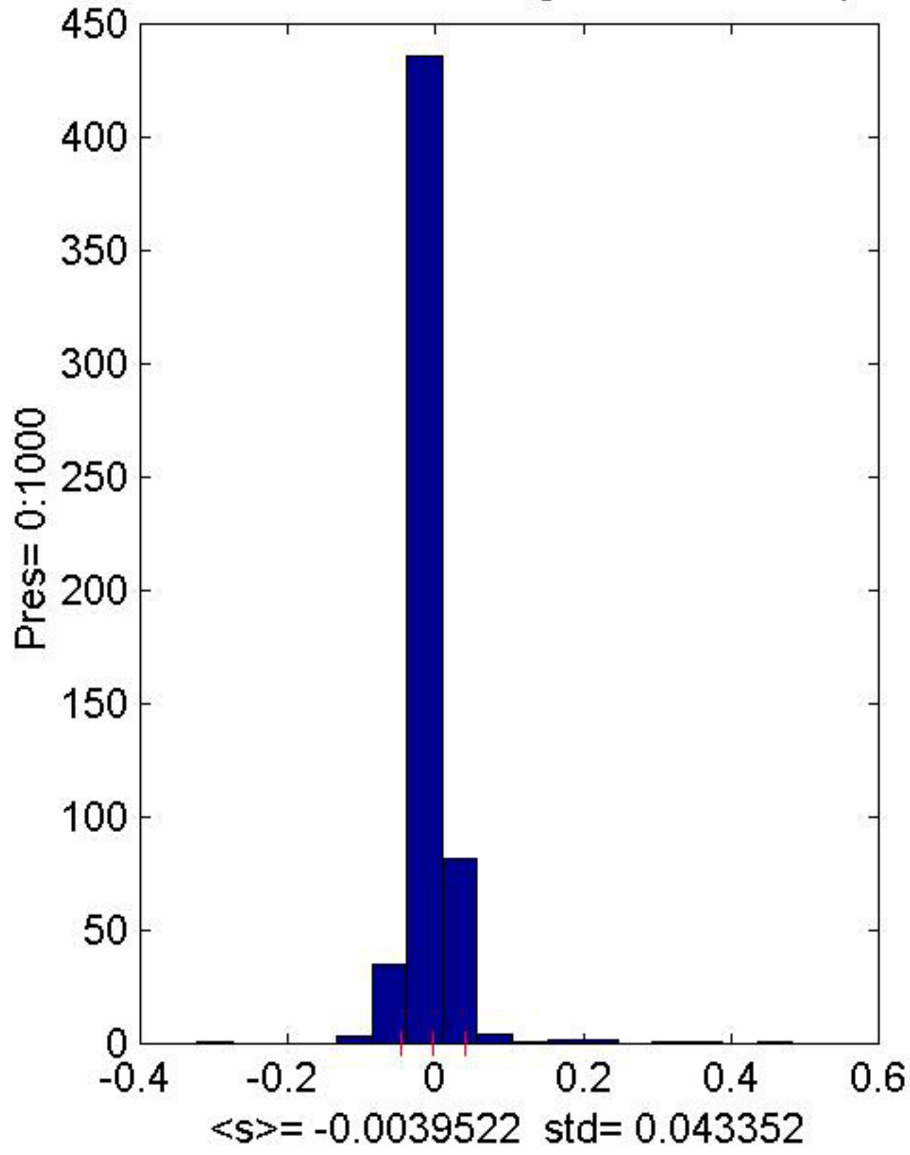
A10N: Down CTD - WS salt Histograms for select pres. intervals
