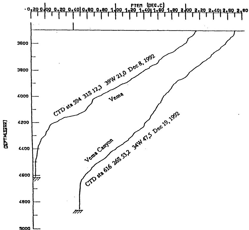
Fig. 27: Vertical profiles of potential temperature near the bottom at the Vema Sill and the northward extension of the Vema Channel, called Vema Canyon. The right curve is shifted by 0.6 K. Both stations were occupied during M 22/4 in December 1992. For locations see Figure 5.
