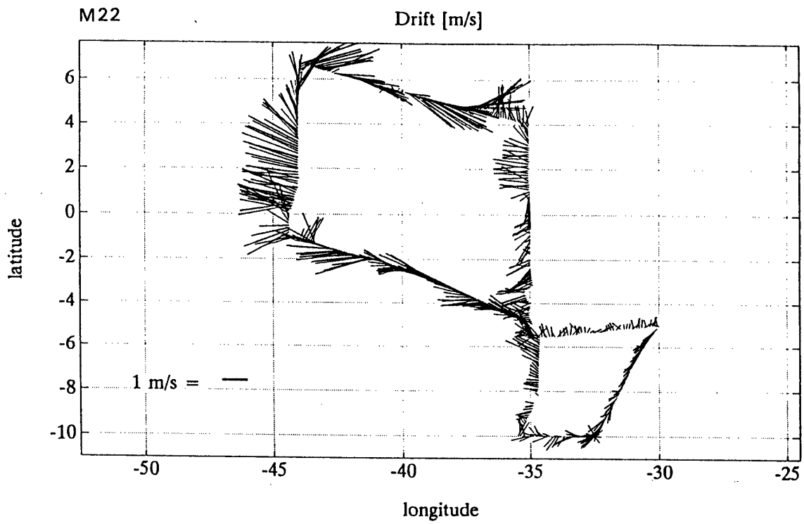
Fig. 24: DVS: ship's drift along cruise track
