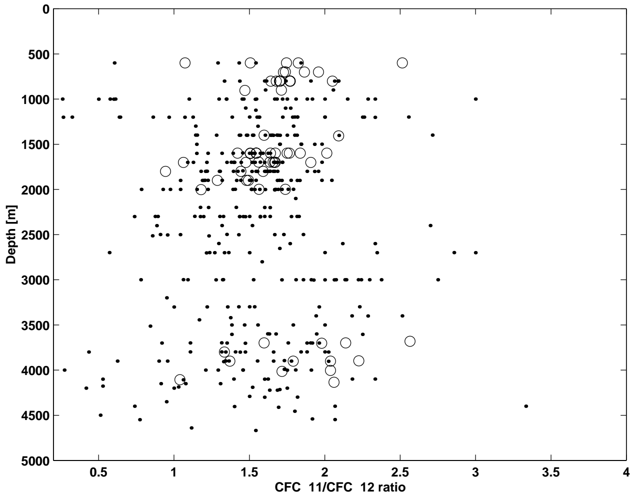
Figure 4: CFC-11/CFC-12 ratio versus depth; CFC-11 concentrations larger than 0.1 pmol/kg -1 are marked by circles.
