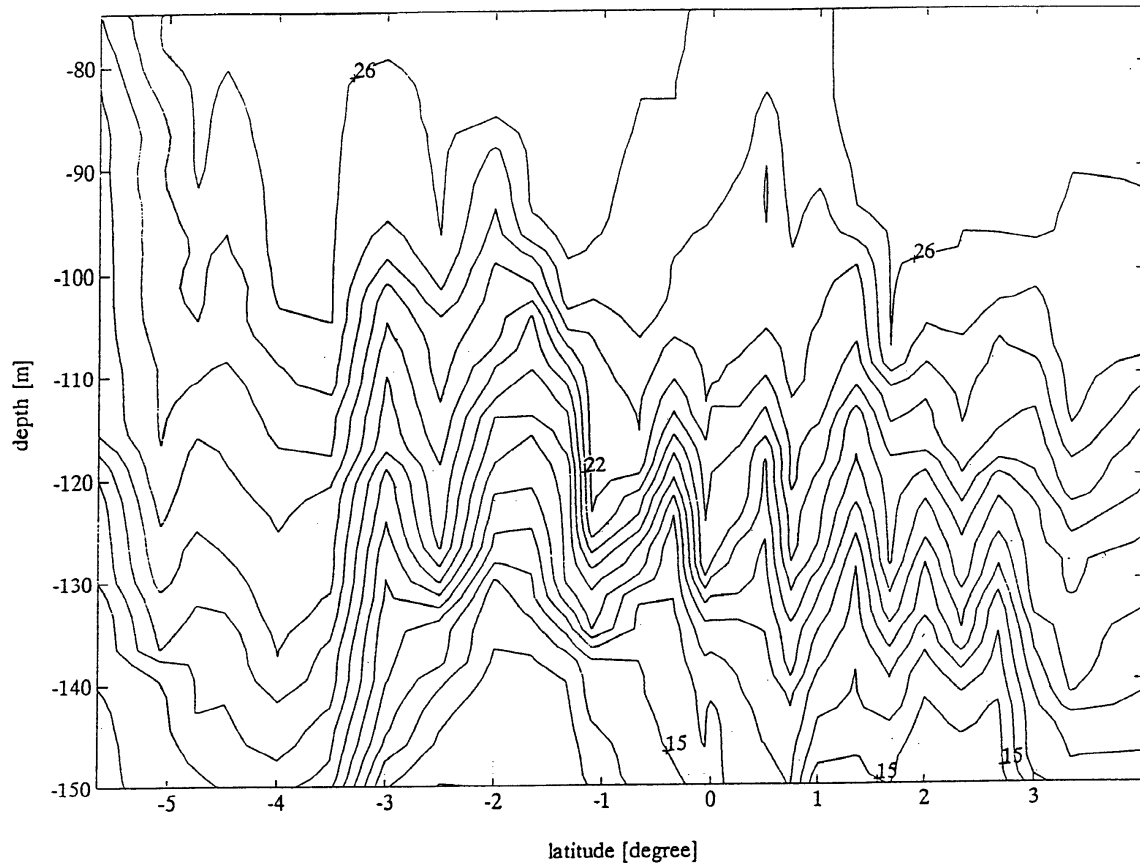
Fig. 18: Temperature distribution from XBT data for the 35°W section for the depth range of the thermocline between 75 and 150 m with an isotherm spacing of 1°C.
