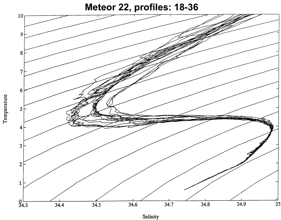
Fig. 14: TS-curves (potential temperature) of all CTD profiles of the 35°W section for the temperature range 0° to 10°C.
