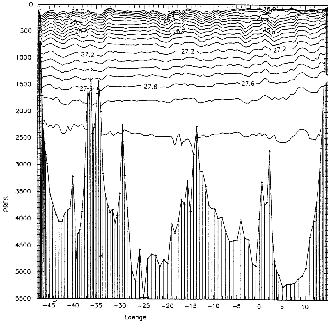
Fig. 32: Sigma-T along 30°S Contour interval: 0,1
