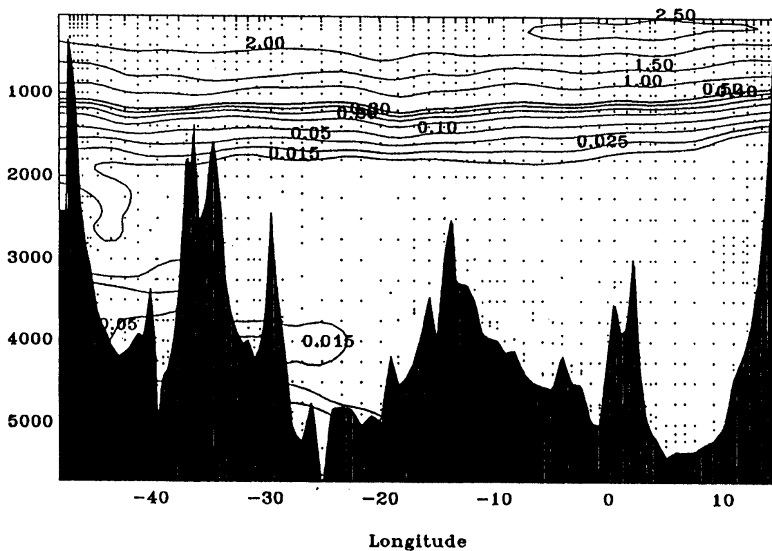
Fig. 35: F-11 section on 30°S
