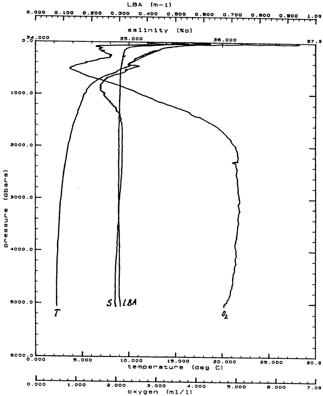
Fig. 12: Profiles of salinity, temperature, oxygen and light beam attenuation (LBA) at station 467-92, south of Cabo Verde Islands
