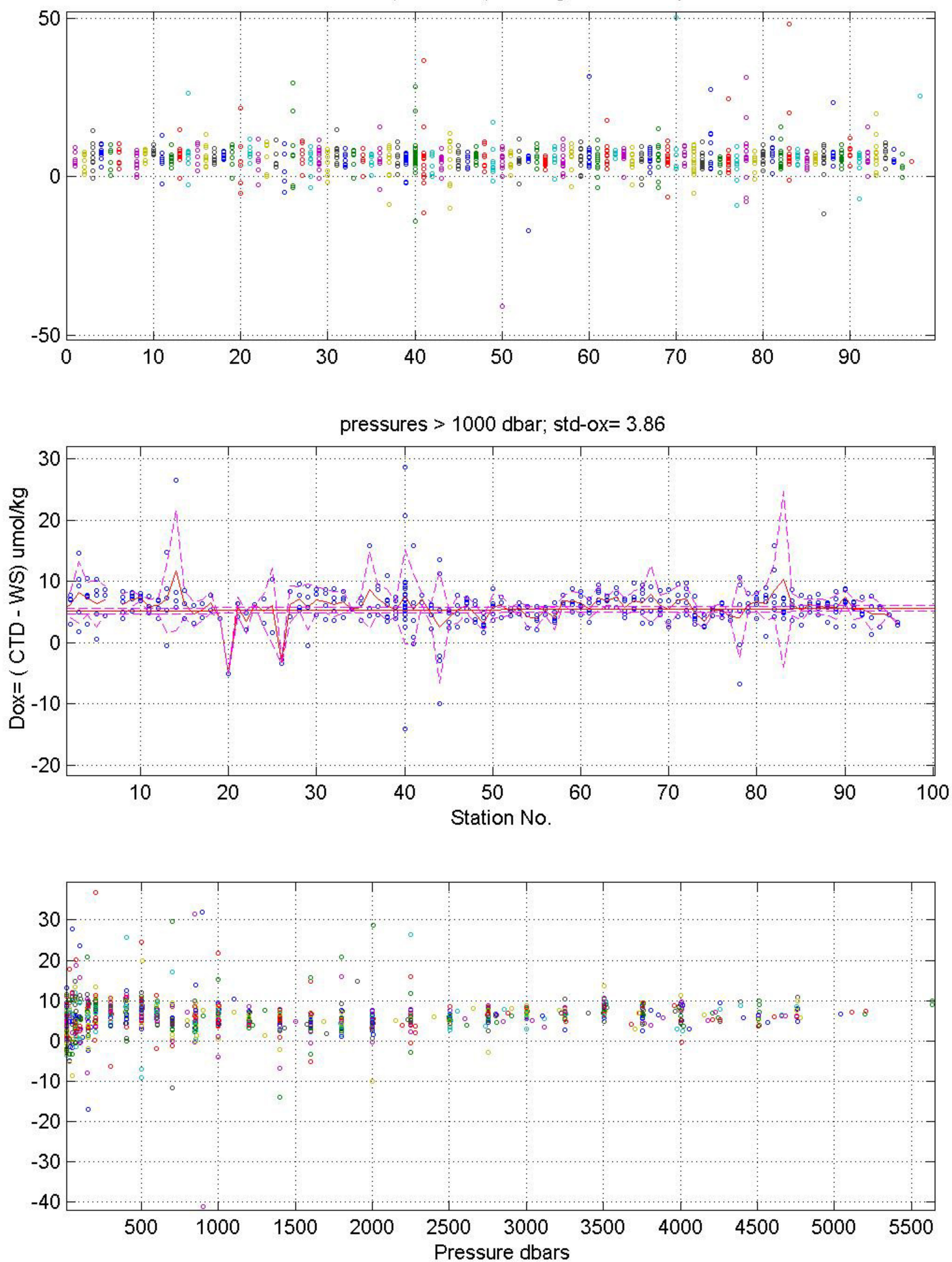
A10N: Dox (CTD -WS) umol/kg down all depths
