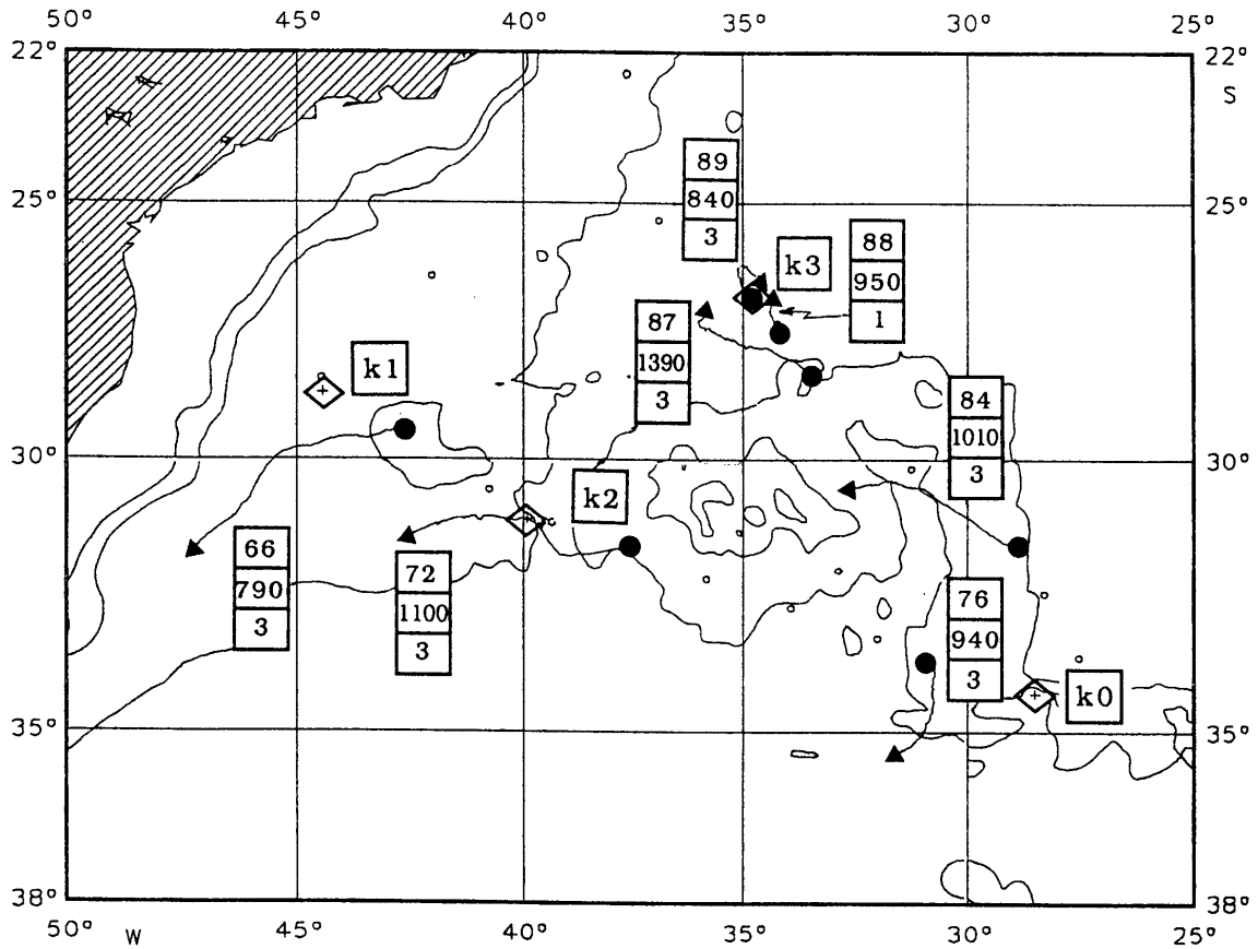
Fig. 29: Trajectories of selected RAFOS floats launched during M 22/4. Numbers indicate IfM serial number, mean depth (m), and mission length (month). Diamonds indicate sound source positions K1, K2, K3, and K0 (from west to east).
