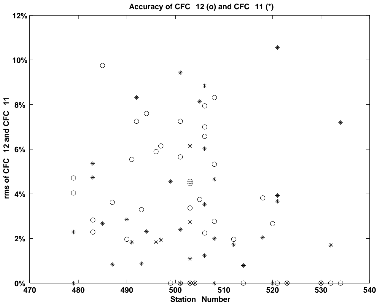
Figure 1: Accuracy of CFC-12 (o) and CFC-11 (*); replicate samples plotted vs profile number.
