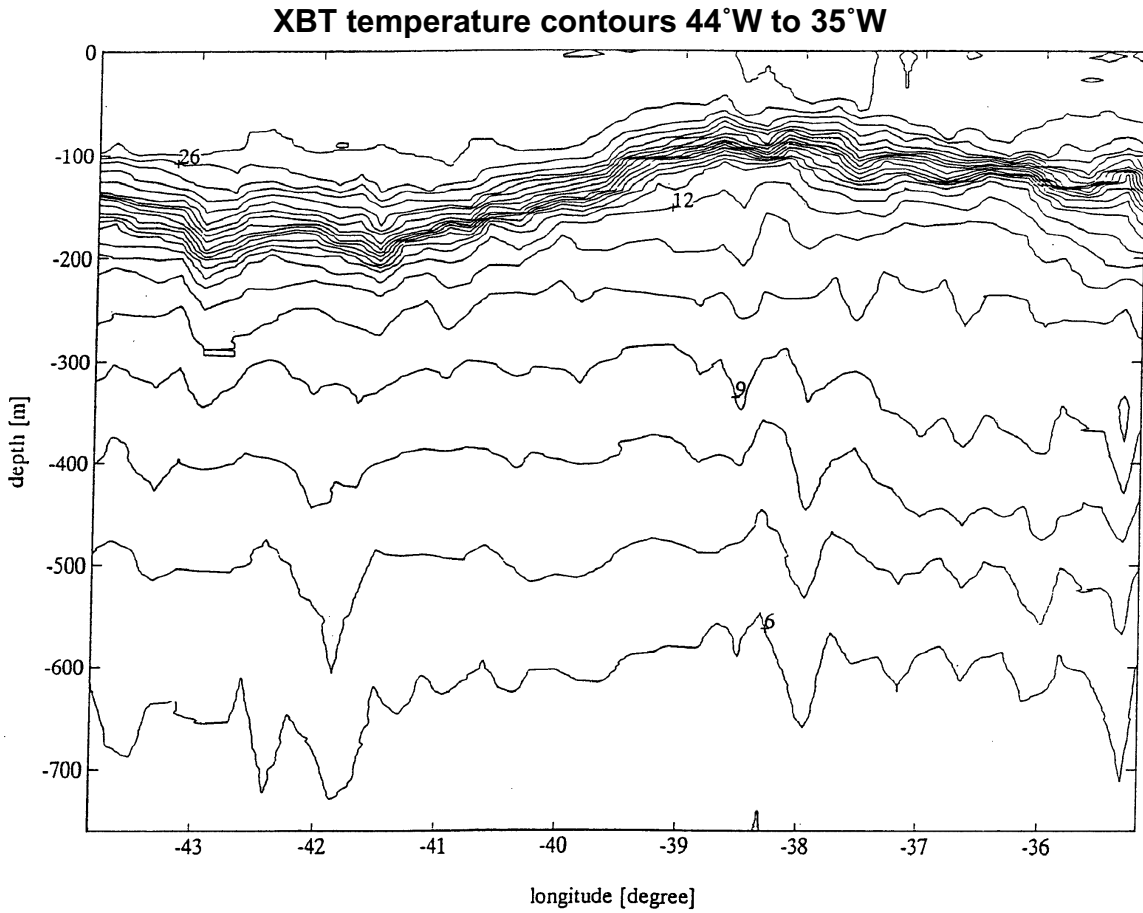
Fig. 19: Temperature distribution from XBT data between 6° 40'N, 44°W and 4°N, 35°W with an isotherm spacing of 1°C.
