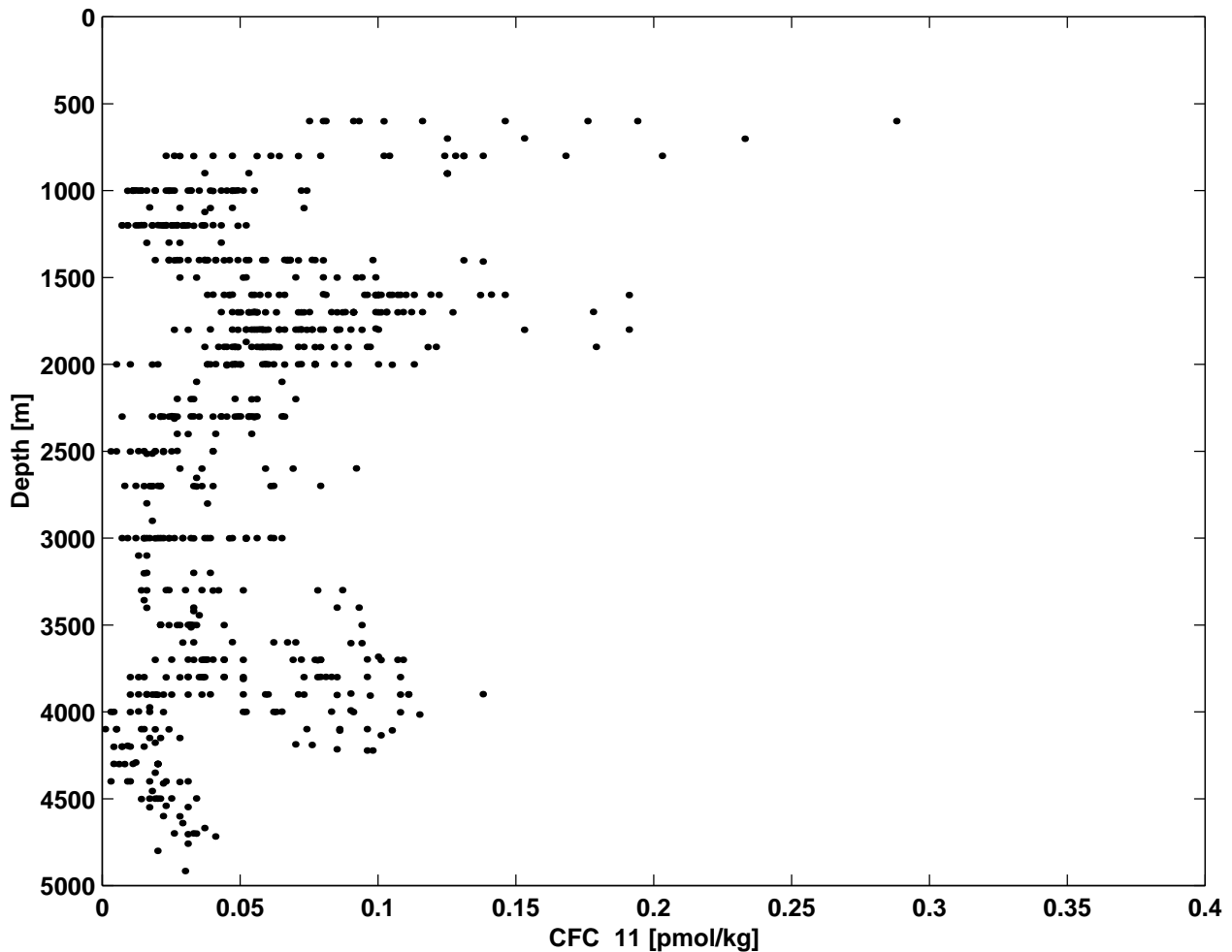
Figure 3: All CFC-11 concentrations [ 0.1 \text{ pmol/kg}^{-1} ] versus depth.
