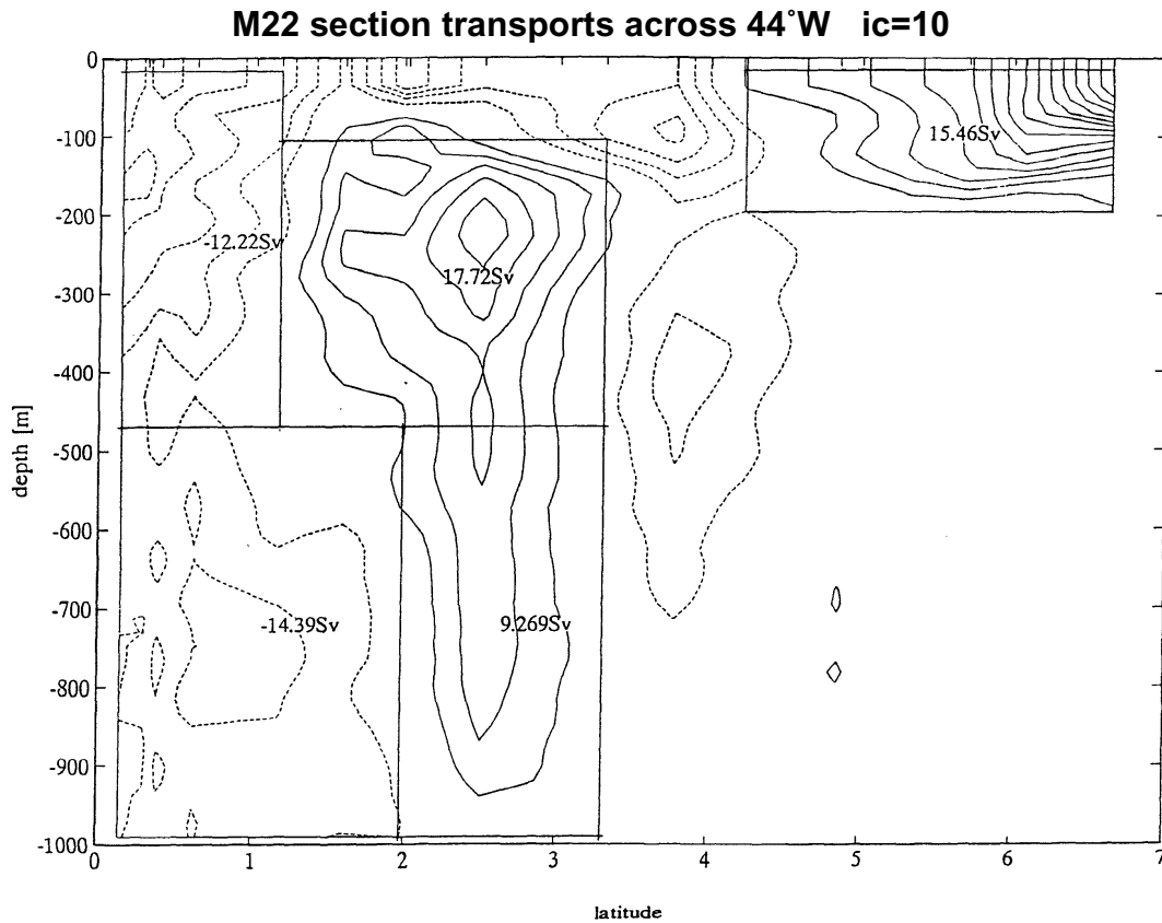
Fig. 16: IADCP: velocity pattern (u-component, cm/s) of the upper 1000 m at 44°W. Transport calculations for the framed regions are included. Numbers are in Sv, positive is directed east.
