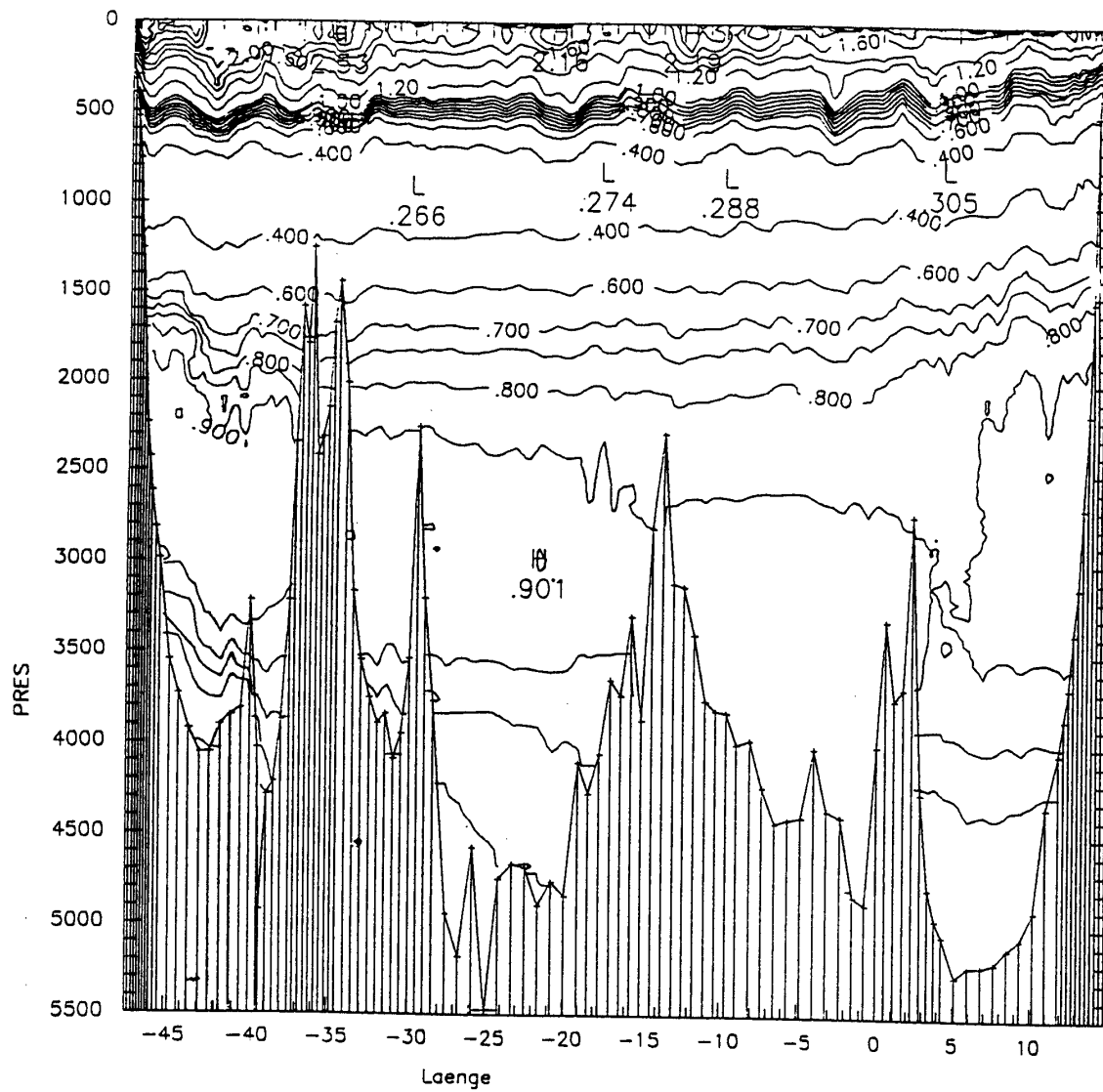
Fig. 31: Salinity-34 along 30°S. Contour interval: 0,05
