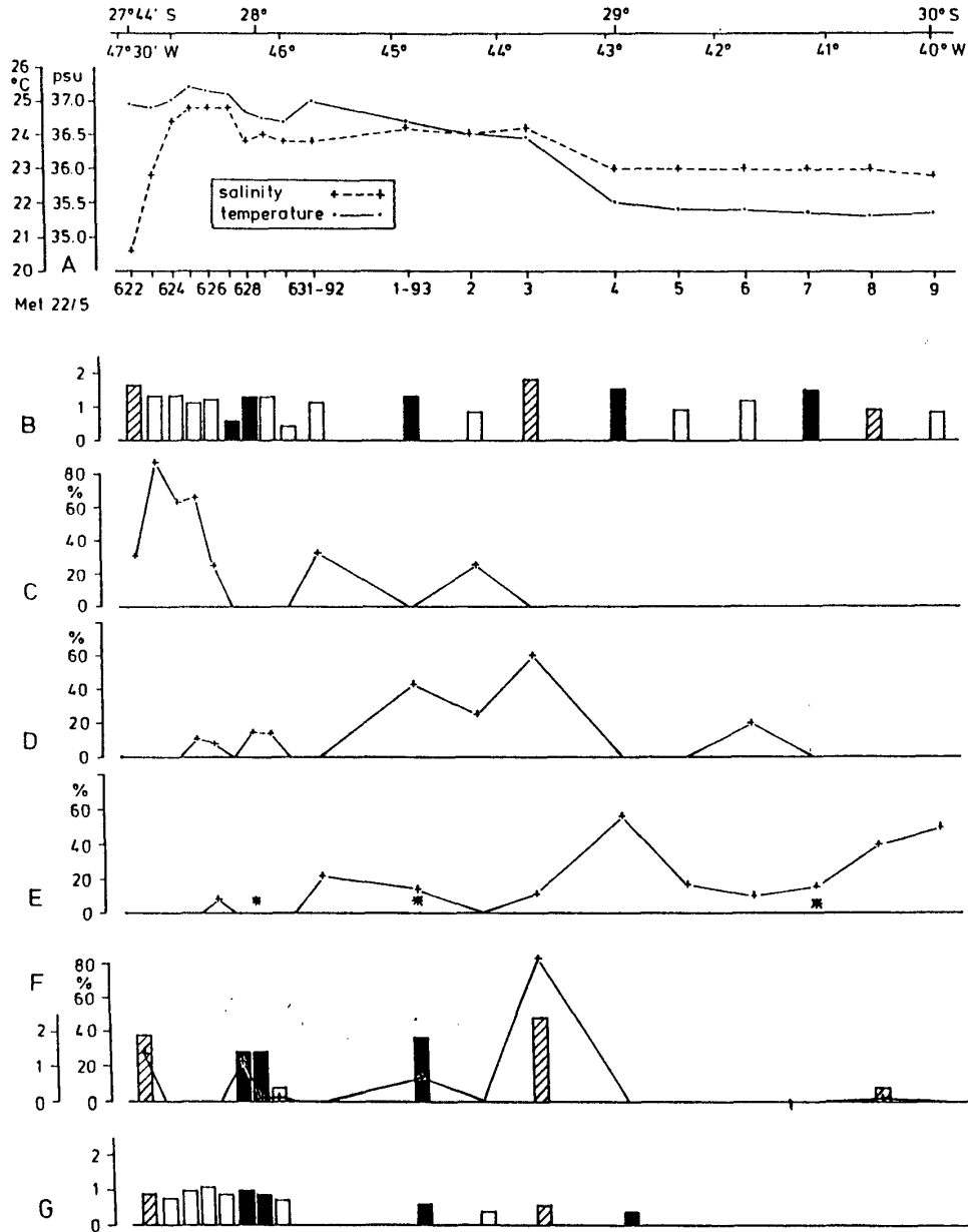
Fig. 34: Hydrographical and biological distribution pattern at the sea surface from Brazil to 40° W.
