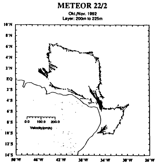
Fig. 22: VM-ADCP: Velocities along the cruise track for different depth layers.
