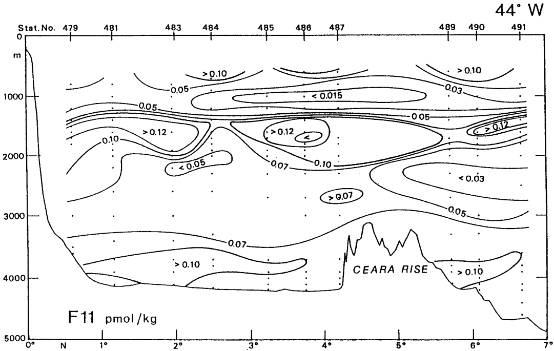
Fig. 15: Freon-11 distribution (pmol/kg) at the 44°W section.
