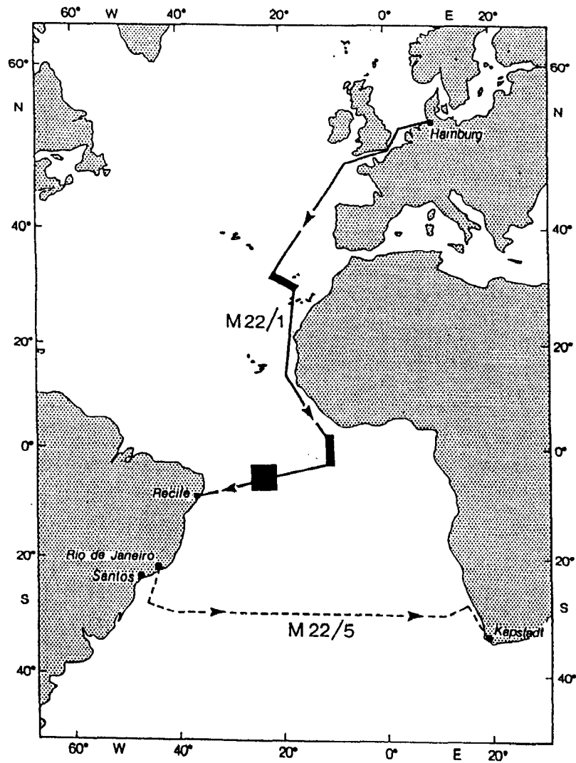
Figure 1a: Track and working areas of METEOR cruise no. 22, leg 5 (WOCE A05) and leg 1 (non-WOCE)
