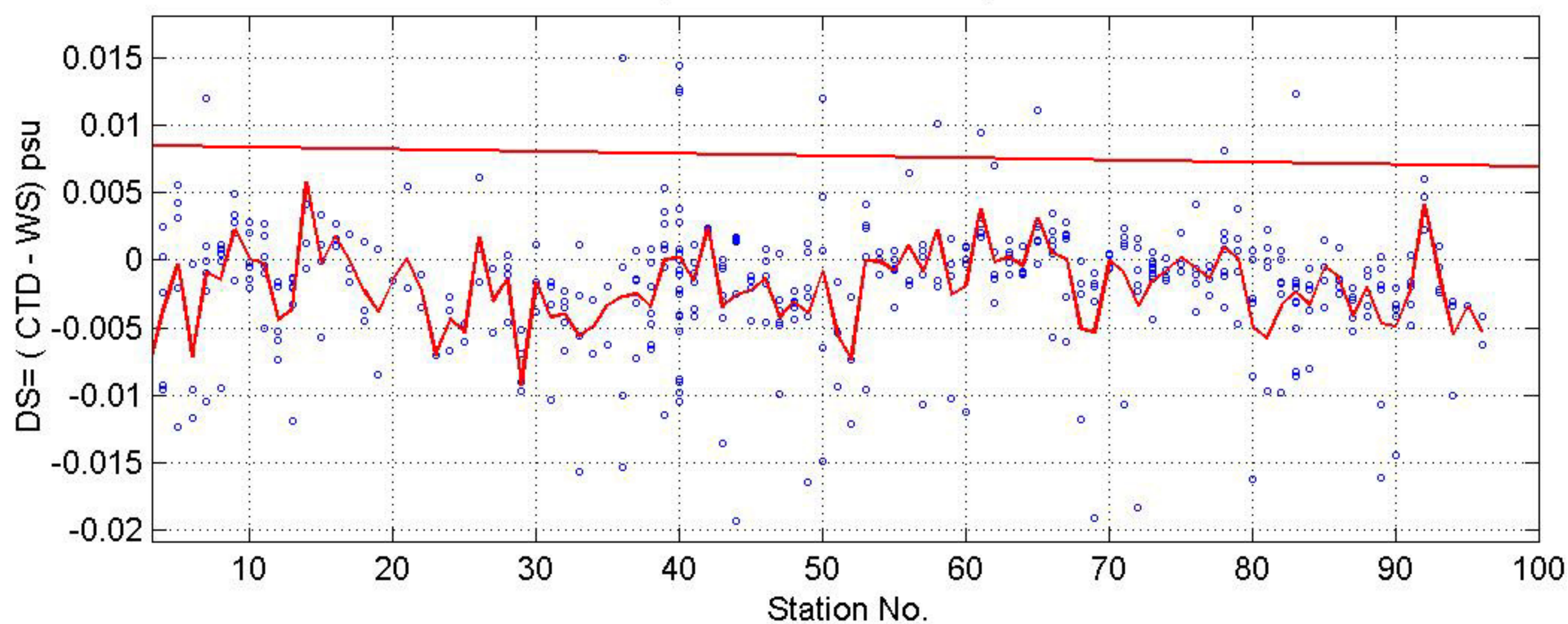
DS down for pressures &gt; 1000 dbar; std-s= 0.00527
