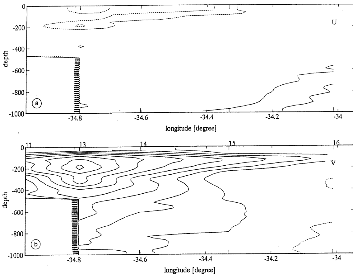
Fig. 17: IADCP: velocity pattern (cm/s) at the 5°S section
