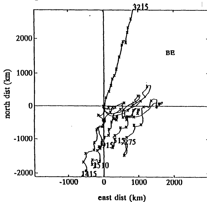
Fig. 28: Progressive vector diagrams from (a) the deepest mooring of the heat flux array ACM3 (BE/335) All curves start at the origin, crosses indicate 50 day intervals, numbers depths in m.
