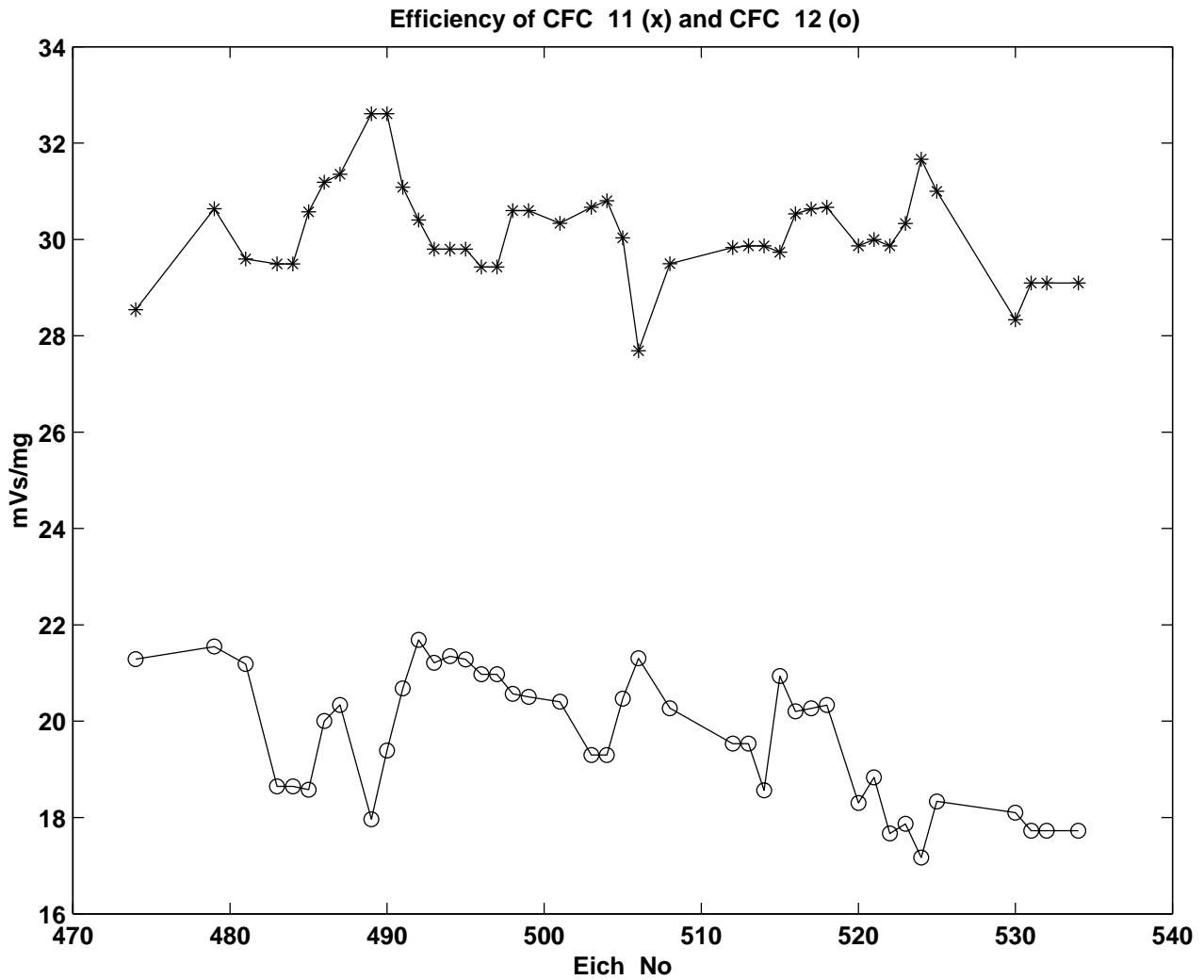
Figure 2: Temporal evolution of the efficiency of the ECD (mVs/mg standard) for the 0.25 mL sample volume.
