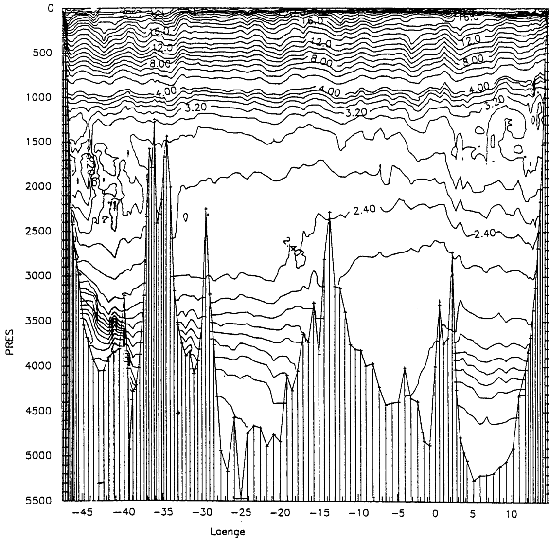
Fig. 30: Potential temperature along 30°S. Contour interval 4 - 25°C: 1°C 0 - 4°C: 0,2°C
