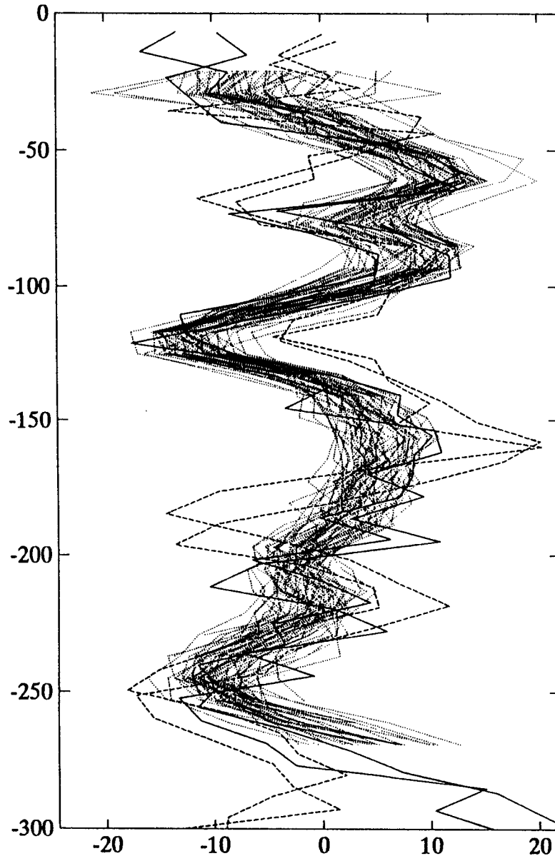
Fig. 21: Zonal current profiles at station S6 (approx. 1000m water depth). The solid lines are the Pegasus profile (down and up cast) on 8 Nov. 1992. The family of dotted curves are ship ADCP profiles during the 4 hours on station there. The dashed curves are the corresponding Pegasus profile from 24 Oct. During the 4 hours on station, the profile is remarkably constant. 2 weeks earlier, many of the features are the same, but the direction of jets had changed.
