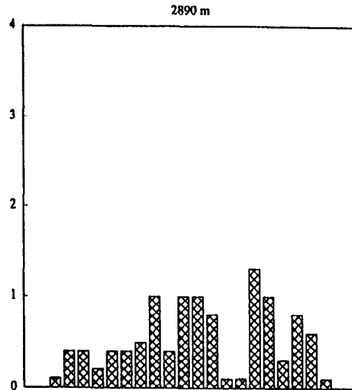
Fig. 10a-c: Volume (arbitrary units) of particles in individual cups of the three sediment traps attached to mooring EA8 (recovered at 6°S in the Gulf of Guinea). The traps started sampling on December 15, 1991 and the last cup stopped sampling at October 6, 1992. For further details see chapter 7.1.2
