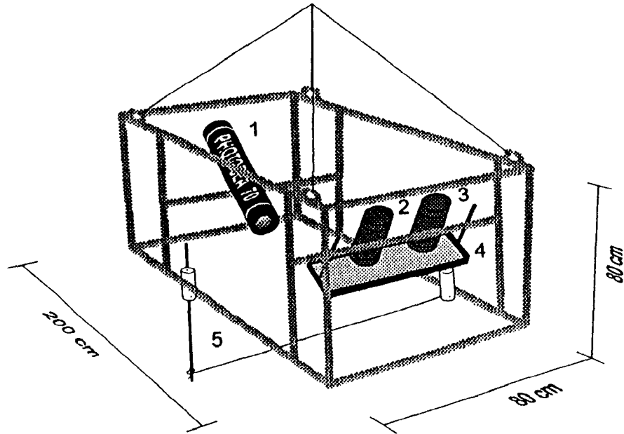
Fig. 11: Perspective view and size of the particle camera system: 1: 70 mm 2 and 3: 150 W-strobes PHOTOSEA 1500s 4: Collimator, consisting of two 30 x 30 cm highly refractive fresnel lenses, mounted in a steel frame. Distance between fresnel lenses and strobe lights is variable 5: Adjustable holder for a 0.5 mm nylon line used as size standard
