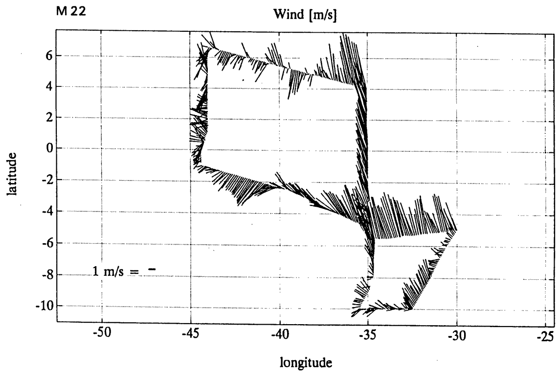
Fig. 25: DVS: winds along cruise track
