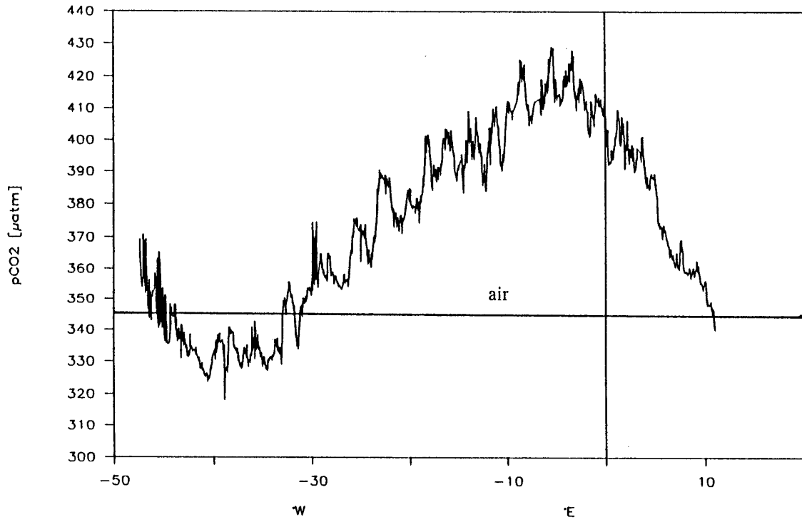
Fig. 33: CO 2 partial pressure in surface water and atmosphere along 30° S
