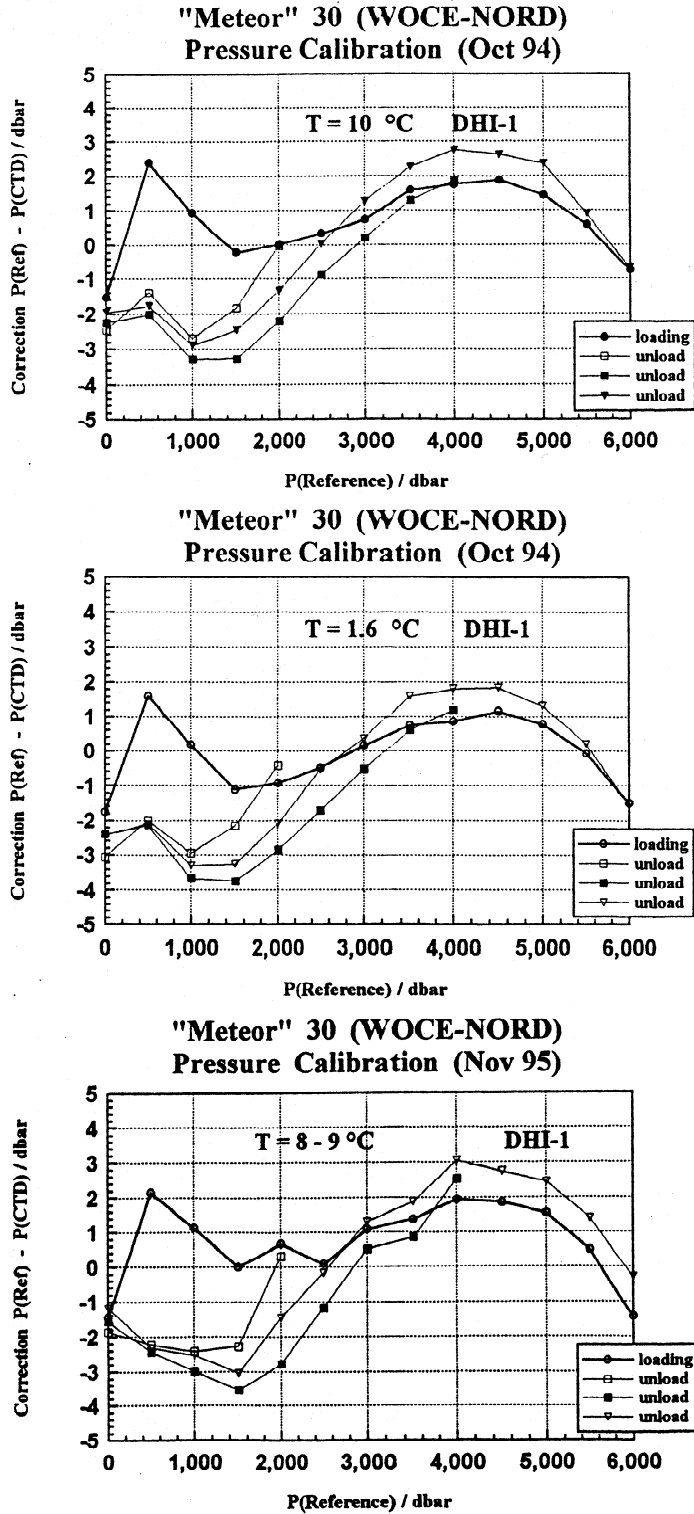
Fig. (13) Pre- and post -cruise calibration (a) Pressure at T = 10°C (Oct 94) (b) Pressure at T = 1.6°C (Oct 94) (c) Pressure at T = 8-9°C (Nov 95)
