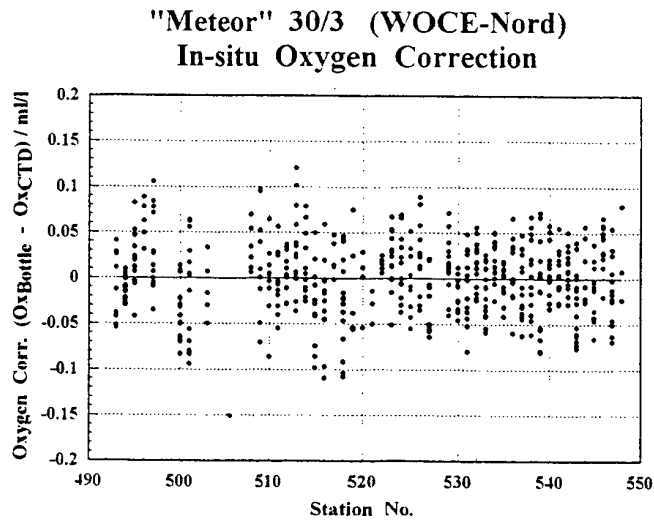
Fig. (15) Oxygen residuals of final fit versus CTD stations
