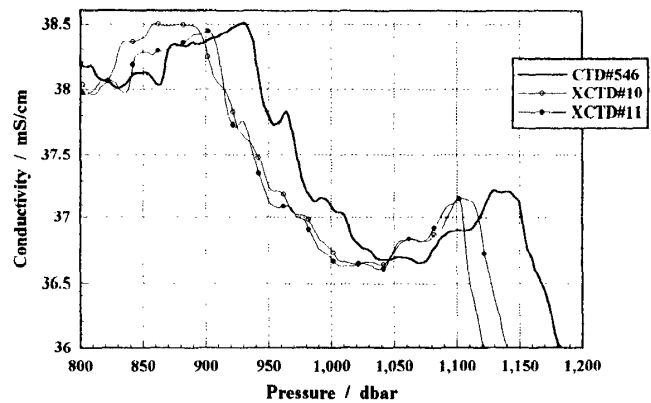
Fig. (26) CTD and XCTD conductivity profiles of the deeper layers (a) at stat. # 542, (b) at stat. # 546
