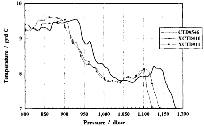
Fig. (24) CTD and XCTD temperature profiles of deeper layers (a) at stat. # 542, (b) at stat. # 546
