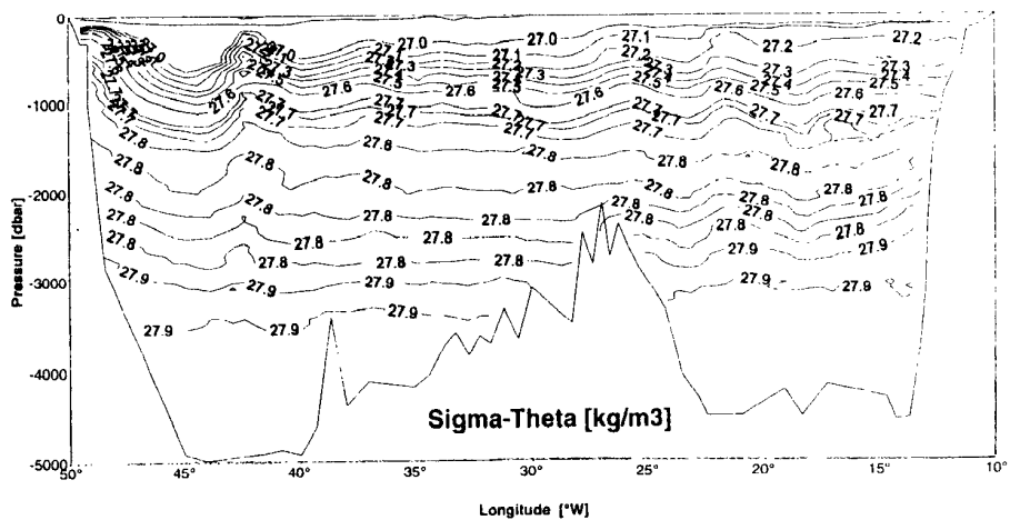
Fig. (7d) Density \sigma_\theta distribution along WHP-A2
