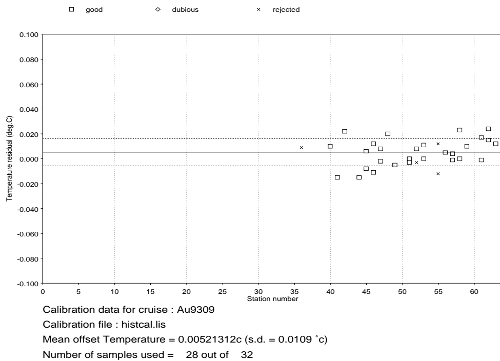
Figure 3a and b: Temperature residual ( T_{\text{therm}} - T_{\text{cal}} ) versus station number for SR3. The solid line is the mean of all the residuals; the broken lines are \pm the standard deviation of all the residuals (as defined in section A2.14 , Appendix 2). Note that the “dubious” and “rejected” categories refer to the conductivity calibration.
