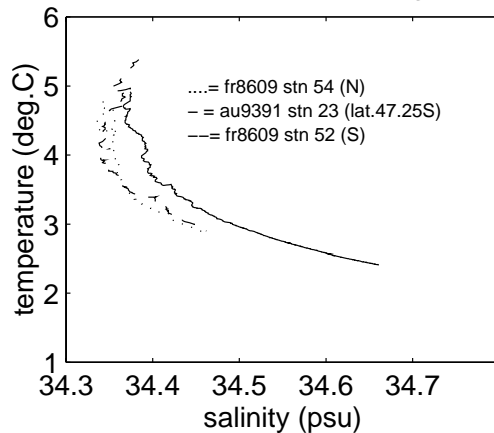
(c) 1000 to 2000 dbar TS diagram
