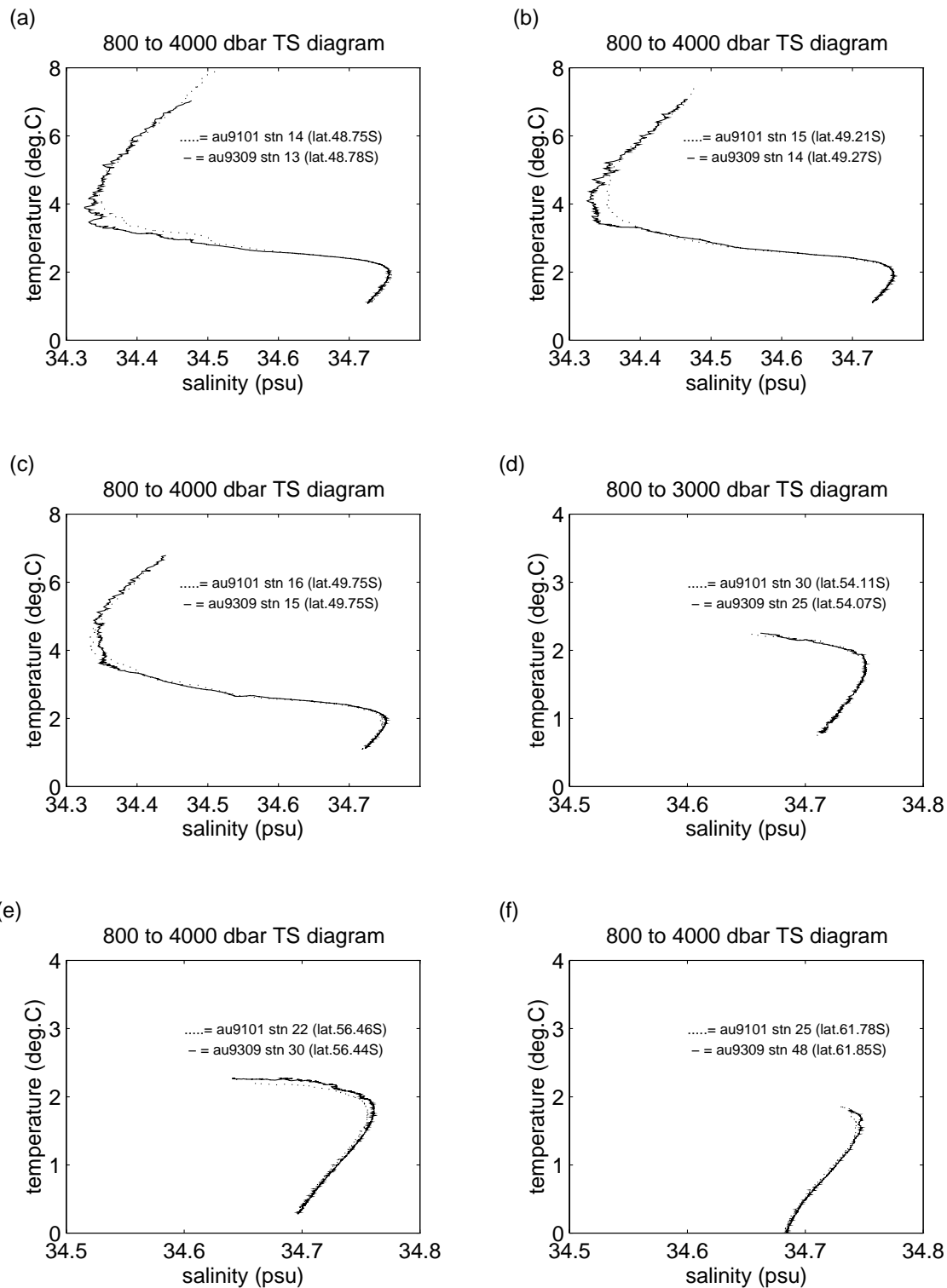
Figure A6.1: TS diagrams for comparison of au9309 and au9101 data.
