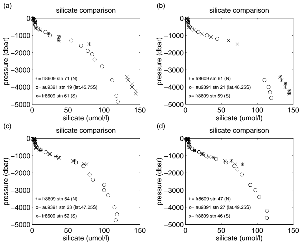
Figure A6.13: Silicate vertical profile comparisons for au9391 and fr8609 data.
