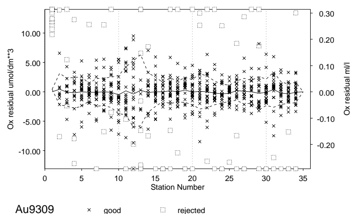
Figure 6: Dissolved oxygen residual ( o_{\text{btl}} - o_{\text{cal}} ) versus station number for SR3 stations 1 to 35. The solid line follows the mean residual for each station; the broken lines are \pm the standard deviation of the residuals for each station (as defined in section A2.14 , Appendix 2).
