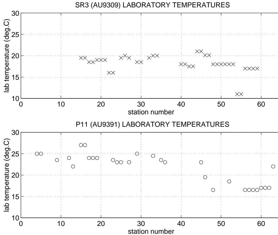
Figure 2: Hydrology laboratory temperatures at the times of dissolved oxygen analyses.
