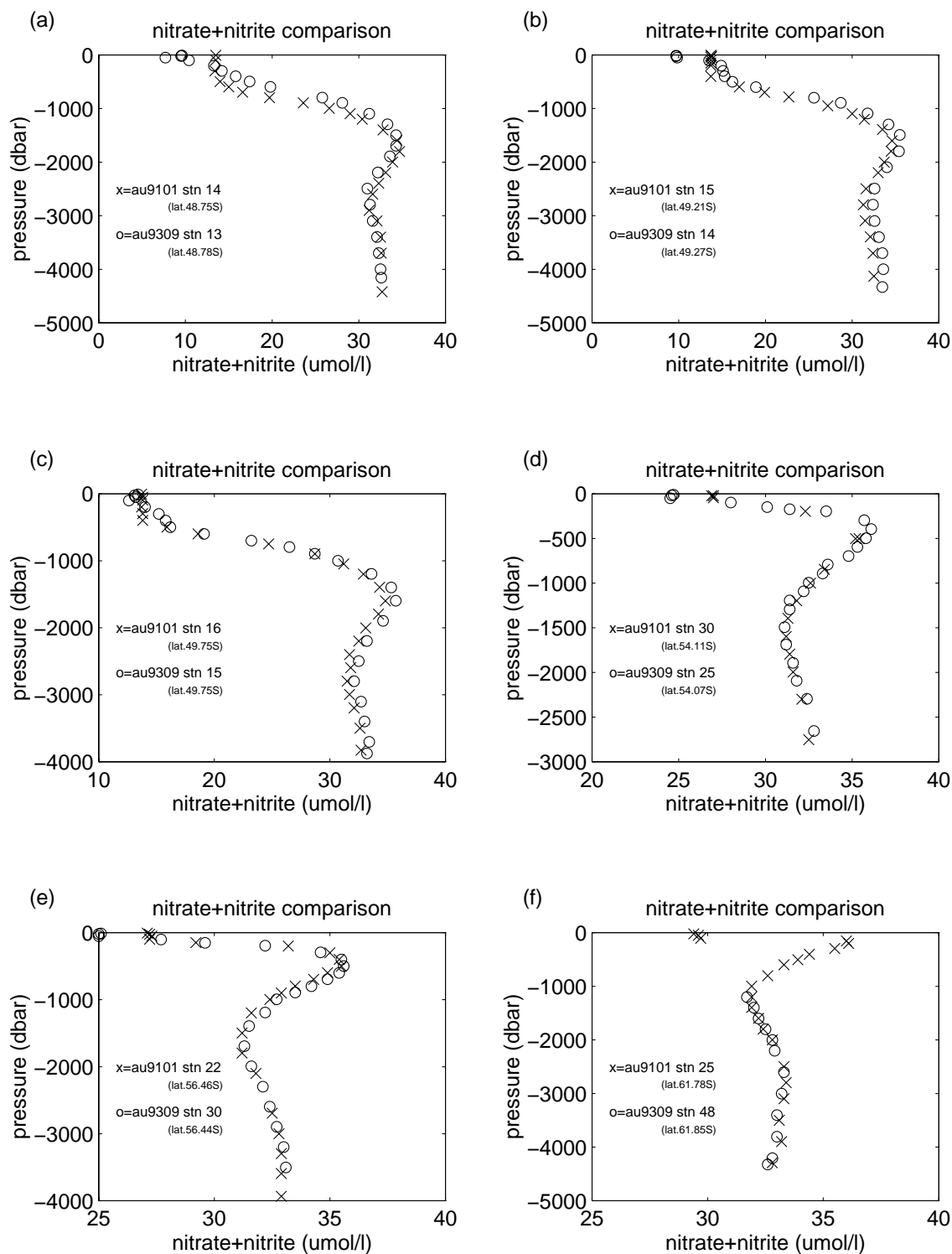
Figure A6.5: Nitrate+nitrite vertical profile comparisons for au9309 and au9101 data.
