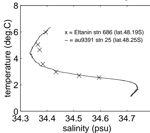
(b) 800 to 4000 dbar TS diagram
