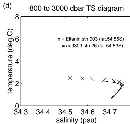
Figure A6.2: TS diagrams for comparison of au9309 and Eltanin data.
