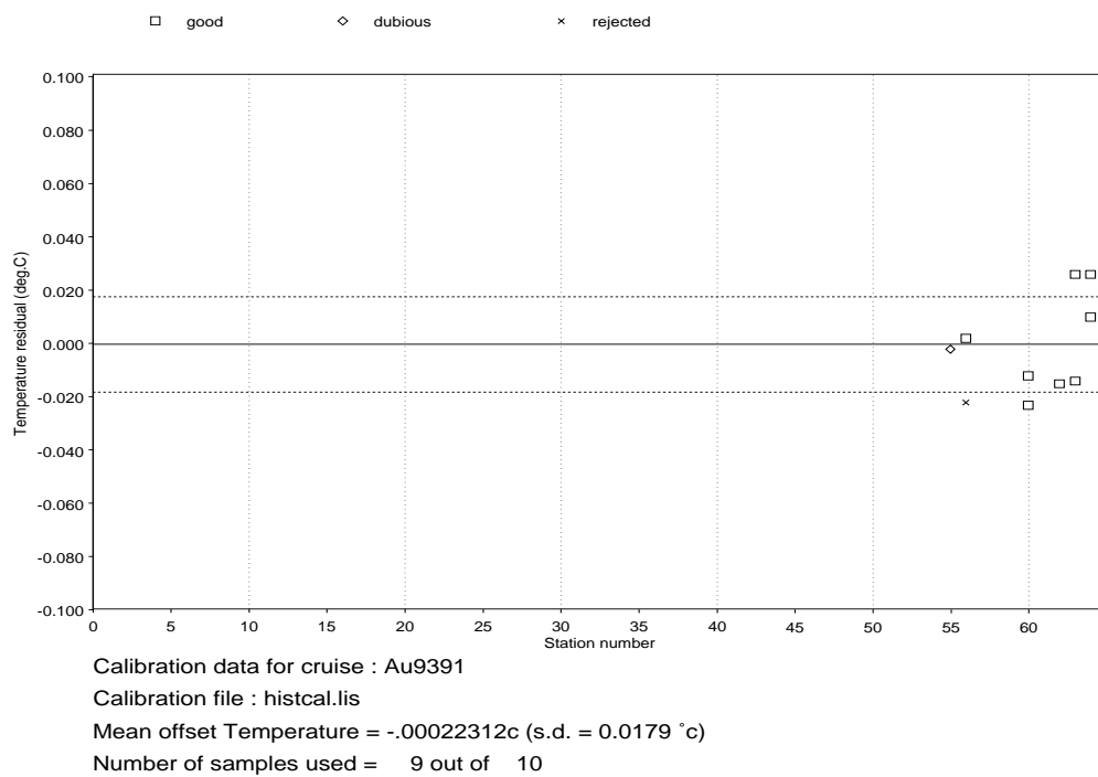
Figure 3c and d: Temperature residual ( T_{\text{therm}} - T_{\text{cal}} ) versus station number for P11 and sea ice stations. The solid line is the mean of all the residuals; the broken lines are \pm the standard deviation of all the residuals (as defined in section A2.14 , Appendix 2). Note that the “dubious” and “rejected” categories refer to the conductivity calibration.
