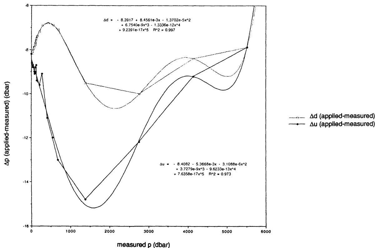
Figure A1.1a and b: Pressure sensor calibration data, for down and upcast calibrations. In the figures, \Delta d is for downcast data, and \Delta u is for upcast data (calibrated August 1991).
