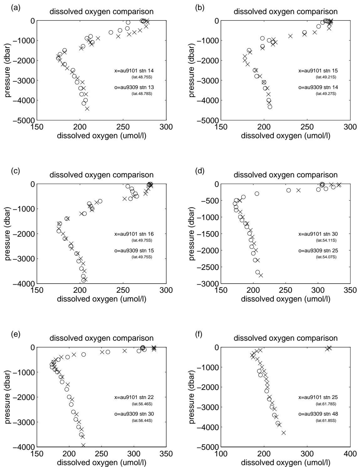
Figure A6.3: Dissolved oxygen vertical profile comparisons for au9309 and au9101 data.
