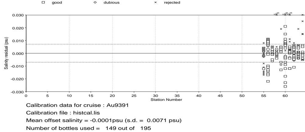
Figure 5a to d: Salinity residual ( s_{btl} - s_{cal} ) versus station number for SR3, P11 and sea ice stations. The solid line is the mean of all the residuals; the broken lines are \pm the standard deviation of all the residuals (as defined in section A2.14 , Appendix 2).
