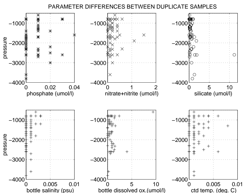
Figure 7: Absolute value of parameter differences between sample pairs derived from Niskin bottle pairs tripped at the same depth. Note that no pressure dependent trend is evident.
