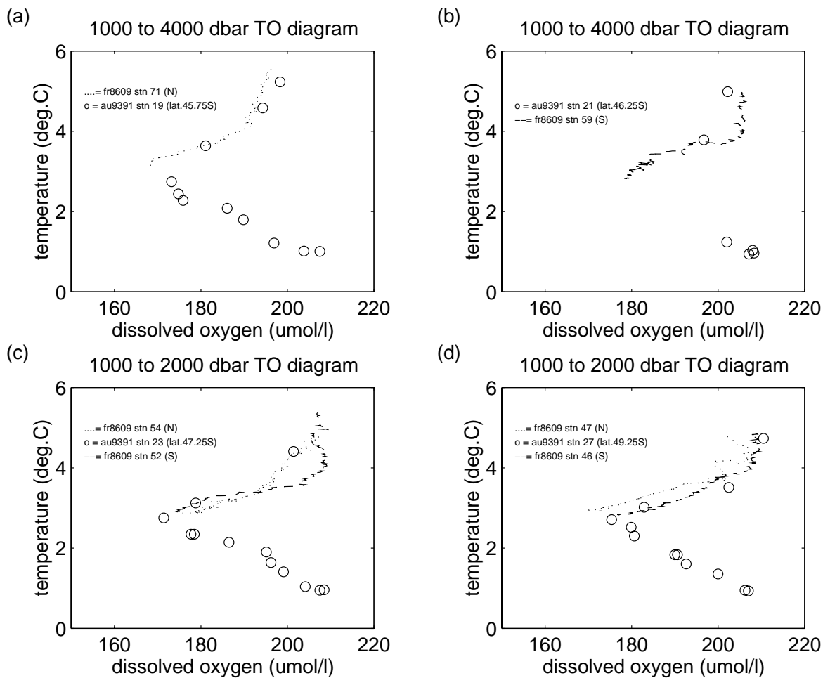
Figure A6.9: TO diagrams for comparison of au9391 and fr8609 data.
