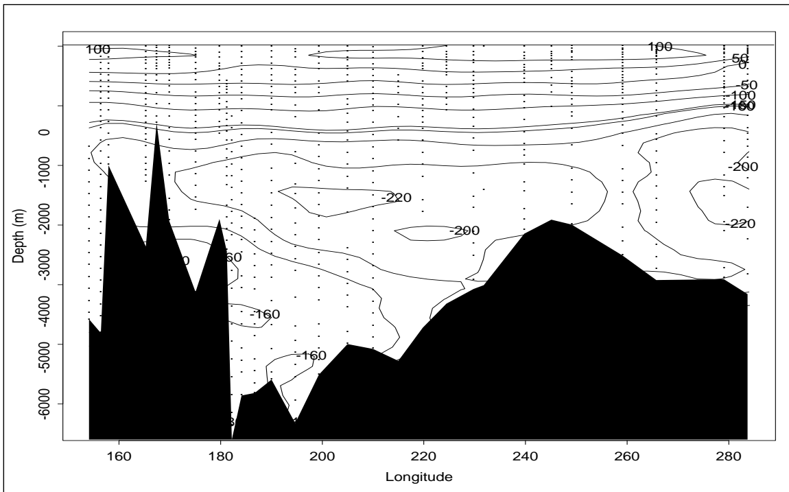
Figure 5: \Delta^{14}\text{C} contour of WOCE section P6 at approximately 32^\circ\text{S} . Longitudes are east of Greenwich. Objective gridding done using the LeTraon (1990) method with a relative long horizontal correlation length scale. The samples in the near bottom water mass centered on 190^\circ and having relatively low \Delta^{14}\text{C} are those which fall above the general deep water trend in Figure 3.
