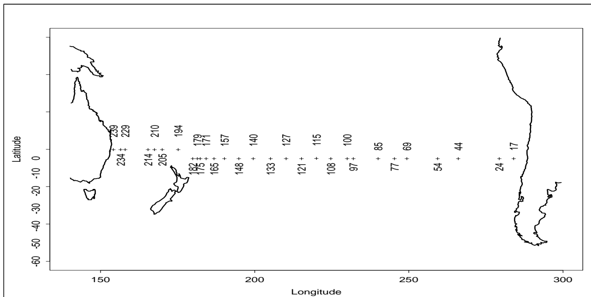
Figure 1: 14 C station locations for WOCE P6. All 14 C sampling was carried out using the AMS technique with sample distribution somewhat sparser than used on meridional WOCE lines.
