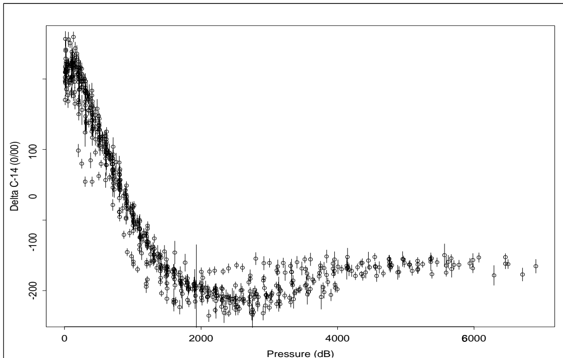
Figure 2: AMS \Delta^{14}\text{C} results for P6 stations shown with 2\sigma error bars. Only those measurements having a quality control flag value of 2 are plotted.
