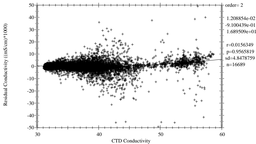
CTD #1, IO95 stas 148-800 residual conductivity slope, after linear corrnx
