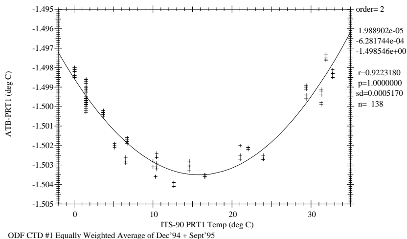
Figure 8.2.1 WOCE95 Primary temperature correction for ODF CTD #1, Dec.94/Sept.95 equally weighted average.
