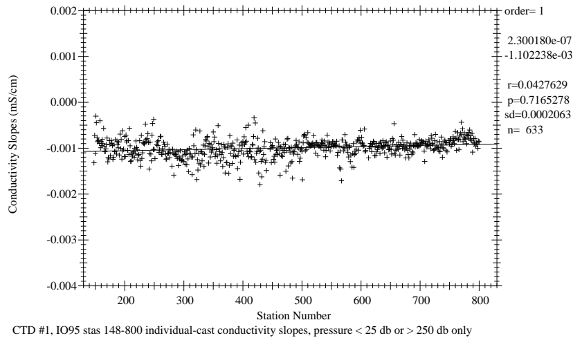
Figure 8.3.0 CTD #1 prelim. conductivity slopes for WOCE95 stations 148(I9N) through 800(I7N).
