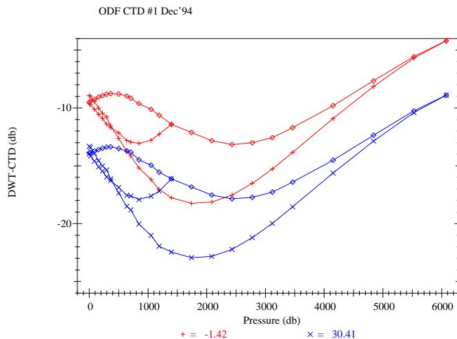
Figure 7.0 Pressure calibration for ODF CTD #1, December 1994.
