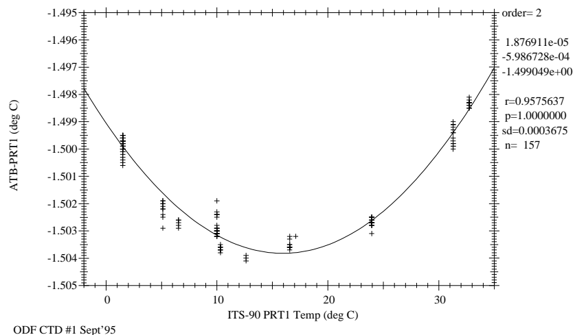
Figure 7.3 Primary PRT Temperature Calibration for ODF CTD #1, September 1995.
