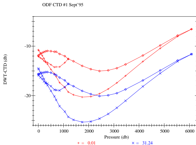
Figure 7.1 Pressure calibration for ODF CTD #1, September 1995.
