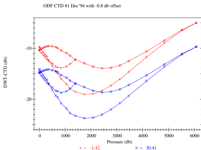
Figure 8.1.0 I4/I5W/I7C Pressure correction for ODF CTD #1: December 1994 calibration offset by -0.8 db.
