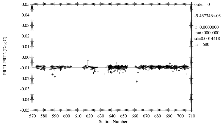
Figure 8.2.0 I4/I5W/I7C Shipboard comparison of CTD #1 primary/secondary PRT temperatures, pressure > 2000 db.
