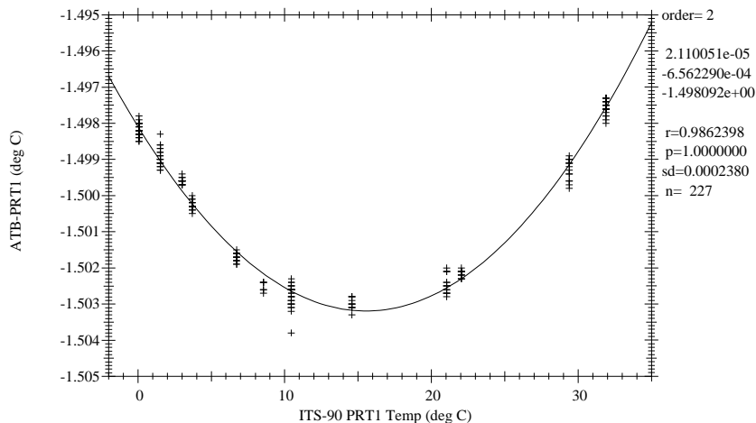
Figure 7.2 Primary PRT Temperature Calibration for ODF CTD #1, December 1994.
