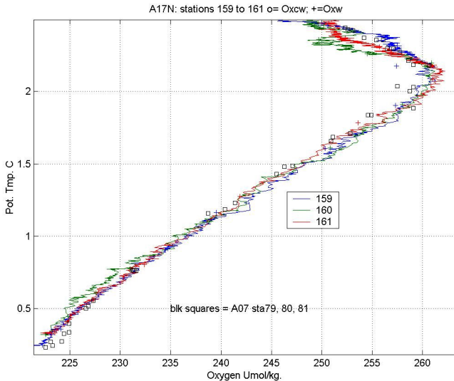
Figure 9a, b and c: Oxygen versus Potential Temperature for intersecting East/West WOCE section A07 (4.5S) compared to nearby stations of A17N
