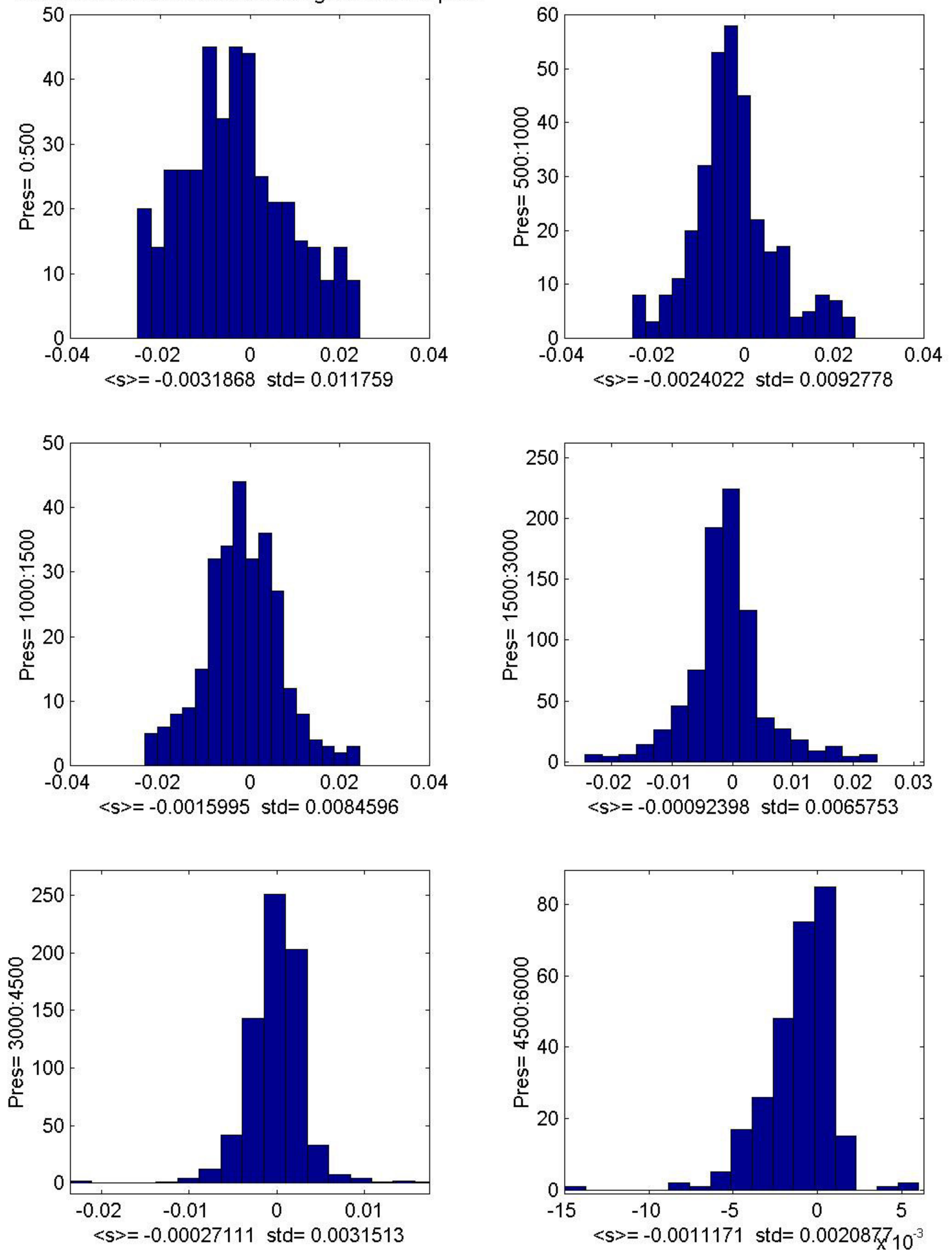
Figure 5a-f: Histograms of water sample salinities & CTD down profile salinity differences (DS= CTD-WS) at various pressures. The average salinity difference for all pressure intervals is -0.0012 psu and the 6 histograms with increasing pressure in figure 5 suggest that the CTD salinity is slightly too low at all pressures.
