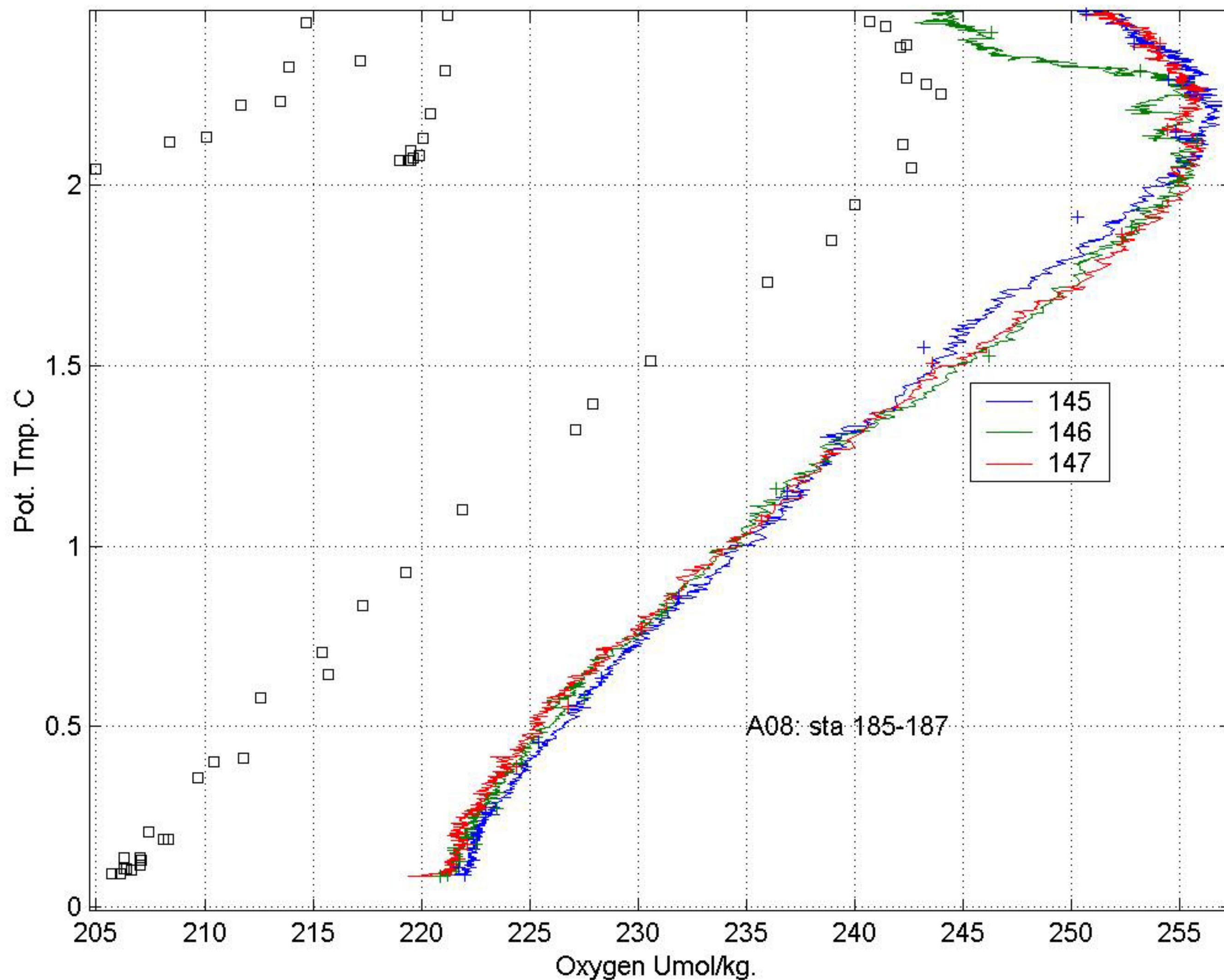
Figure 9a & b: Oxygen versus Potential Temperature for intersecting East/West WOCE sections A06 (7.5N) and A08 (11.2S). Oxygen values of A08 are low by 15 uM/kg and appear to be questionable.
