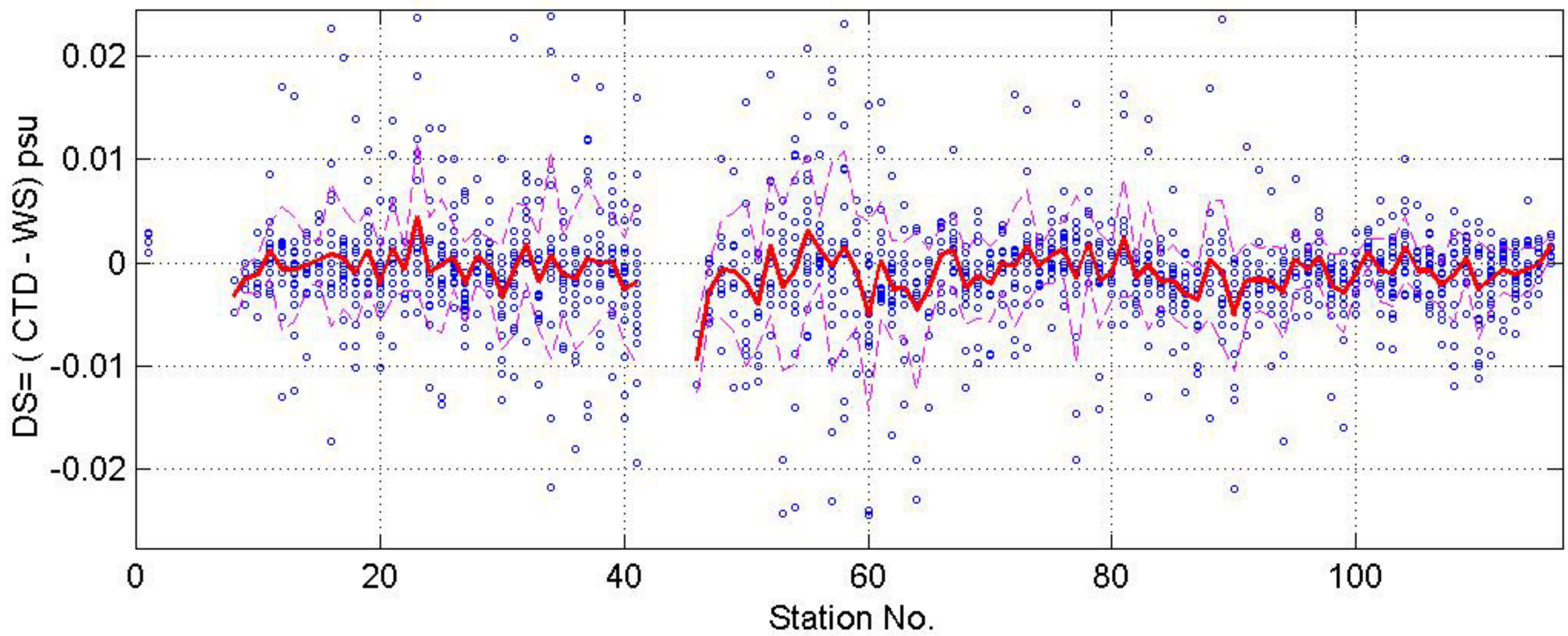
4b DS down for pressures > 1500 dbar; std-s= 0.00494
