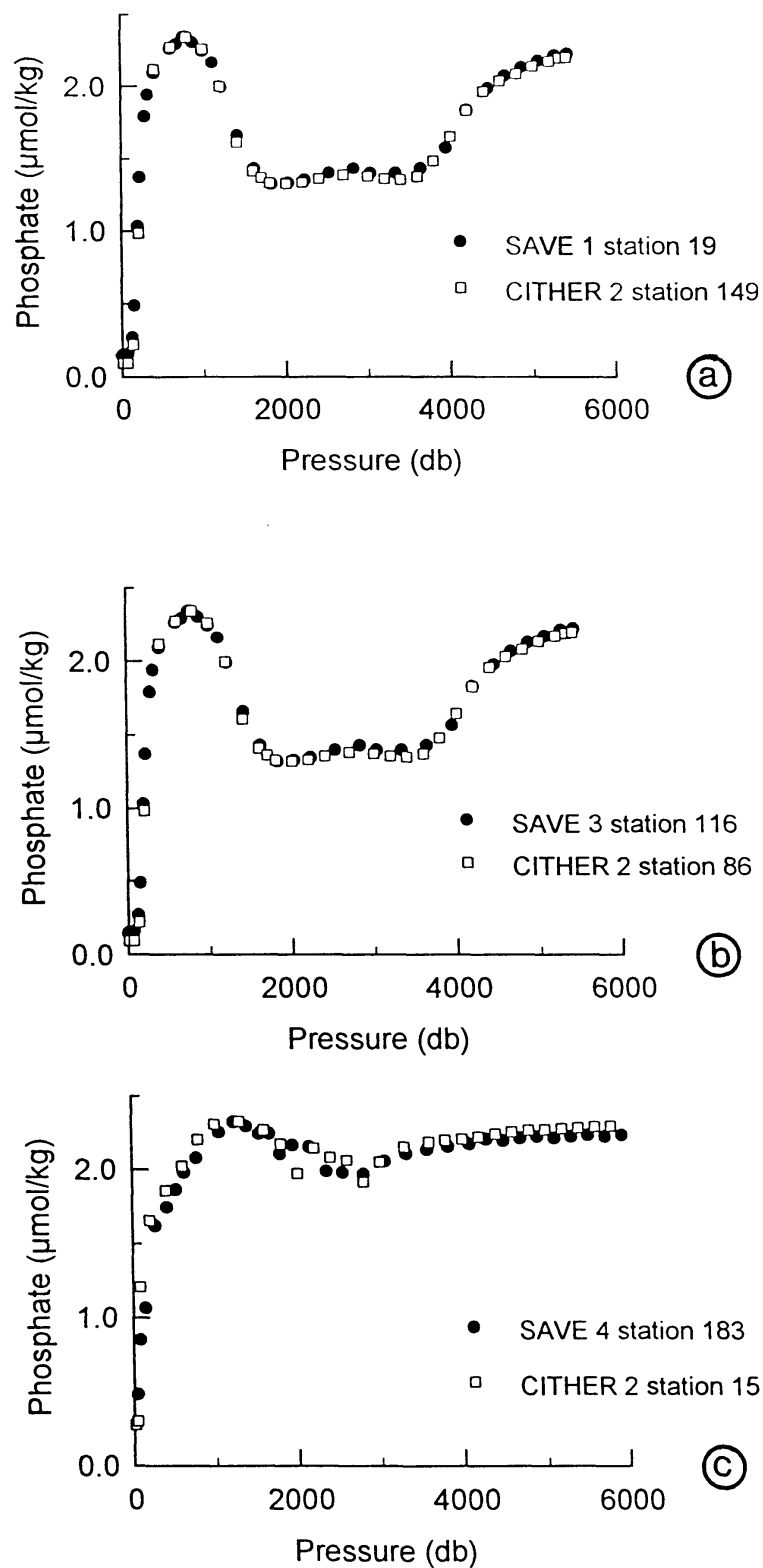
Figure IV-11: Comparison of phosphate profiles for the stations occupied at the same geographical position during CITHER 2 and SAVE cruises.
