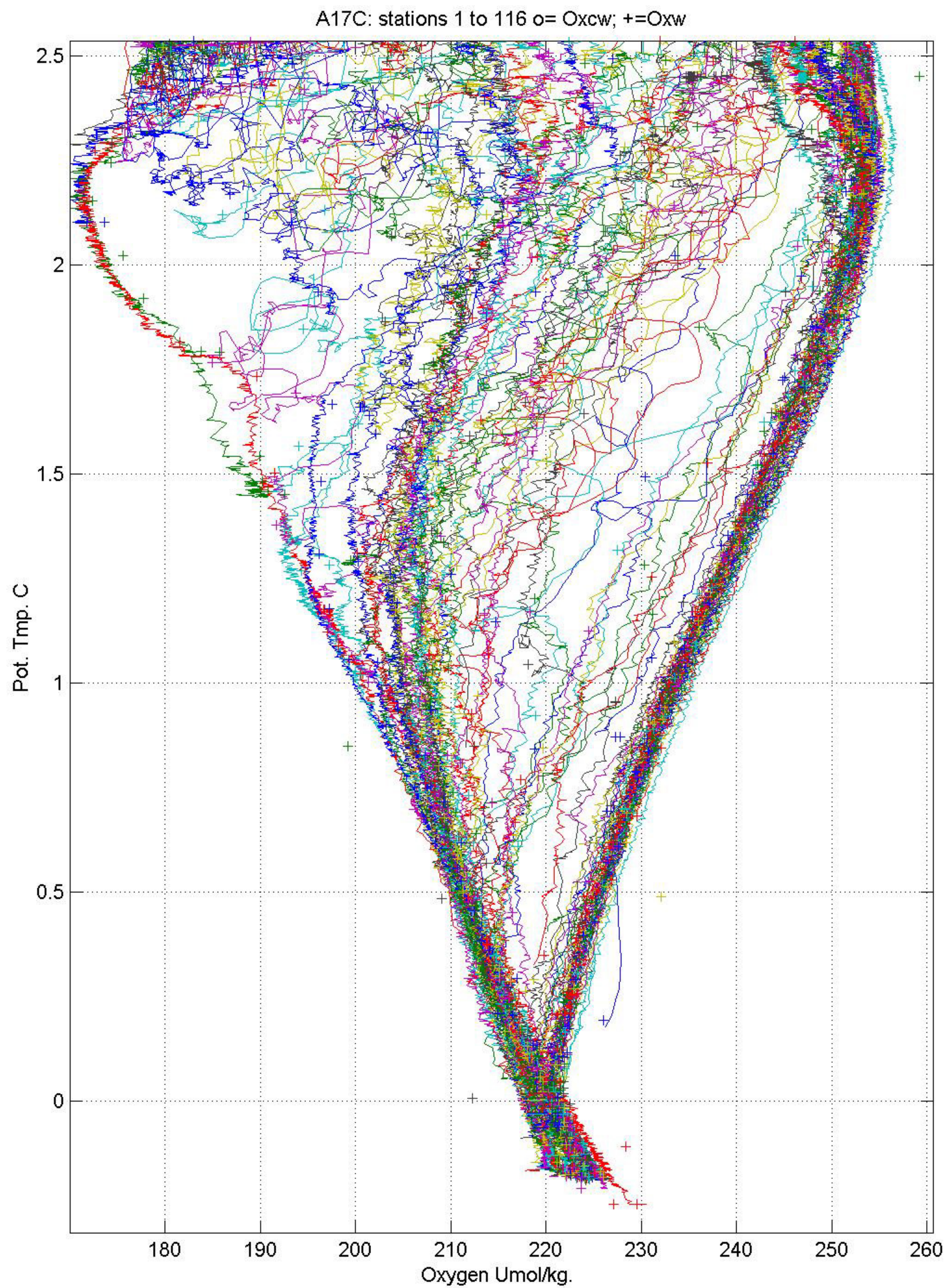
Figure 3b: deep-water plot oxygen versus Pot. Temperature.
