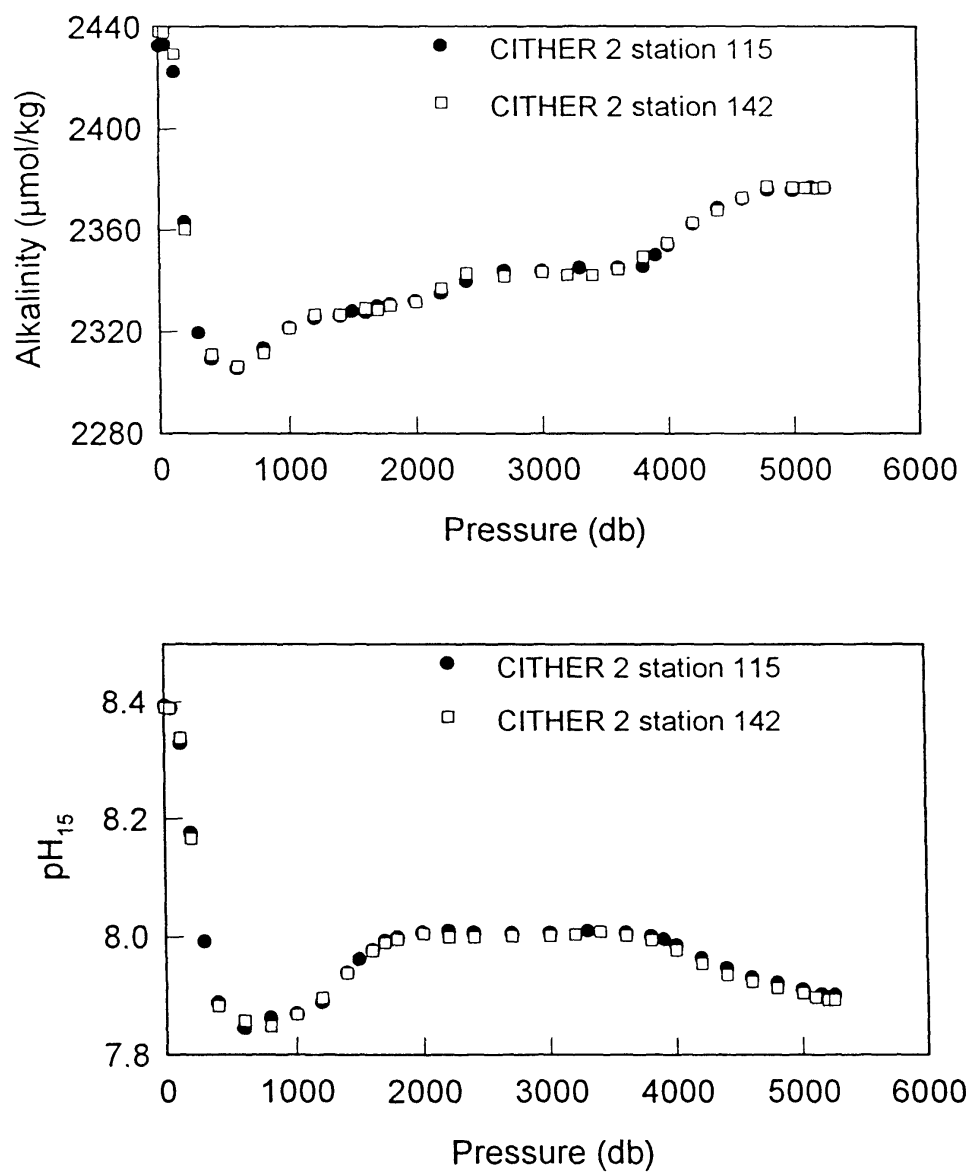
Figure VI-8: Comparison of vertical distributions of \text{pH}_{15} and alkalinity between stations 115 and 142 surveyed at the same geographical position.
