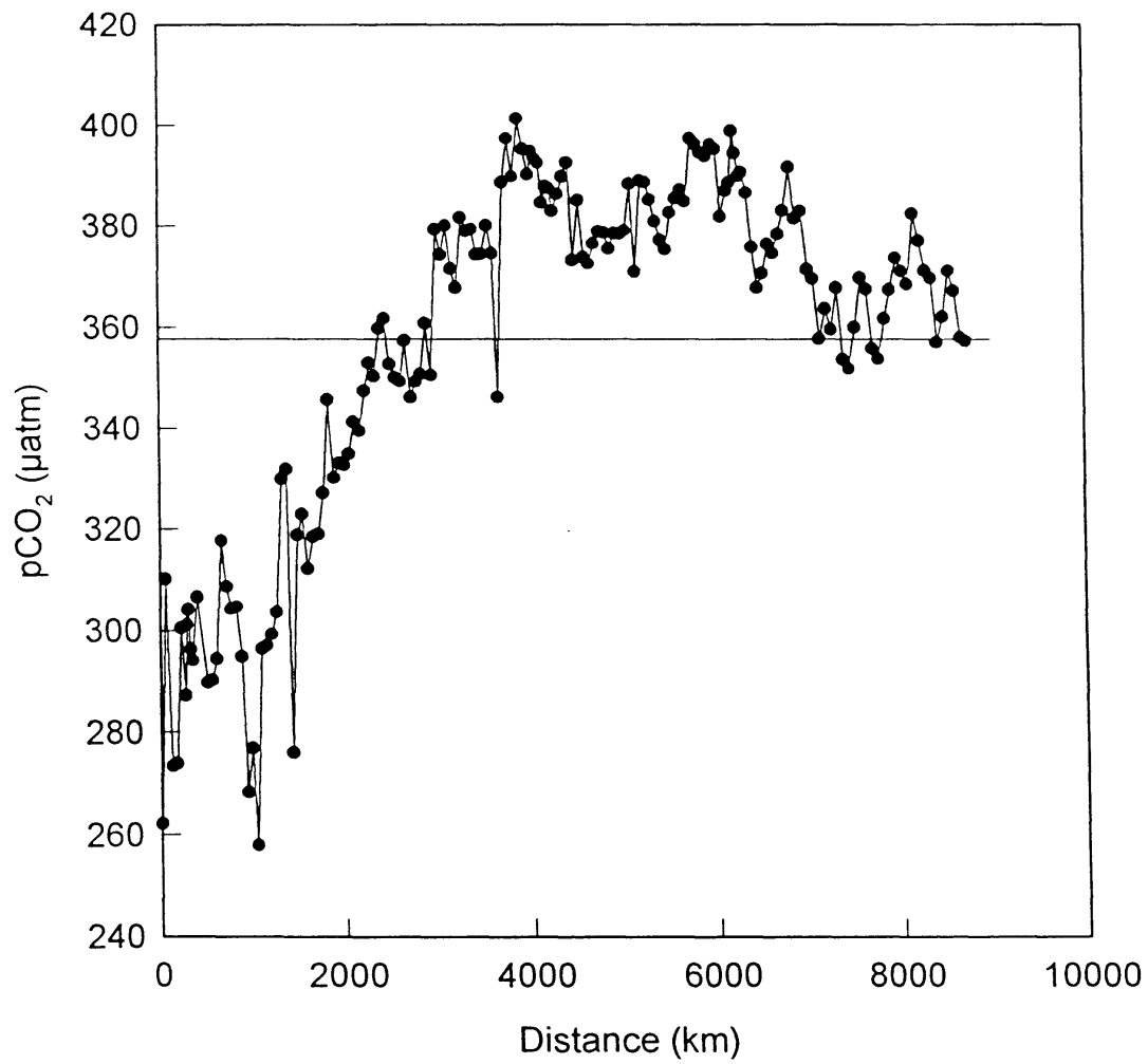
Figure VI-12: Distribution of surface p\text{CO}_2 along the main section. The straight line at 357.7 is the atmospheric p\text{CO}_2 for 1994 according to Keeling et al.(1995).
