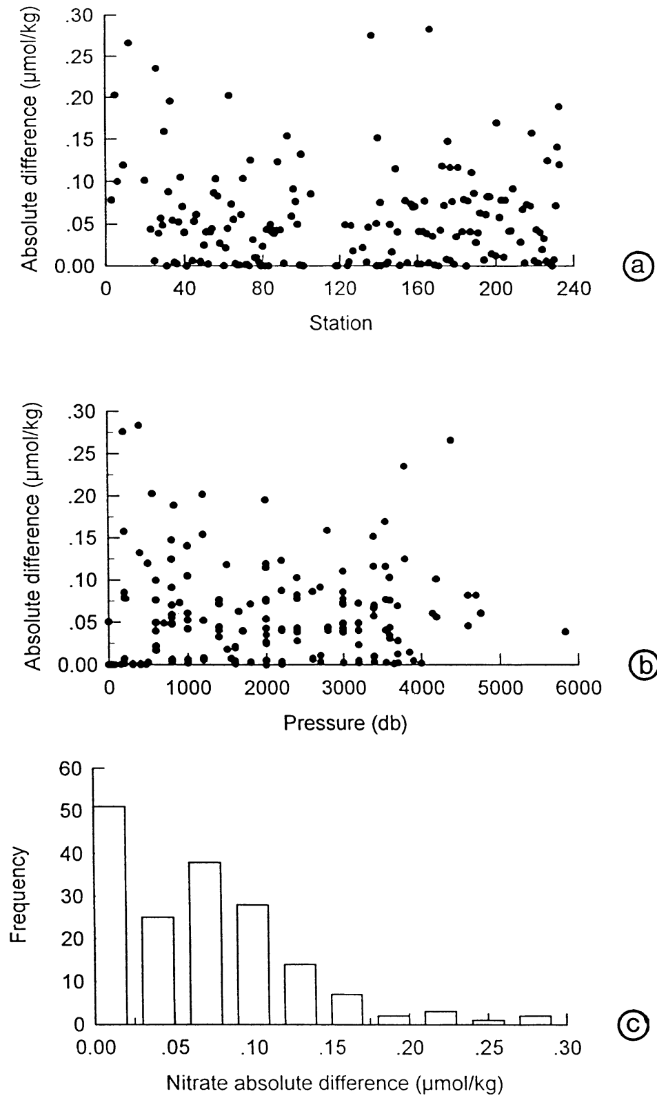
Figure IV-1: Absolute difference of nitrate concentrations for duplicate samples fired at the same level versus station number (a) and versus depth (b); and frequency distribution of the absolute difference (c).
