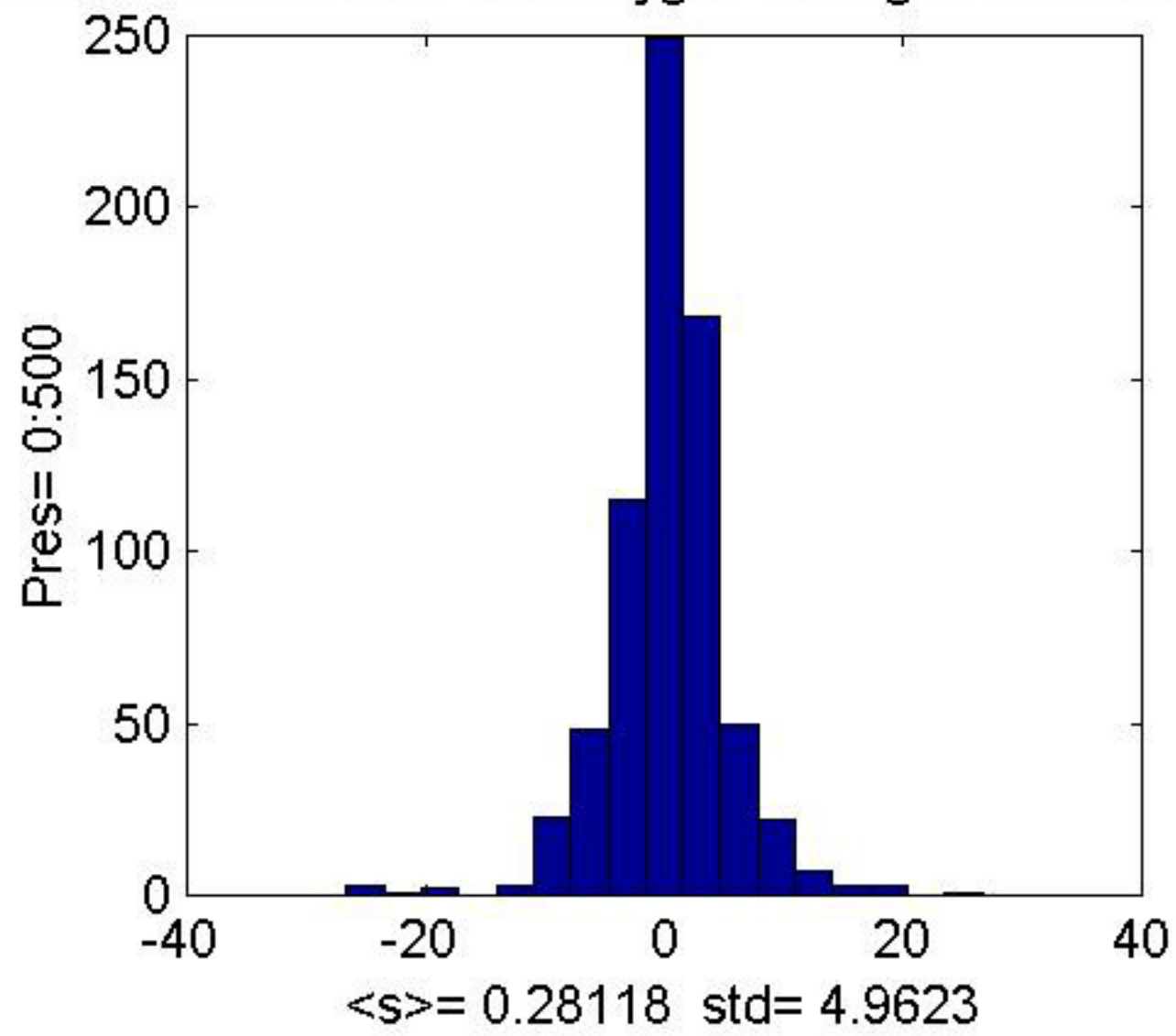
A17C: Down CTD - WS Oxygen Histograms versus pres.
