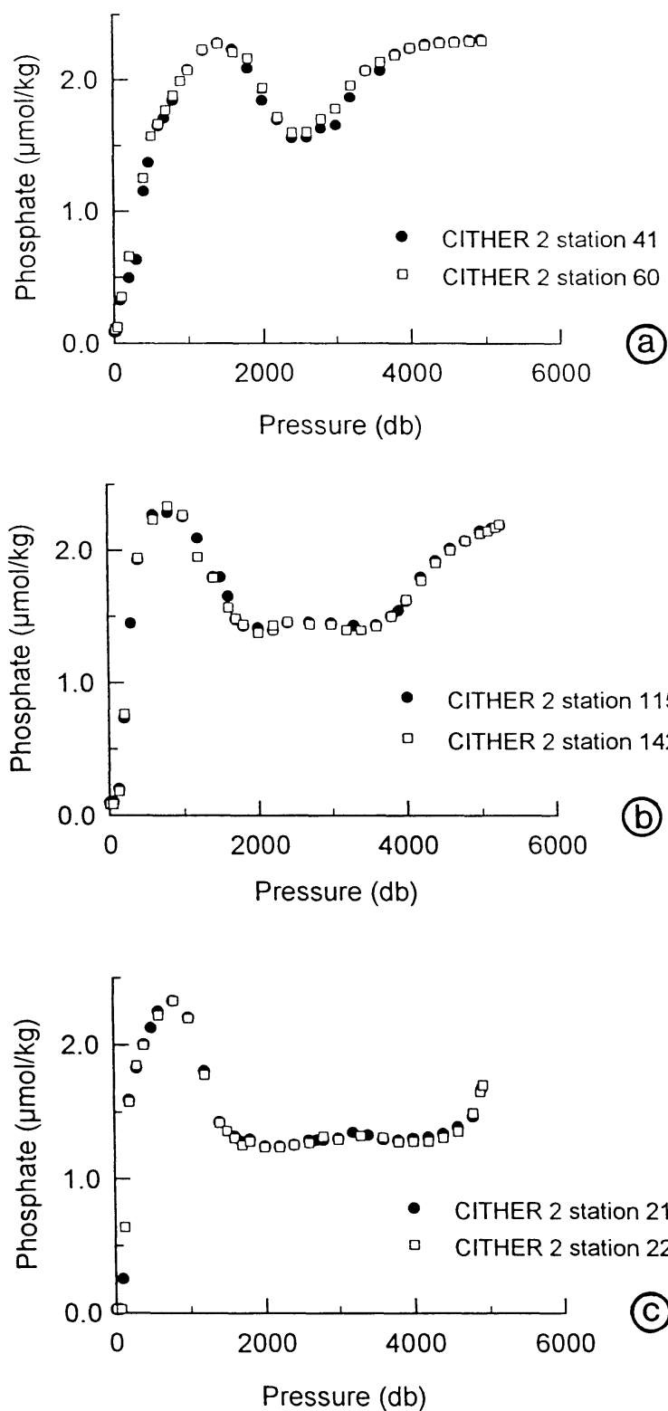
Figure IV-5: Comparison of phosphate profiles for the pairs of stations occupied at the same geographical position during the CITHER 2 cruise.
