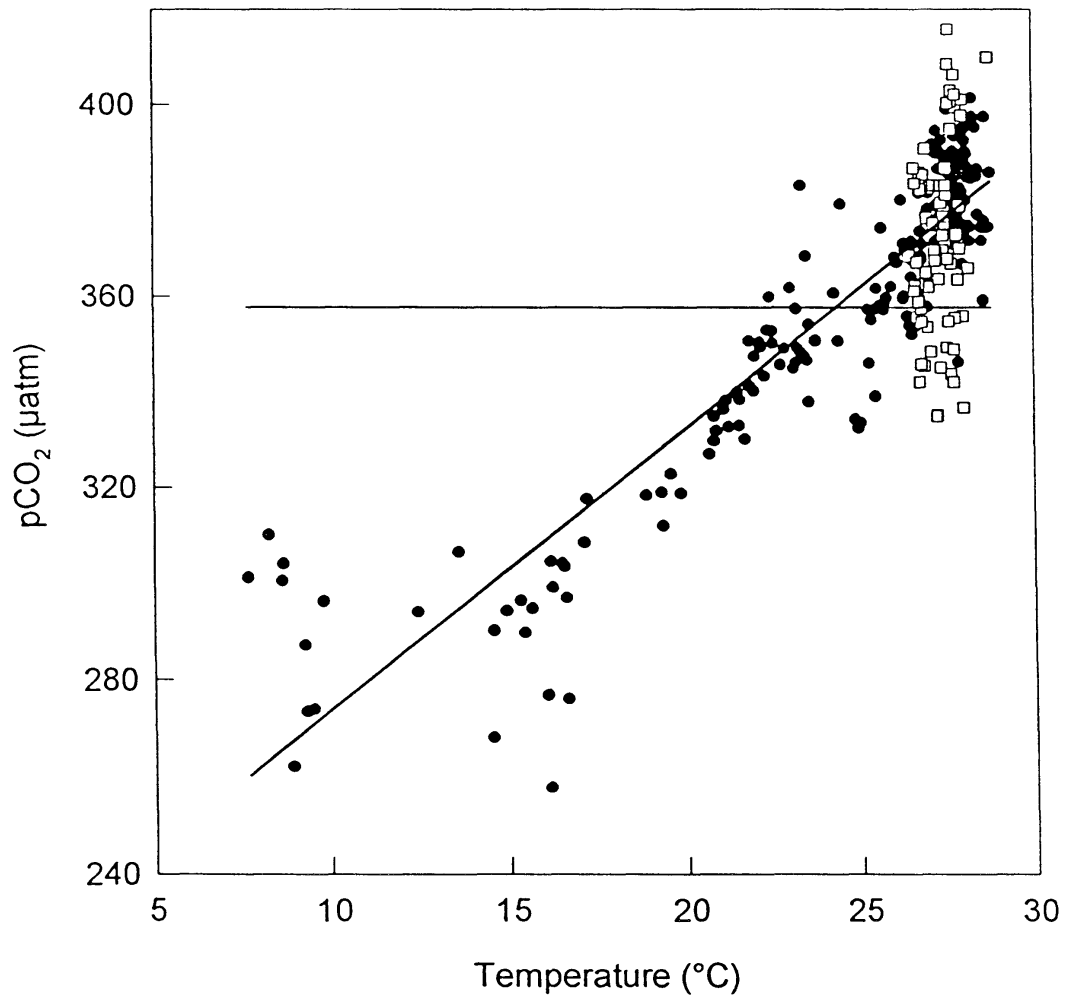
Figure VI-13: Surface p\text{CO}_2 versus temperature. Dots represent CITHER 2 stations, white squares are FOCAL stations.
