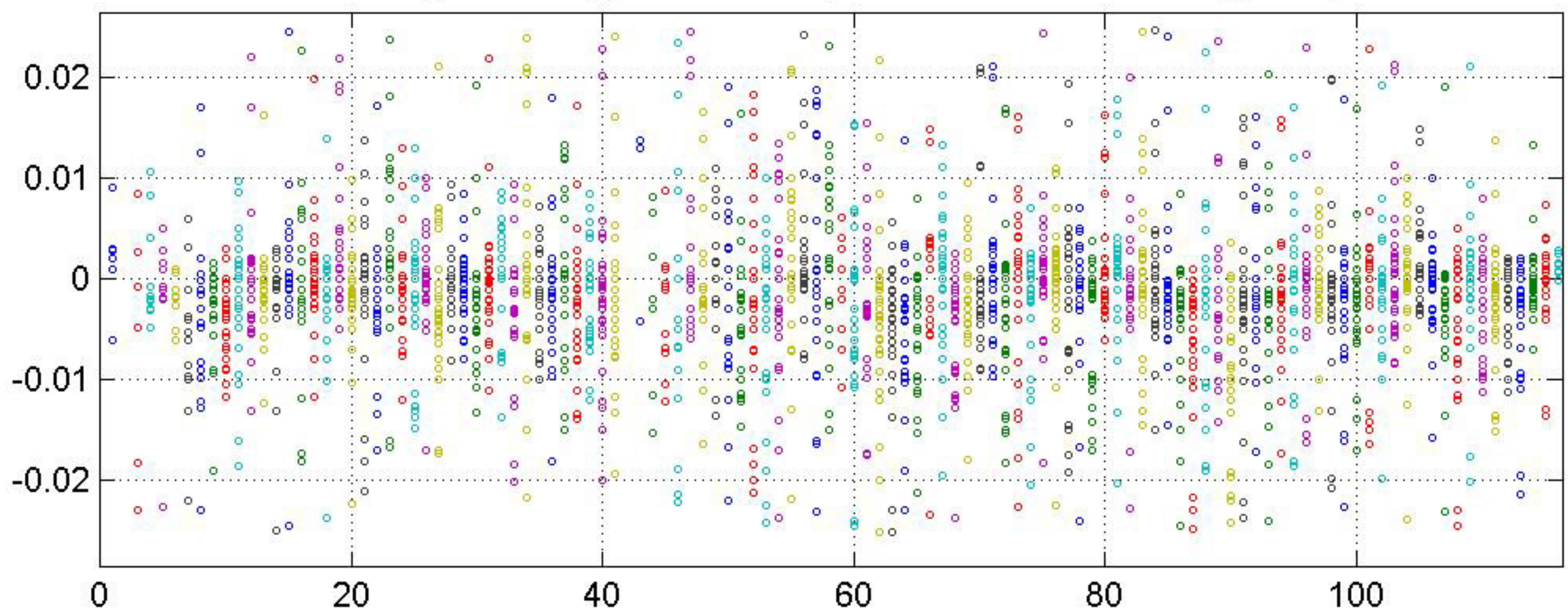
4a A17C: DS (CTD -WS) psu down: only PI Good "2" bottle salts @ all depths
