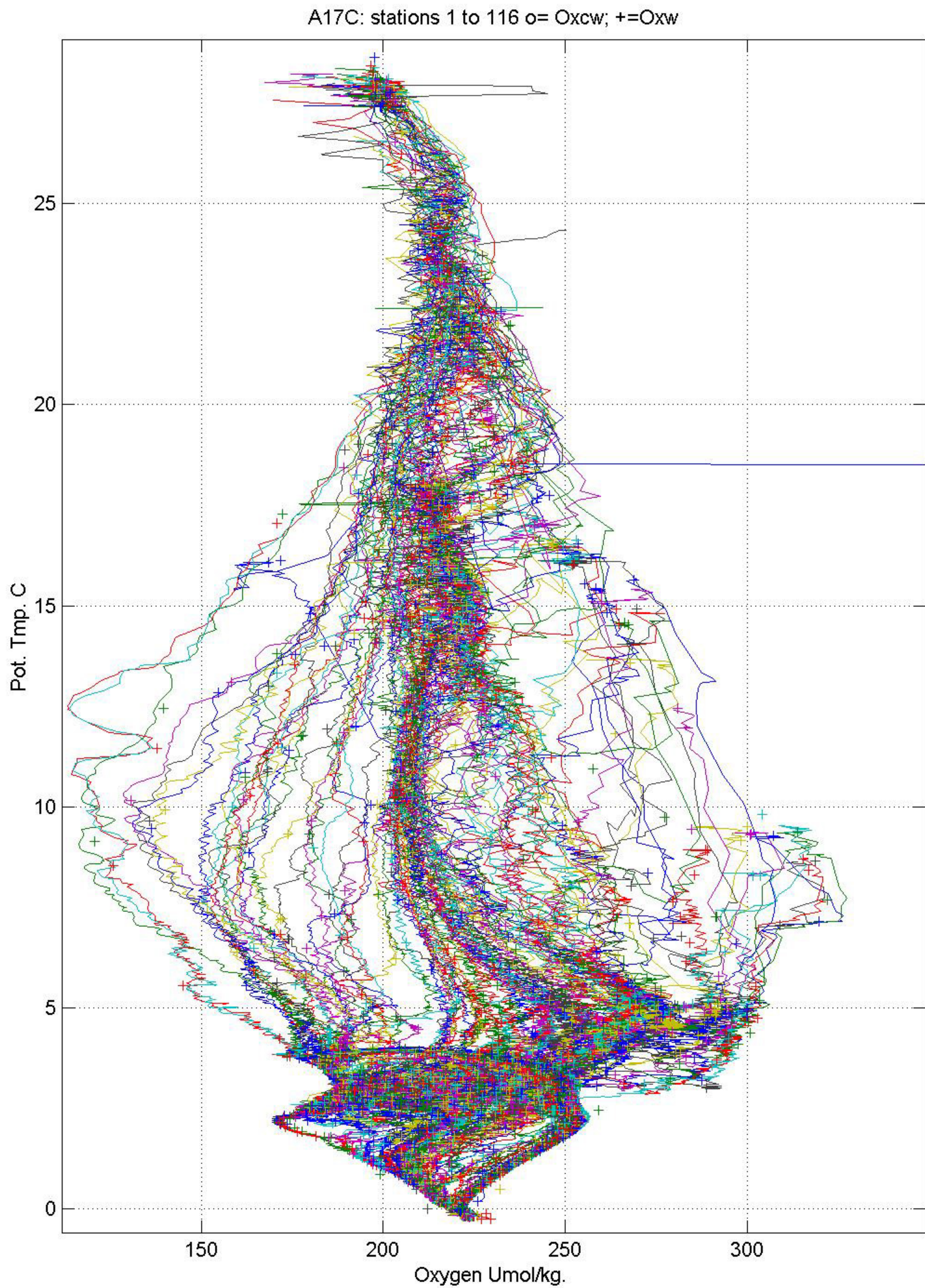
Figure 3a: Overall plot of oxygen versus potential temperature.
