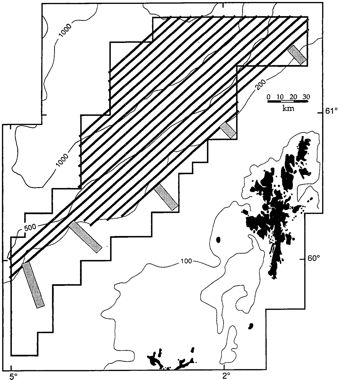
Fig. 2. Proposed survey plan, showing idealised TOBI survey tracks (bold lines) and potential area that could be covered with a 100 kHz sidescan system (shaded rectangles).
