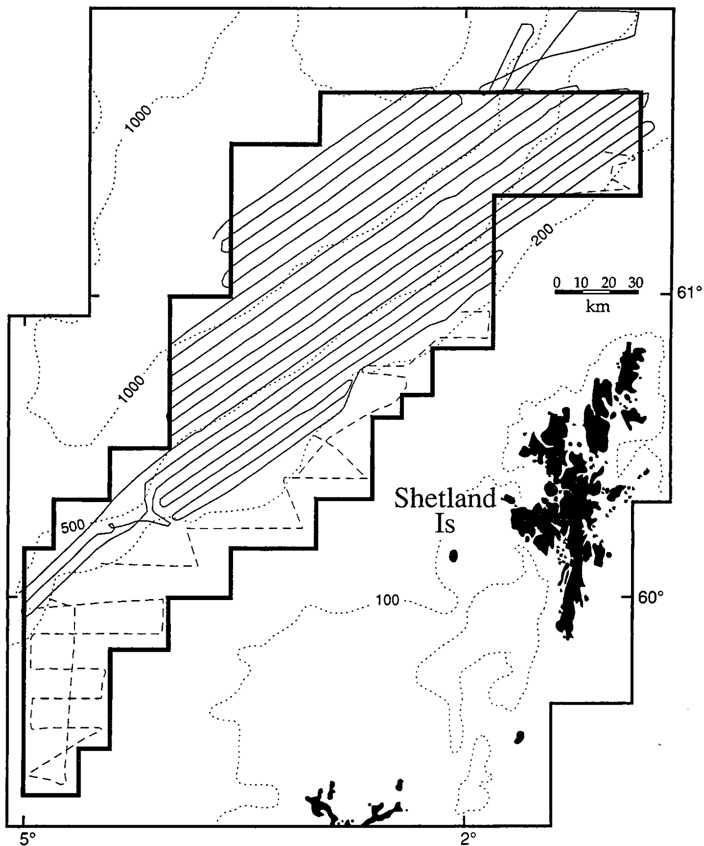
Fig. 5. Survey tracks occupied during the sidescan sonar survey. TOBI survey track is shown by continuous line with line spacing set to give 100% coverage. Dashed line shows 100 kHz sidescan survey track, with a swath width of 750 m. Bold outlined box shows the hydrocarbon licence area.
