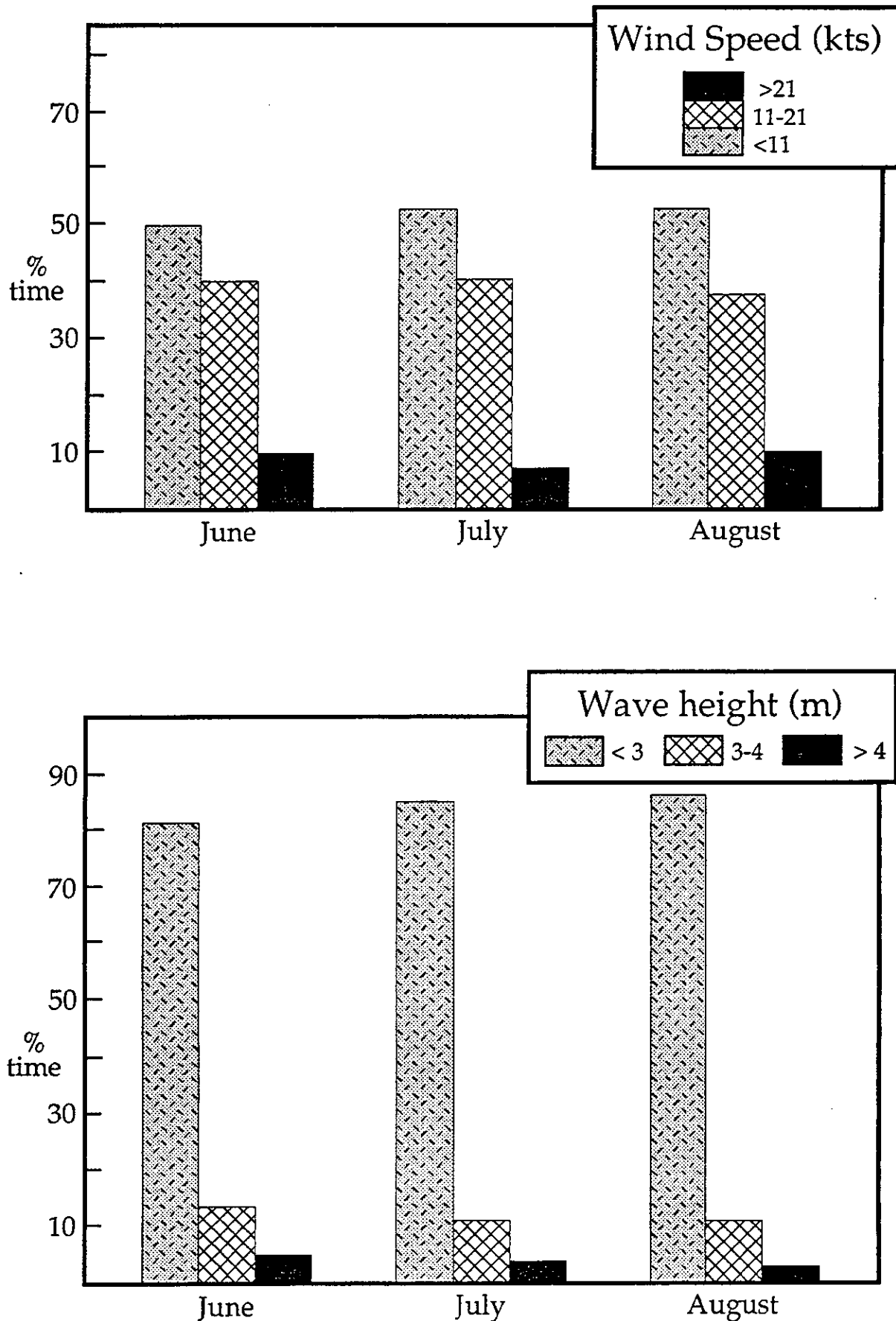
Fig. 3. Predicted weather conditions west of Shetland for the months June to August. Winds in excess of 20-25 kts and seas in excess of 3-4 m are likely to hamper or prevent TOBI operations. In practice just under 5% of survey time was lost due weather related problems (see Table A5).
