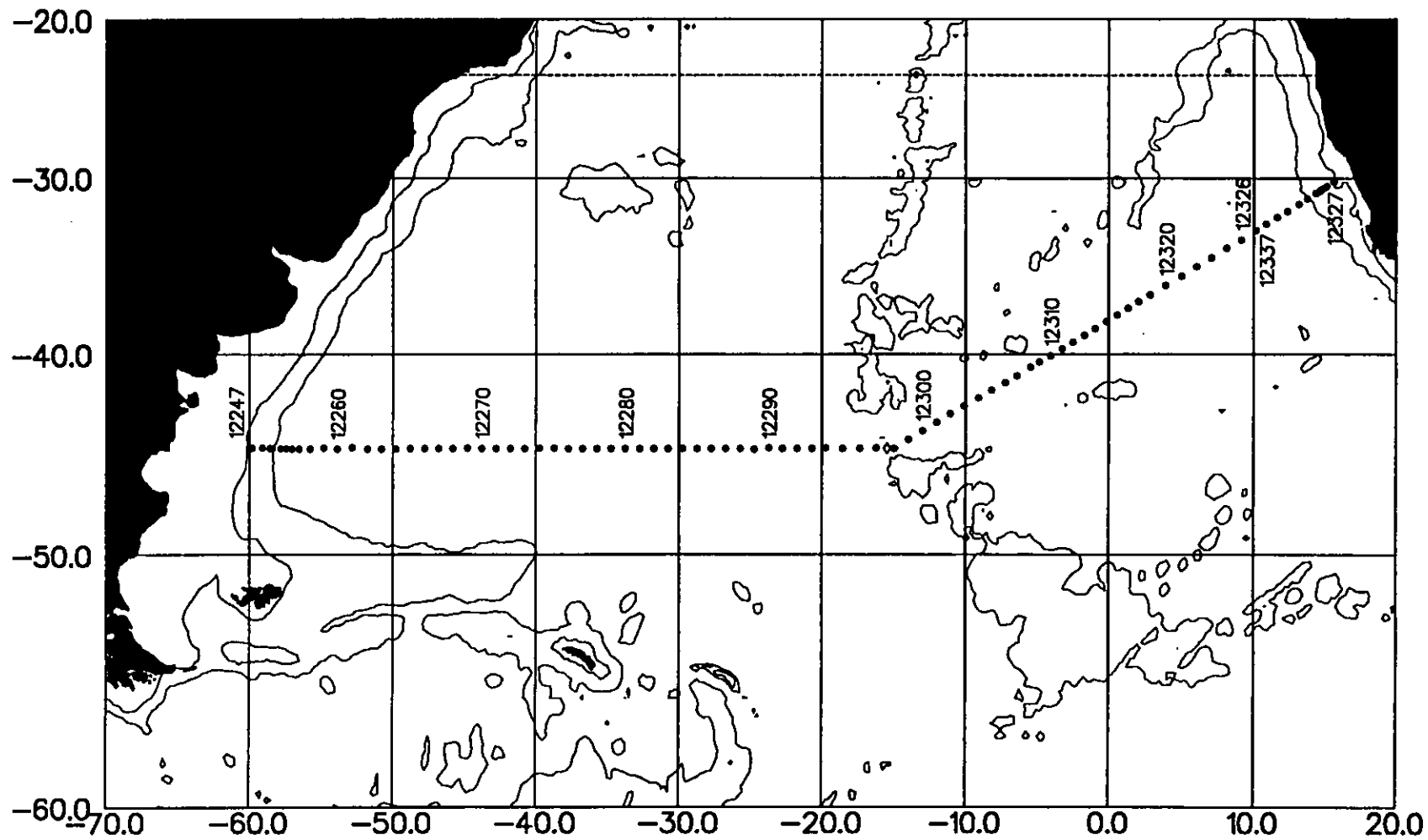
Figure 1. Track Chart: RRS Discovery Cruise 199, 22 Dec 1992 - 01 Feb 1993. Station numbers and isobaths of 200m and 3000m are superimposed.
