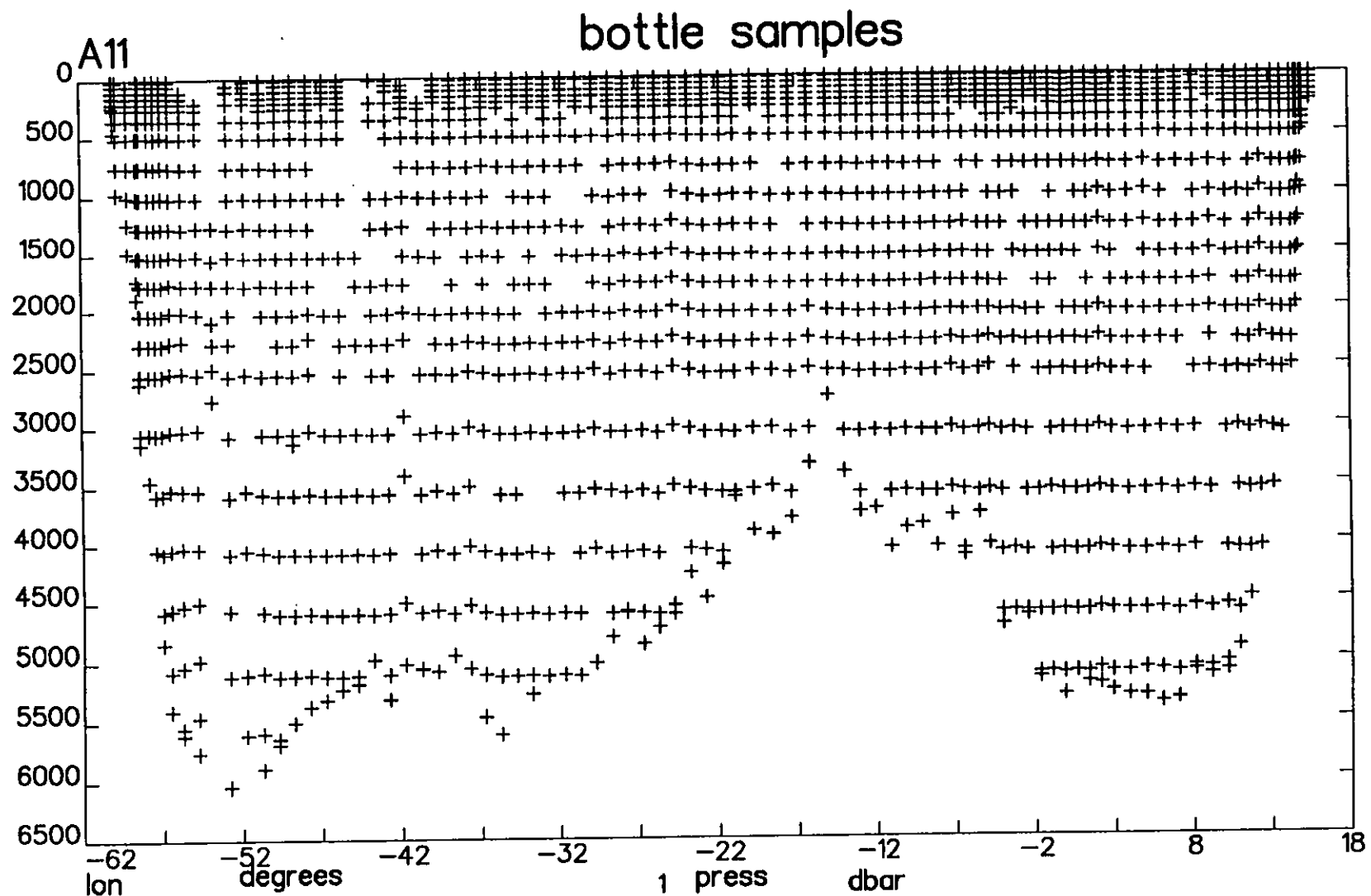
Figure 2. The location of 10 litre water samples collected on cruise A11. Depth is in dbar.
