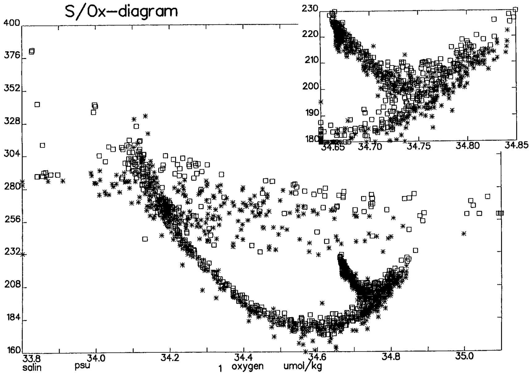
Figure 4. Dissolved oxygen concentration versus salinity for A11 * and SAVE 4 data: both are in the Argentine basin and for the whole water column. The inset, where the deepest levels form the left branch of the Y, shows the small discrepancy between the data sets.
