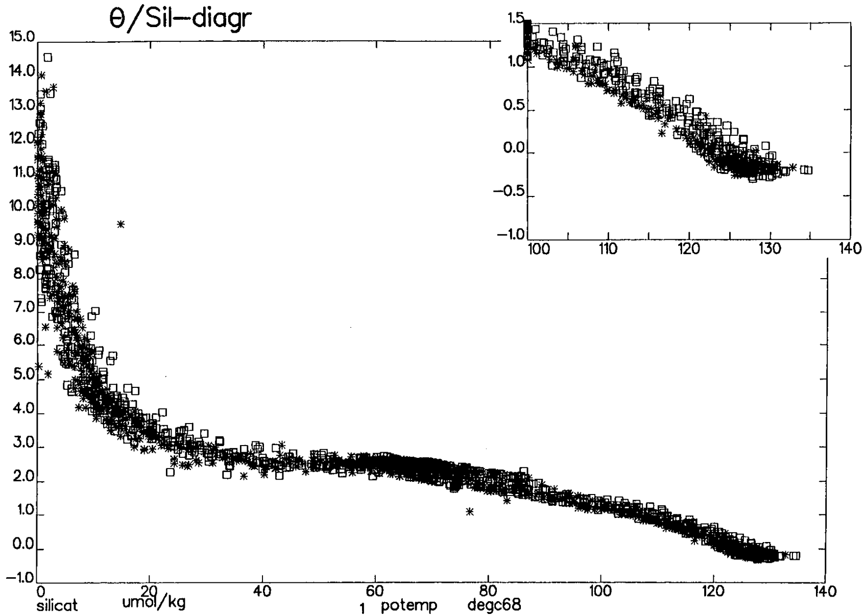
Figure 3. Silicate concentration versus potential temperature for A11 * and SAVE 4 data: both are in the Argentine basin and for the whole water column. The inset, for the deepest levels, shows the small discrepancy between the data sets.
