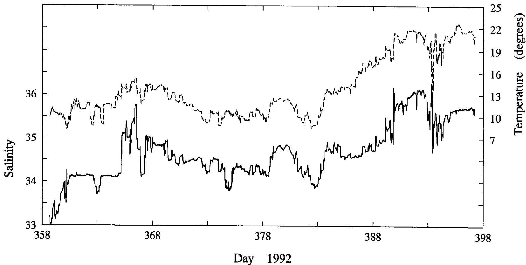
Figure 7. Surface salinity (bold) and temperature (broken) on cruise A11. The cruise begins on the Argentine shelf, passes through the Falkland current (day 363), enters the Brazil current retroflection (day 365), traverses the Subantarctic Zone until somewhere between day 386 and 390 it enters the subtropical gyre. The cruise ends in S. Africa.
