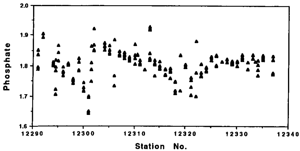
Figure 5. Deep water collected on station 12240 from 2500m was used as quality control for the nutrient measurements: results are shown for the last 50 stations of the cruise.
