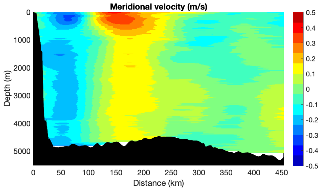
Figure 4a. Meridional velocity section for the Abaco line, from Lowered-ADCP profiles collected at the CTD stations.
