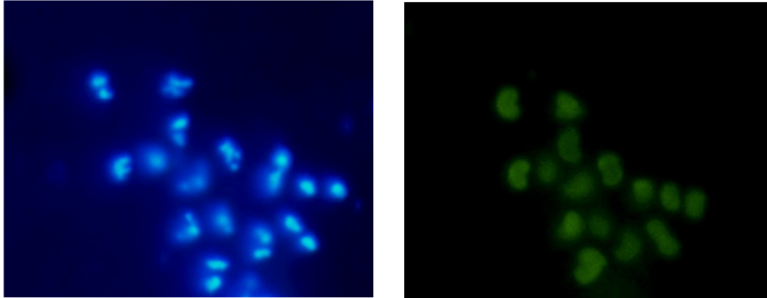
Figure 2. The image on the left shows cellular DNA stained with DAPI. DAPI is excited at 350 nm and emits a blue colour at 450 nm. The blue rod-shaped areas identify individual bacterial cells in a microcolony which had formed in a laminarin incubation by day 3. The image on the right shows the same microscopic field excited at 490 nm. The green colour is light emitting at 520 nm, indicative of fluorescein that the cells have incorporated when degrading the polysaccharide laminarin. In separate FISH experiments we gathered preliminary evidence for affiliation of these cells with Bacteroidetes.
