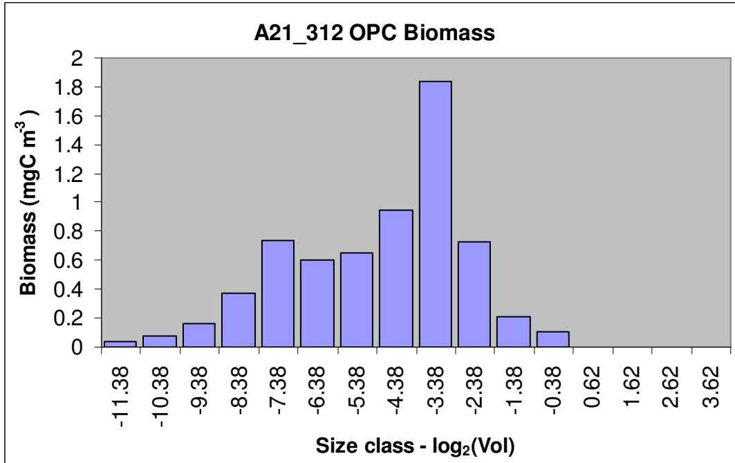
Figure XX.2. OPC Biomass from net cast on AMT21.
