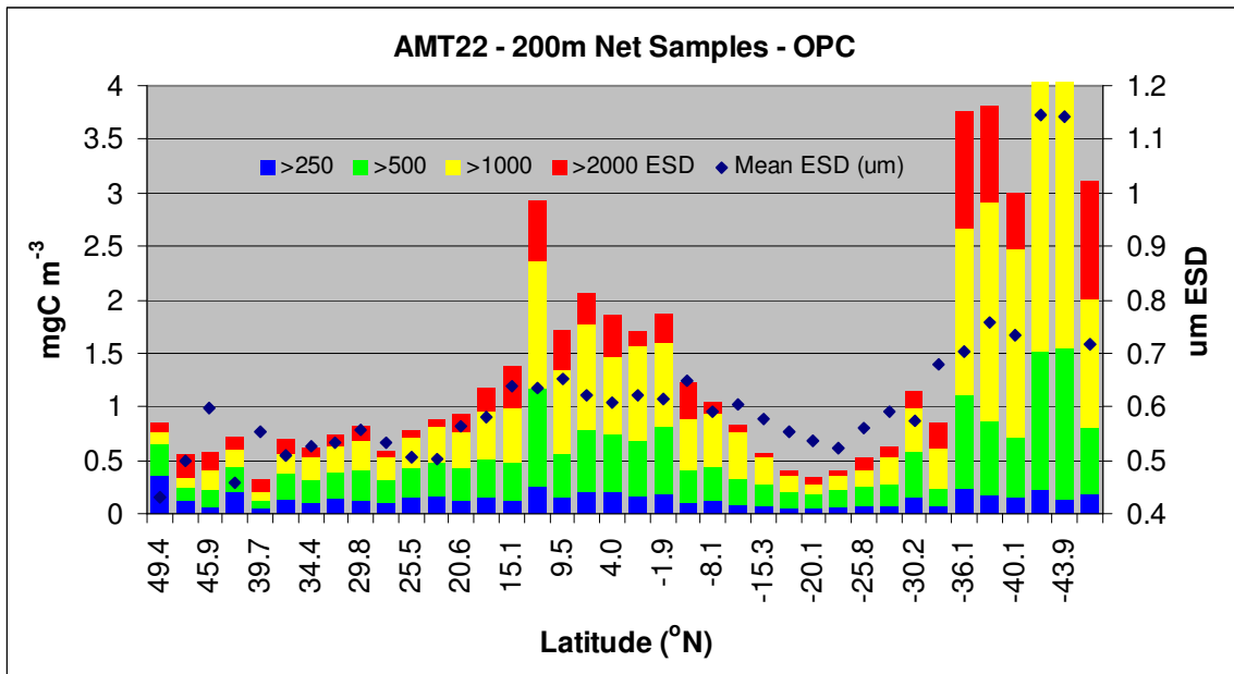
Figure XX.4. OPC size-distributed biomass from all net casts on AMT22.
