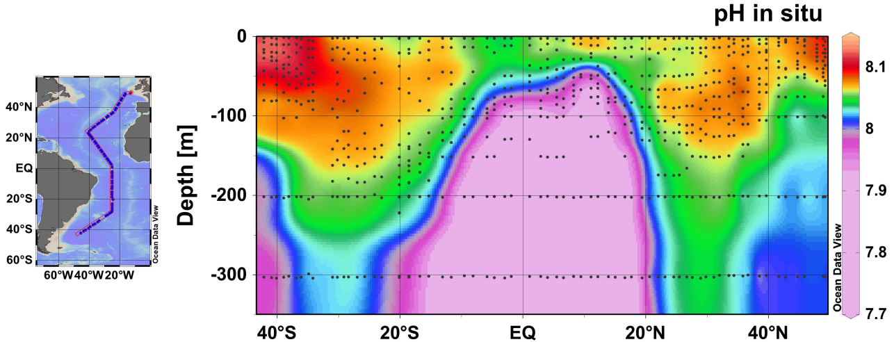
Figure 1: Preliminary pH_T data along-track for AMT 22 (JC079) (stations 2-70). Dots show samples location.
