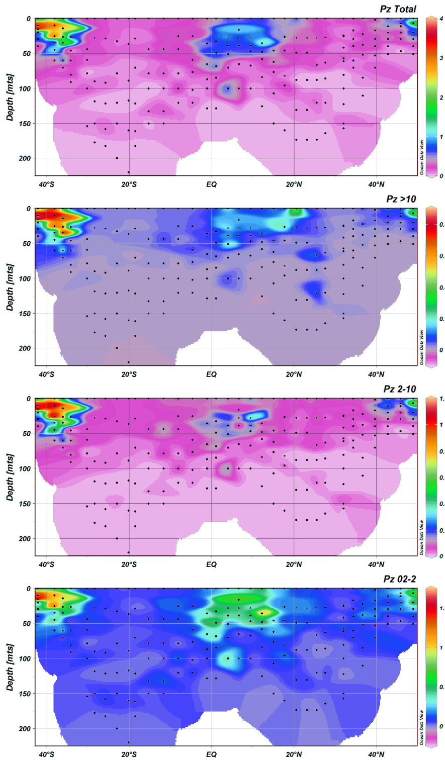
Figure 1. AMT22 Primary production ( \text{mg m}^{-3} \text{d}^{-1} ) in total (Pz Total), micro- (Pz >10), nano- (Pz 2-10), picophytoplankton (Pz 0.2-2) size fractions.
