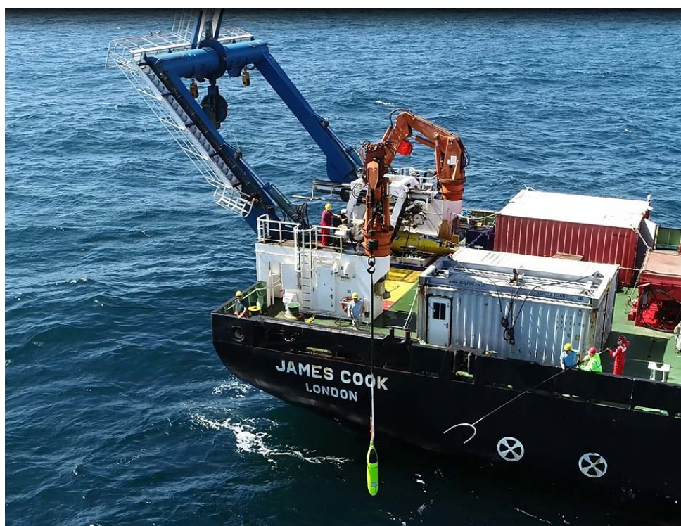
Fig. 5.2 Deepglider deployment
