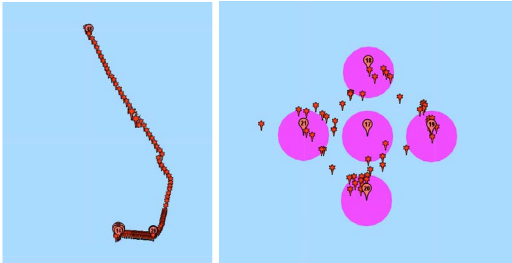
Fig. 4.6 Waveglider holding pattern on 50m radius (using PID line-following)
