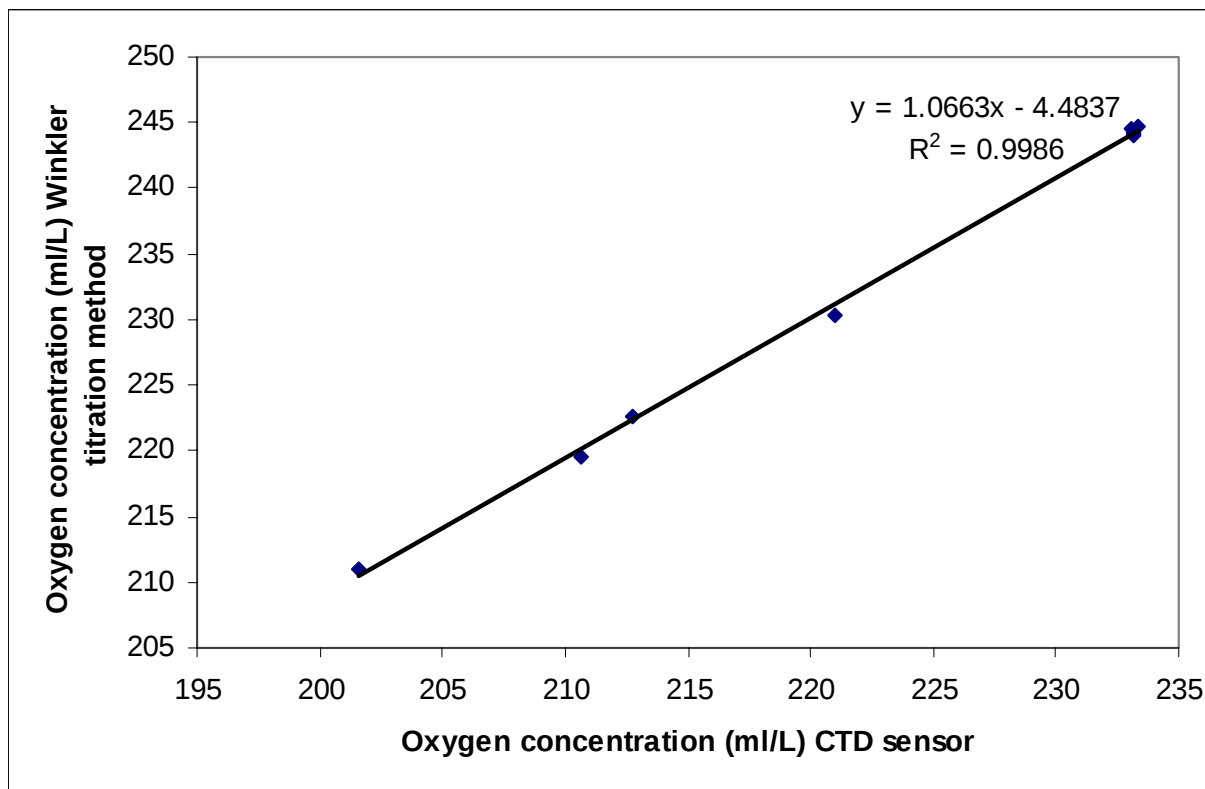
Figure 6 Preliminary Calibration Data for the Stainless Steel CTD Oxygen Sensor. The Complete Calibration Procedure will take Place at BODC
