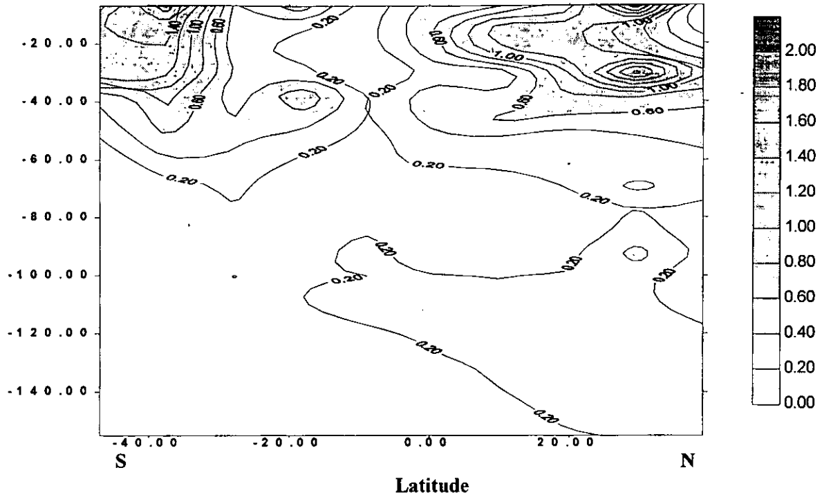
Figure 11 shows a contour plot of total photosynthesis values in a frame of water depth (0-160m) and latitude (50°S to 50°N).
