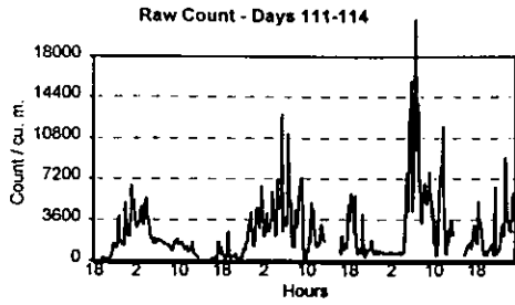
Figures 15a-h. Raw particle counts per cubic metre in underway mode for the whole cruise, showing zooplankton abundance.
