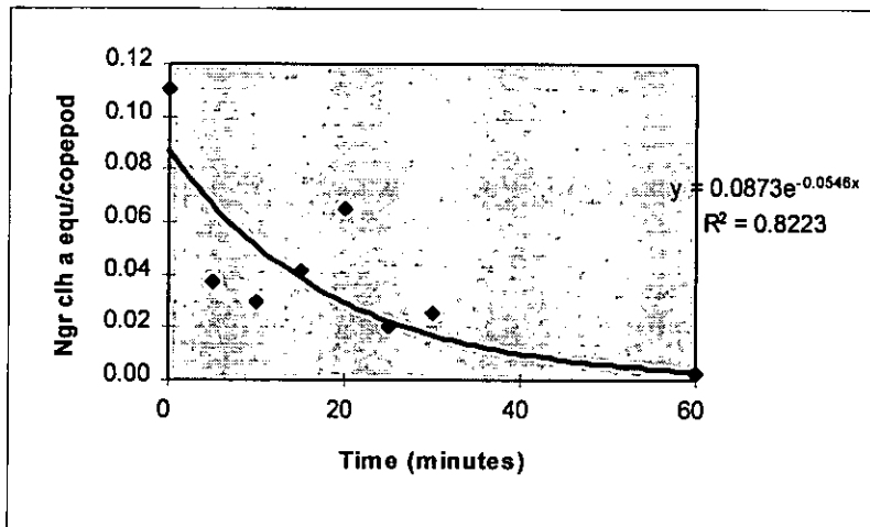
Figure 17 :Example of gut evacuation curve. Size fraction 500-1000μm. Date: 24 -April
