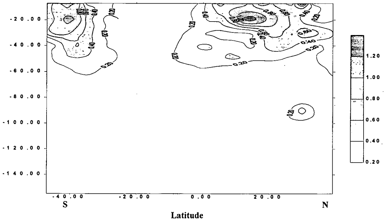
Figure 10 shows a contour plot of picoplankton (0.2-2 \mu m) primary production values in a frame of water depth (0-160m) and latitude (50°S to 50°N).
