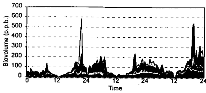
Underway biovolume size fractions Day 132-134
