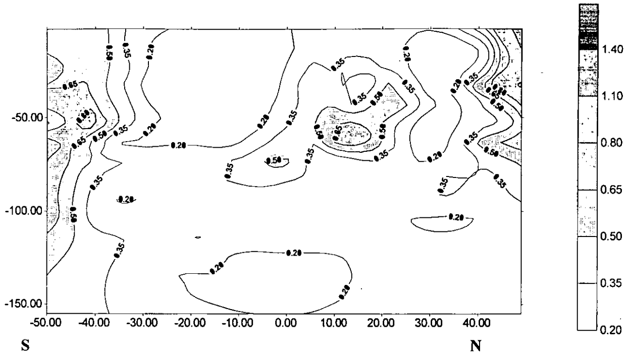
Figure 8 shows a contour plot of total chlorophyll a values in a frame of water depth (0-160m) and latitude (50°S to 50°N).
