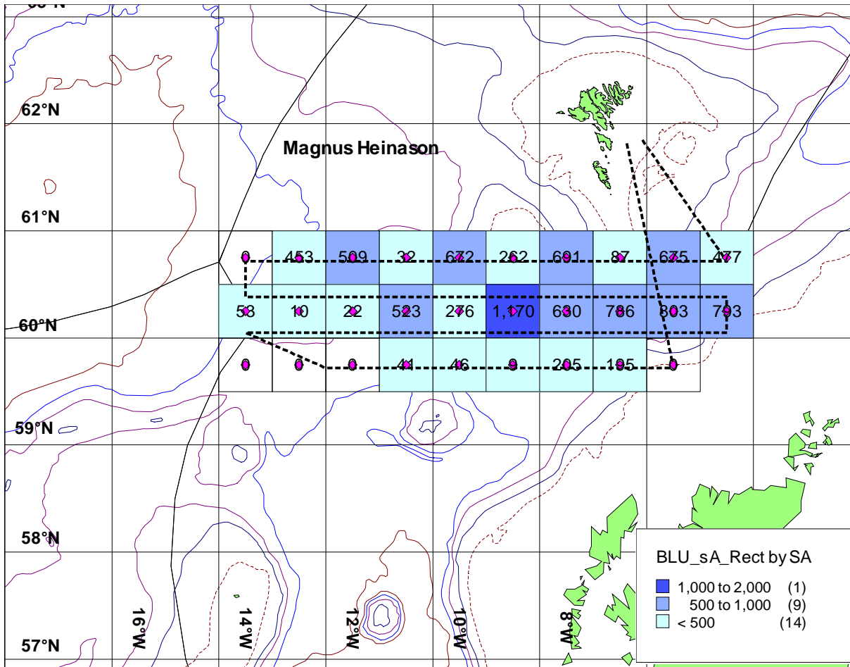
Figure 3. Mean integration values ( s_A , m^2/nm^2 ) of blue whiting per statistical square (1x2 degrees), Magnus Heinason cruise 1410, 27/3-9/4 2014.
