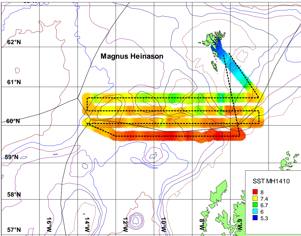
Figure 6. Sea-surface temperature (°C) south of the Faroes, Magnus Heinason cruise 1410, 27/3-9/4 2014.
