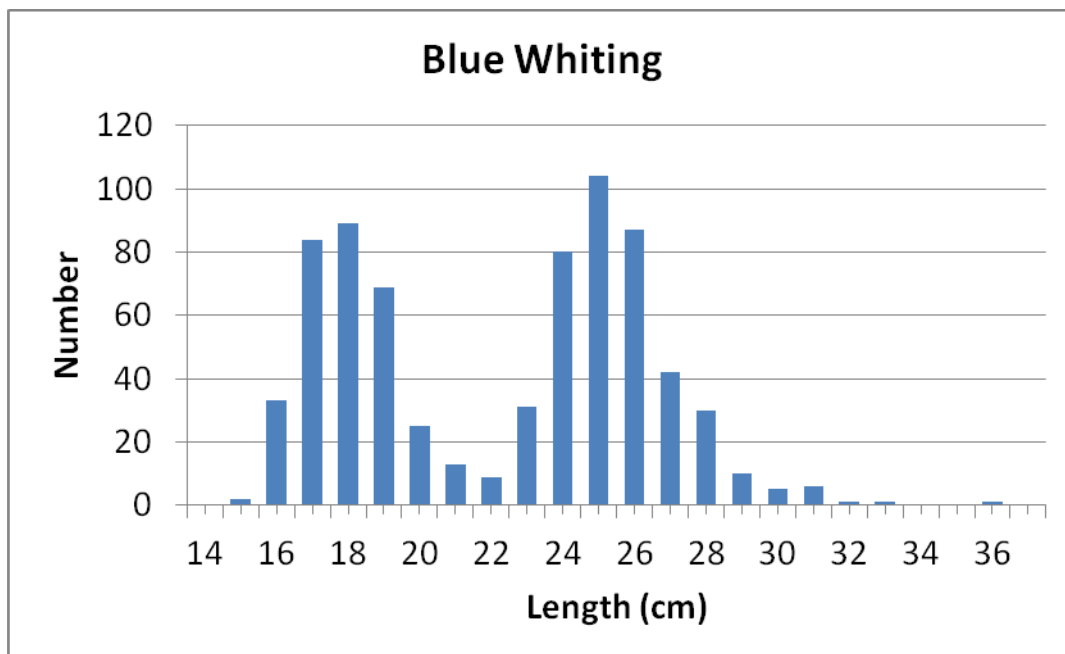
Figure 4. Length distribution of blue whiting south of the Faroes, Magnus Heinason cruise 1410, 27/3-9/4 2014.
