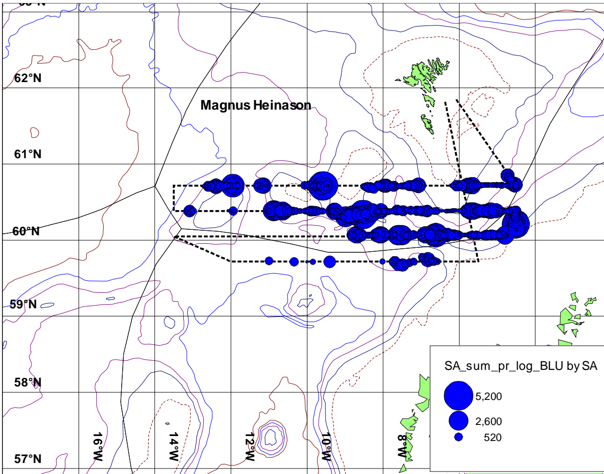
Figure 2. Integration values ( s_A , m^2/nm^2 ) of blue whiting per each nm along the cruise tracks, Magnus Heinason cruise 1410, 27/3-9/4 2014. The size of the circles corresponds to amount of fish.
