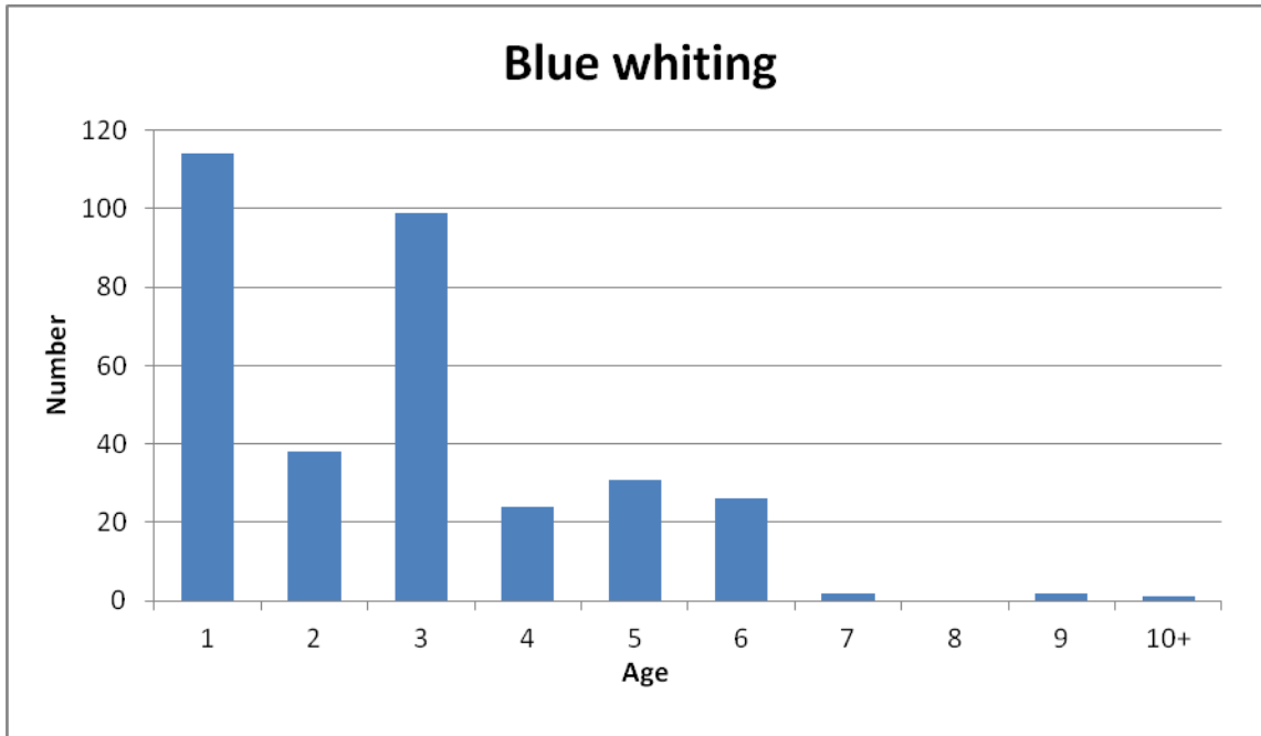
Figure 5. Age distribution of blue whiting south of the Faroes, Magnus Heinason cruise 1410, 27/3-9/4 2014.
