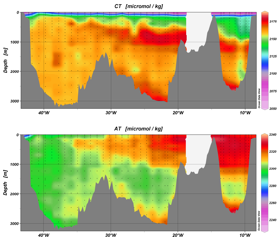
Figure 8-. Distribution of (a) dissolved inorganic carbon (CT) and (b) total or titration alkalinity (AT) along the former WOCE A1 section.
