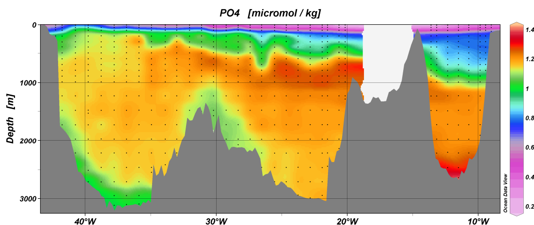
Figure 6. Dissolved phosphate
