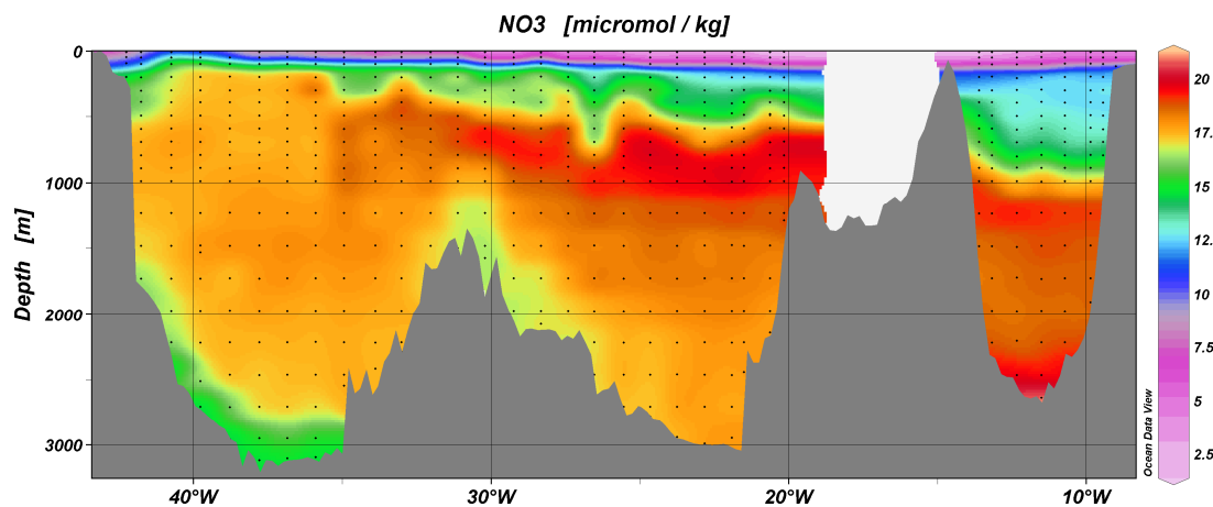
Figure 7. Dissolved nitrate
