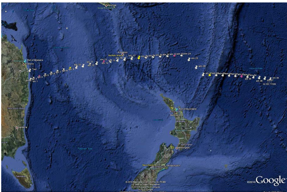
Figure 4. Station locations along the Australian leg of the GEOTRACES GP13 cruise track (voyage ss2011_v02) overlain on Google Earth bathymetry of the study region. Normal stations (1o longitude spacing) are shown in white, super stations (every 5o) in yellow and mega stations (every 10o) in pink. Start (Brisbane, 13 May 2011) and finish (Auckland, 05 June 2011) ports are shown as blue markers. Stations 9 and 25 were cancelled due to bad weather.
