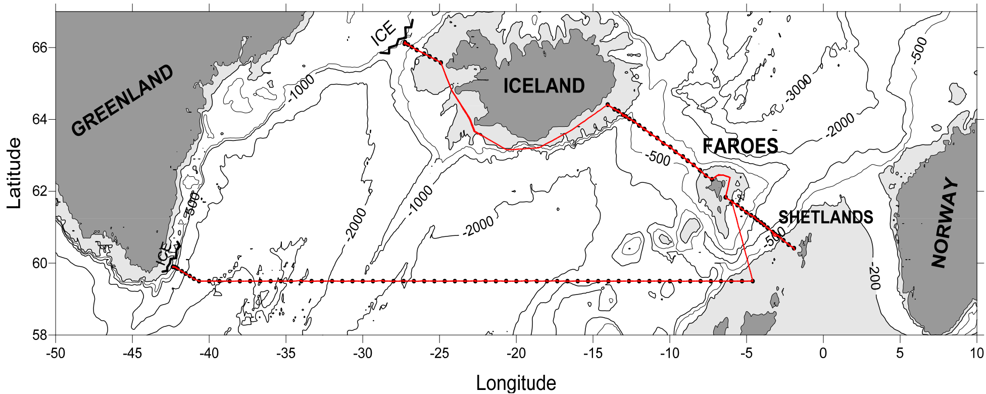
Fig. 1 Station locations (black circles) and ship track (in red). The shelf area with depth less than 200 m is shaded.
