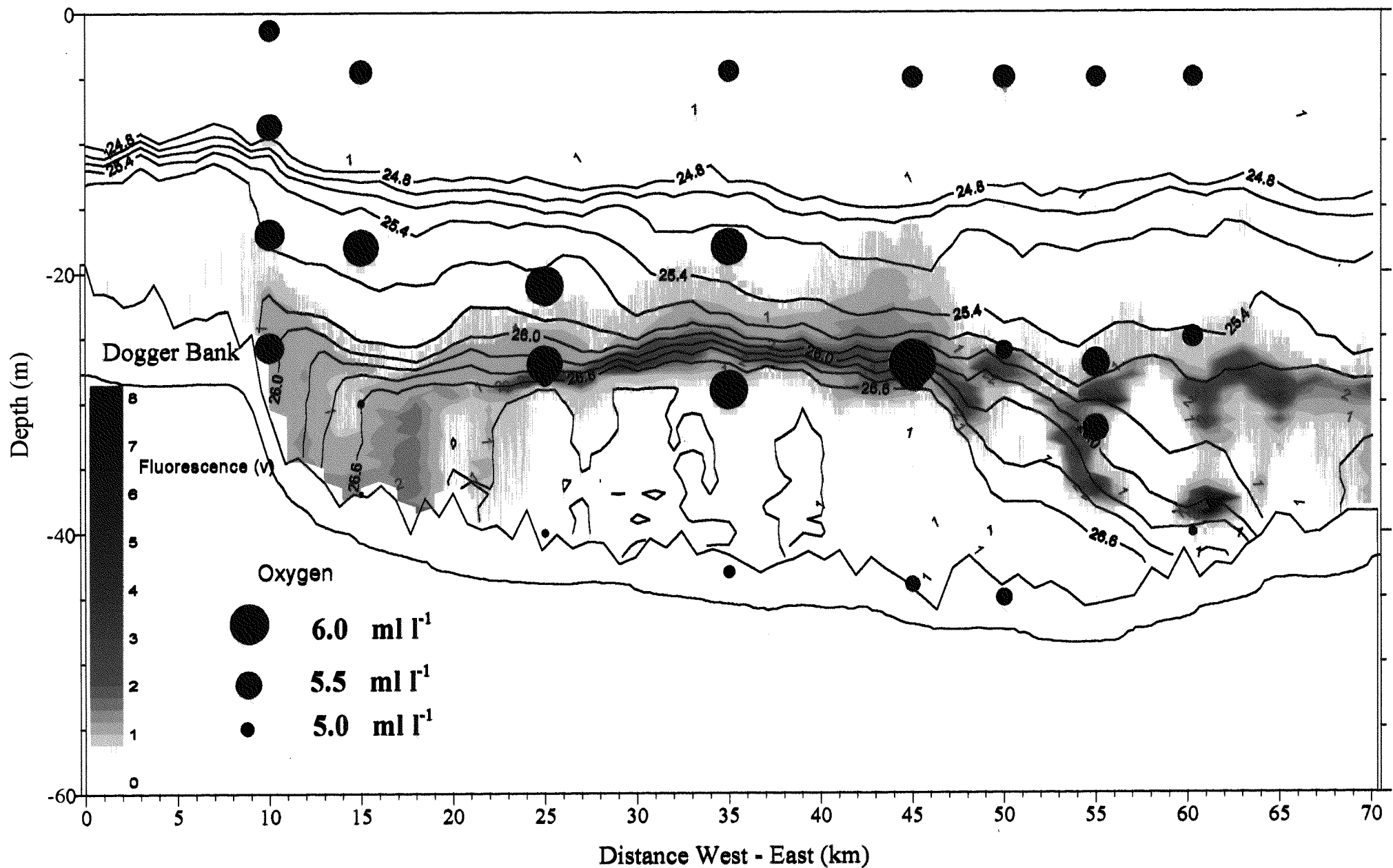
Figure 4 Density ( \sigma_t kg m -3 ), fluorescence (volts) and Oxygen (ml l -1 ) from CTD's along Section 10
