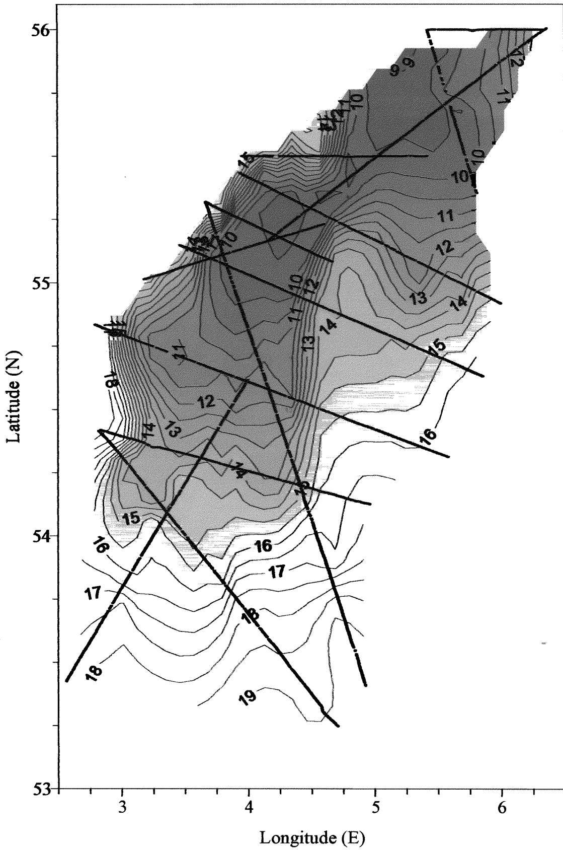
Figure 2 Bottom Temperature 13 - 24 August
