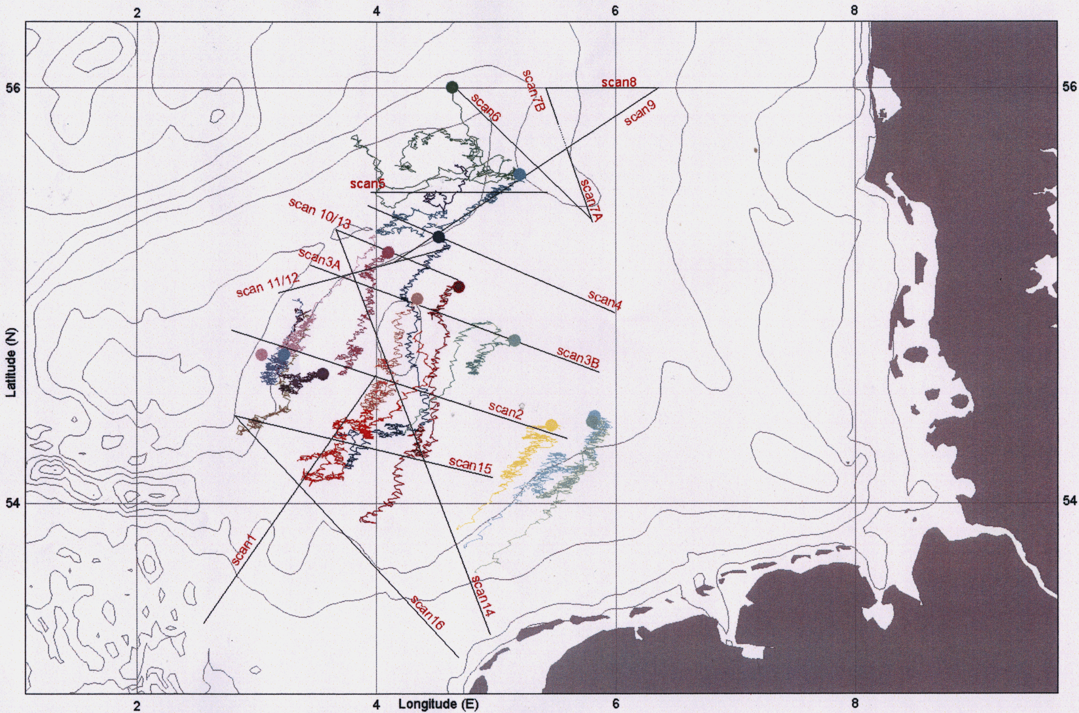
Figure 3: August and July drifter tracks and recovery positions with scanfish survey lines
