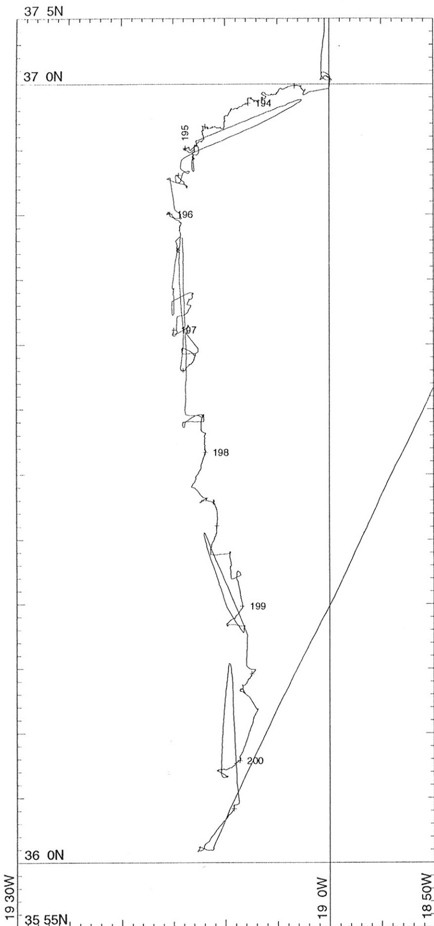
Fig. 7. Plan of cruise track, RRS Discovery Cruise 221, in vicinity of Argos buoy, Leg 2 12 July-18 July 1996.
