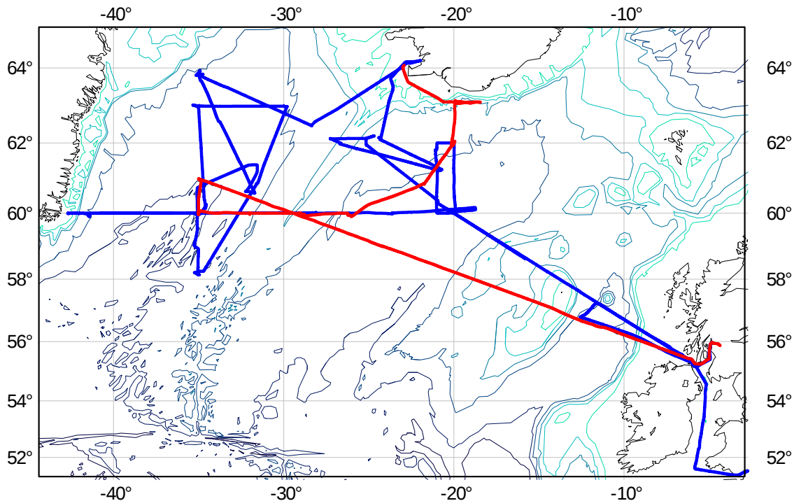
Fig. 1: Cruise tracks of D350 (red) and D354 (blue); contour lines show 200, 500, 1000, 2000, 3000 and 4000 m bottom depth
