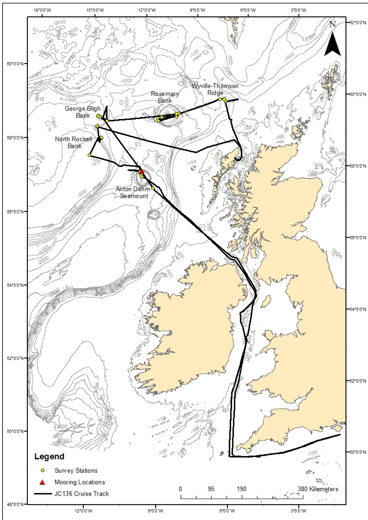
Working area and track chart of RRS James Cook, Cruise JC136. Bathymetry from GEBCO.
