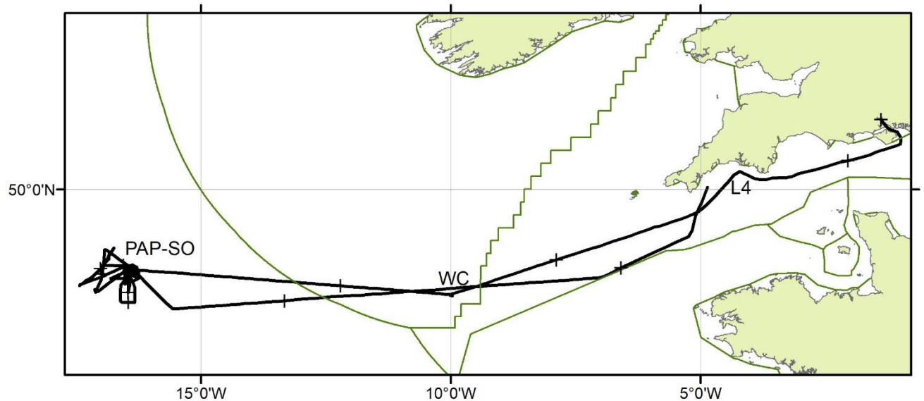
Cruise track until 5-21st May 2023. PAP-SO: Porcupine Abyssal Plain Sustained Observatory, WC: Whittard Canyon, L4: Part of Western Channel Observatory, +: midnight positions.
