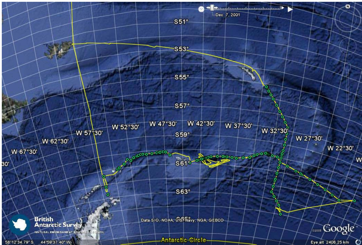
Ship track of JR235/236/239 when active in field area (originally passage from Montevideo to Stanley, FI, not fully shown). Green dots denote locations of CTD/tracer/CO2 stations.
