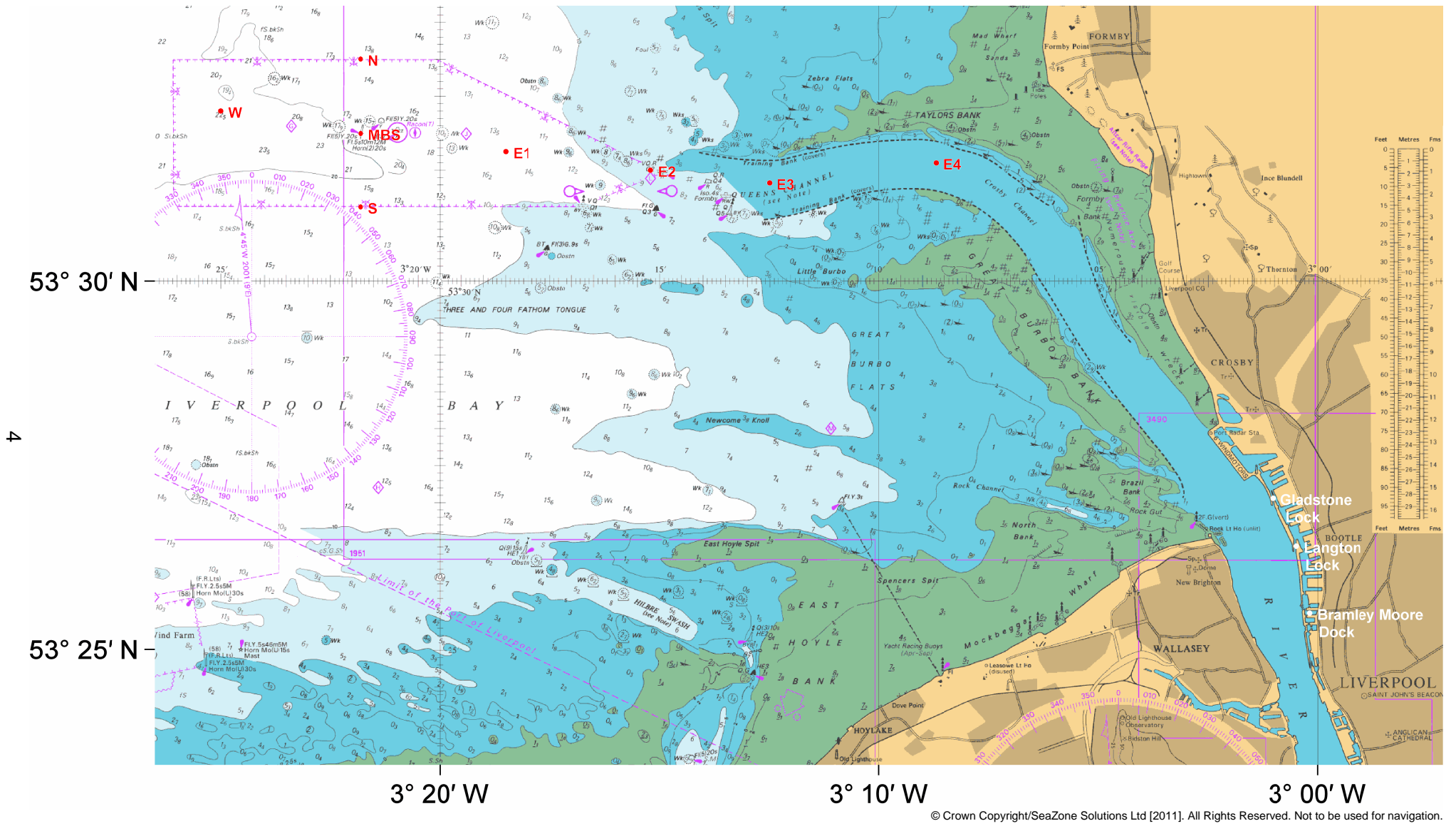
Figure 1. Liverpool Bay Observatory cruise 80, CTD stations, 8–10th November 2011
