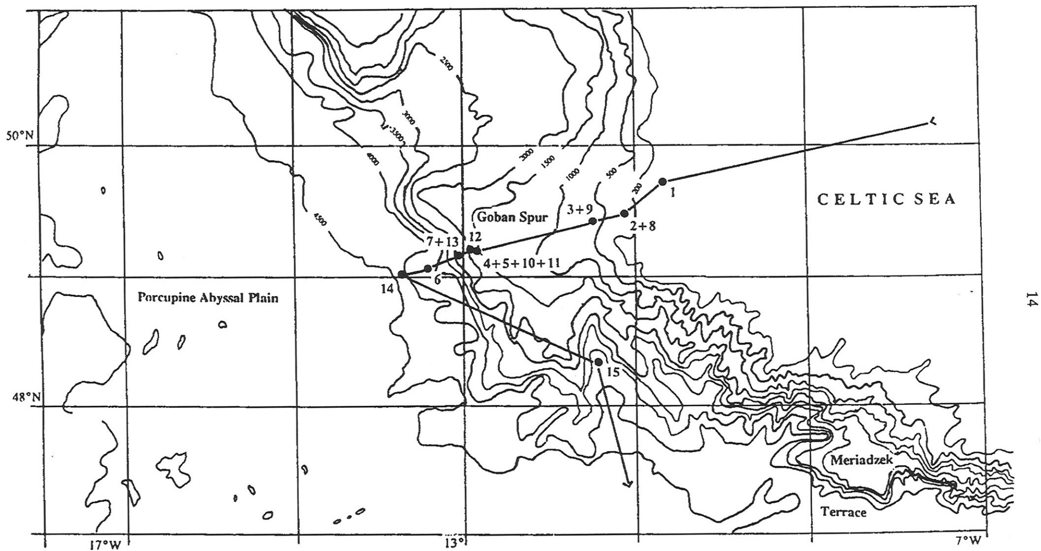
Fig. 3: Cruise track and sampling stations of M 27/1. Due to adverse weather conditions several stations had to be occupied several times.
