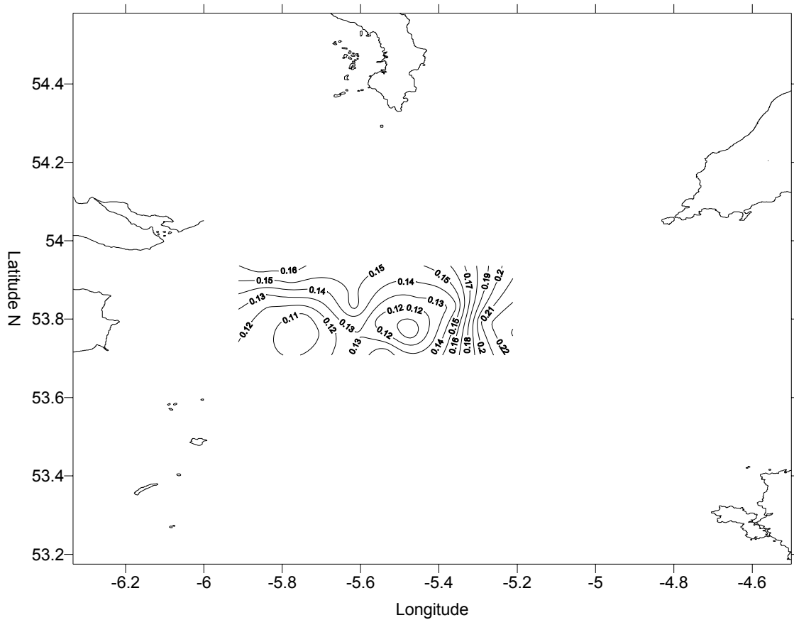
Figure 6. Map of K(555) m -1 in the Western Irish Sea, measured during RV Prince Madog Cruise, 2-6 April 2002
