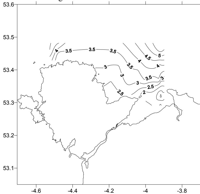
Figure 7. Contour plot of Secchi Depth (m) around Conwy Bay generated using data gathered by R.V. Prince Madog cruise from 26 th November 2001 – 30 th November 2001
