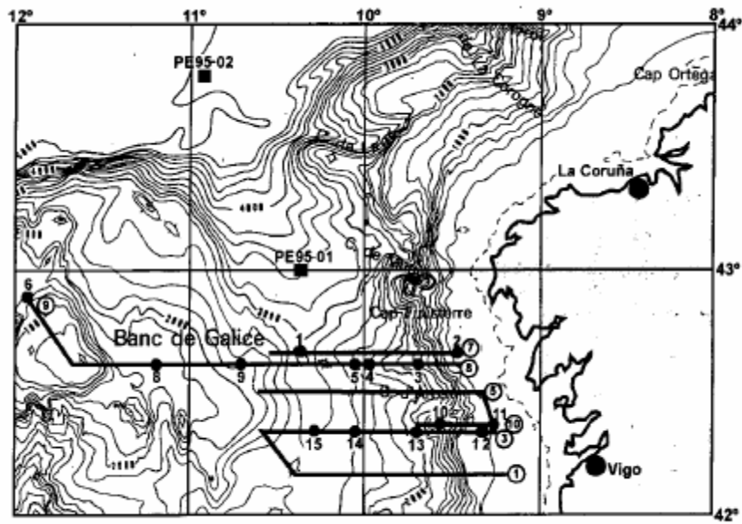
Fig. 2.1. Map of cruise tracks and sampling stations.
