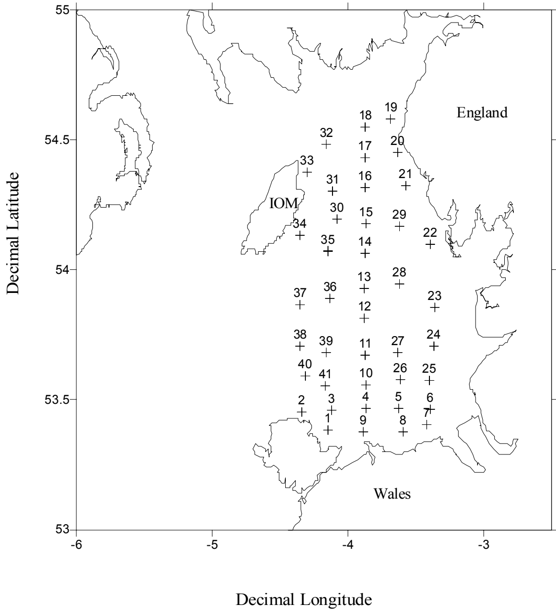
CEFAS charter programme, cruise Prince Madog 5 / 03: station track showing mid-point positions of 41 plankton tows (numbered consecutively) in the eastern Irish Sea, 28 - 30 April 2003.
