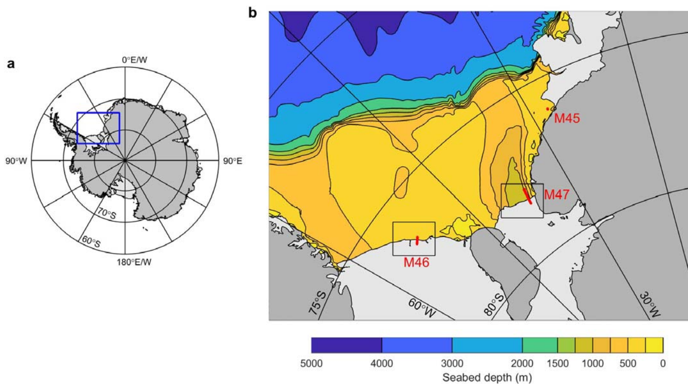
(a) Map of Antarctica showing ice sheet (darker shading), ice shelves (lighter shading) and study area (outlined in blue). (b) Enlargement of study area showing bathymetry and routes of ALR missions M45, M46 and M47.
