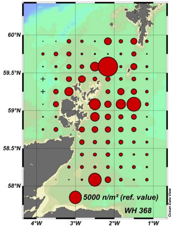
Figure 1: Cruise track (by haul number, left panel) and corresponding abundance of herring larvae in the Orkney/Shetland area ( n/m^2 , right panel). The symbol size corresponding to 5000 larvae per square metre is indicated in the figure.
