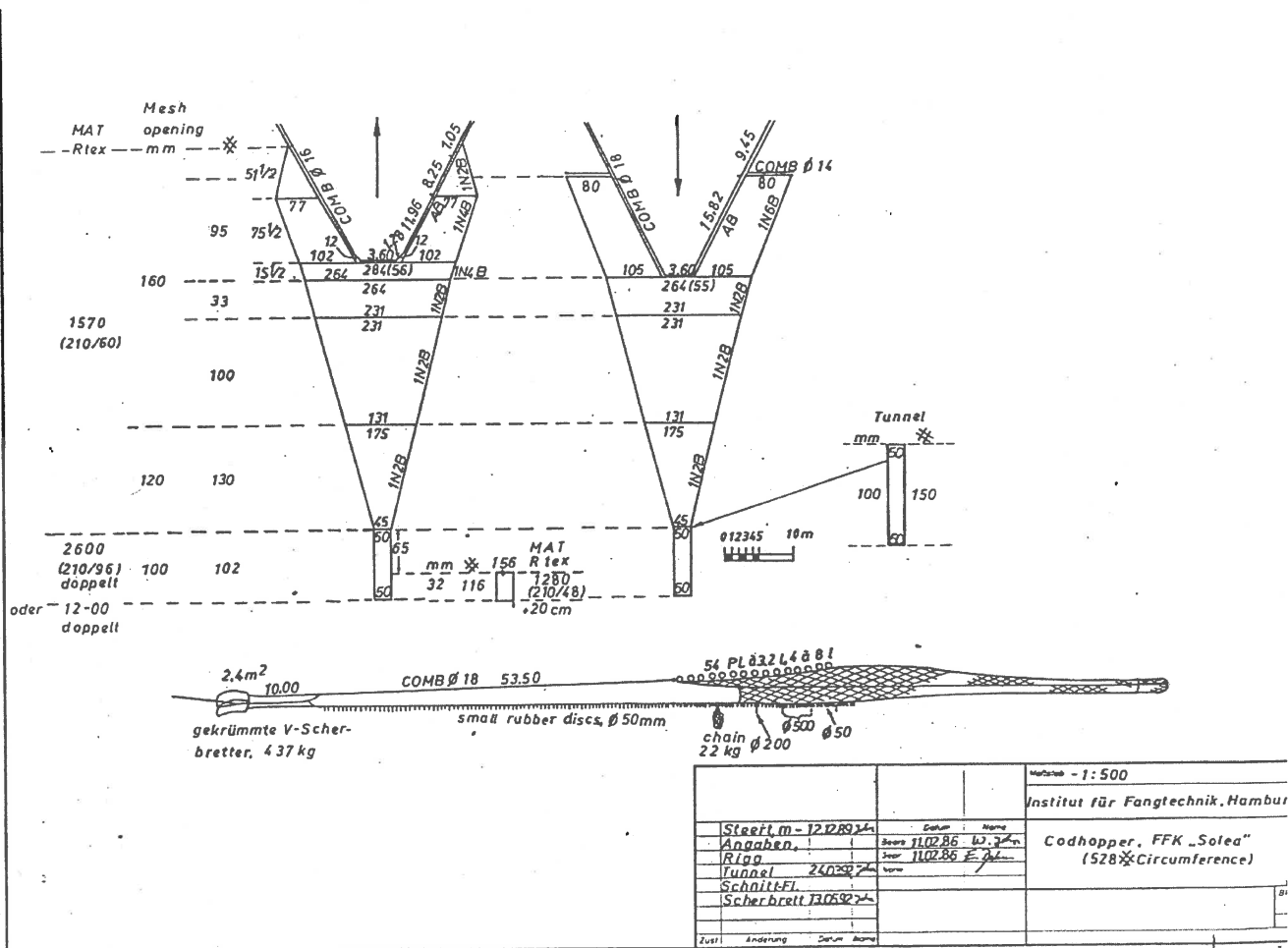
Specification of the gear (Codhopper)
