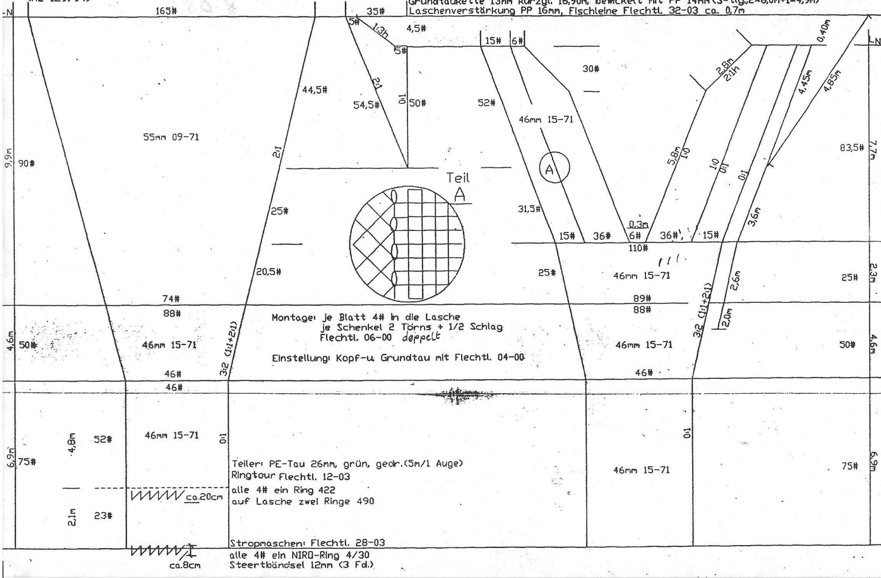
Specification of beam trawl
