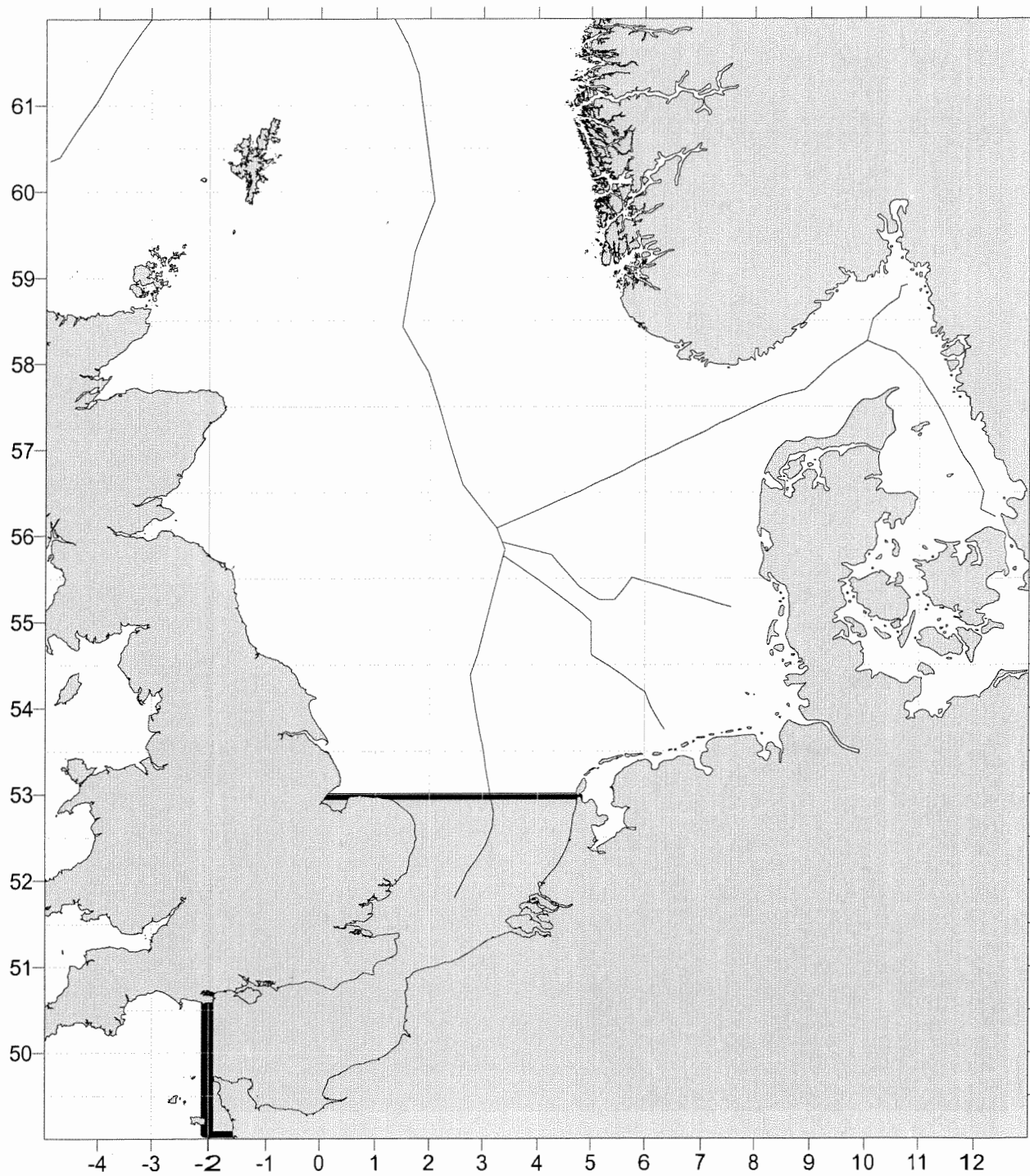
Comparative fishing and horse mackerel egg survey, Tridens, 15 - 19 May 2006
