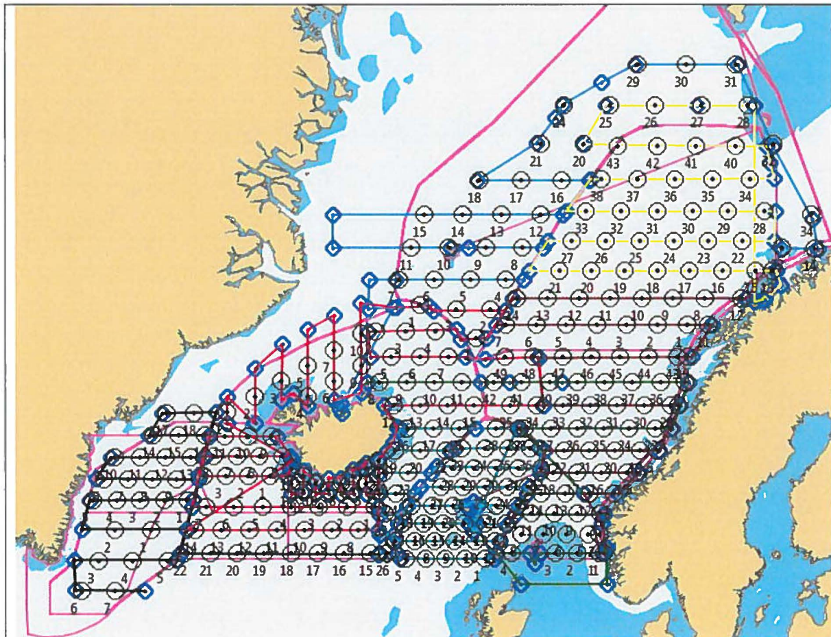
Figure 1. Preliminary surface stations (open black circles) and transects (black, blue and yellow = Norway with 2 vessels, turquoise = Faroe Islands, red = Iceland, black = Greenland) for IESSNS in July-August 2018.
